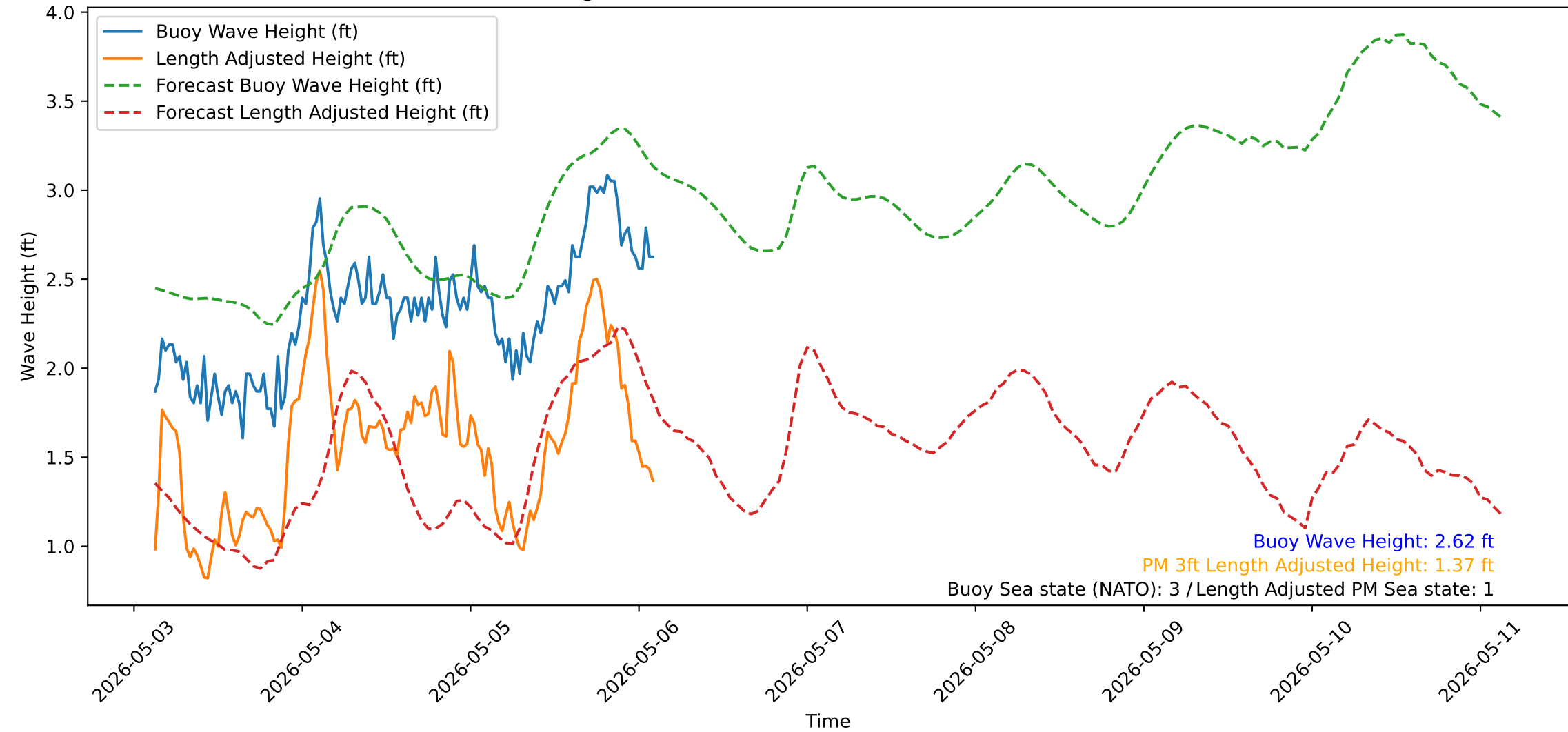
Wave Heights over Time for Red Beach at 2026-05-06 02:40:50
