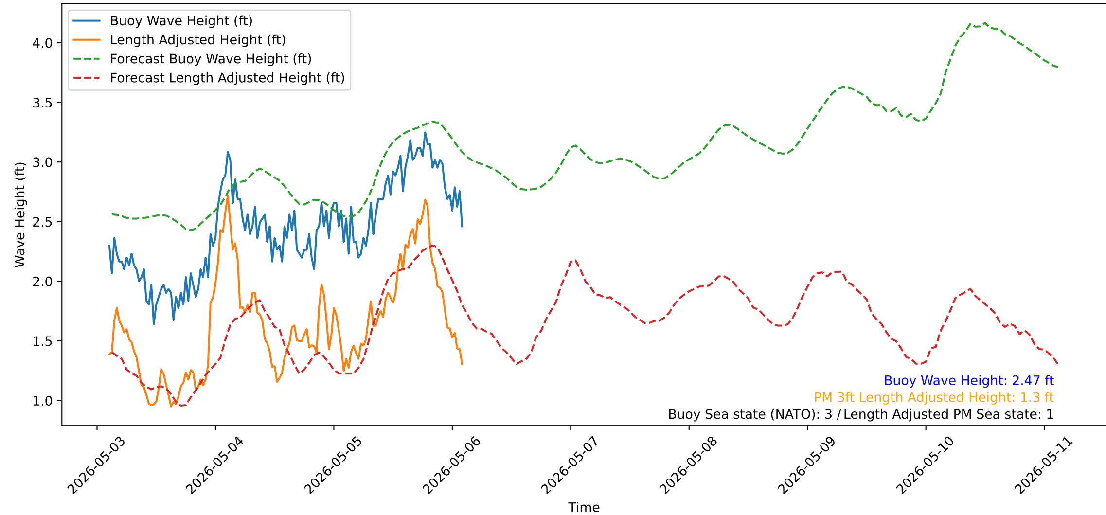
Wave Heights over Time for Oceanside Harbor at 2026-05-06 02:40:31
