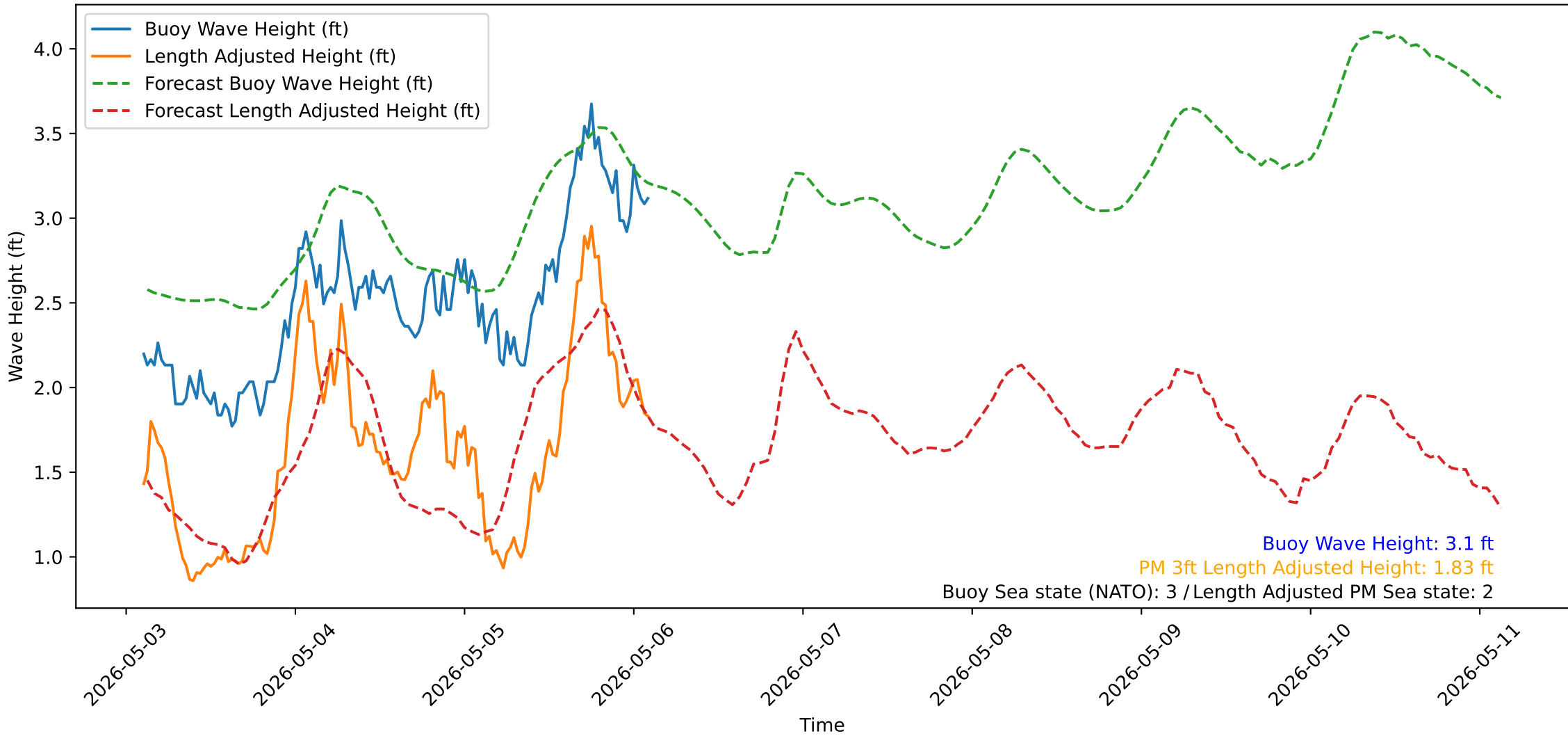
Wave Heights over Time for Green Beach at 2026-05-06 02:41:12
