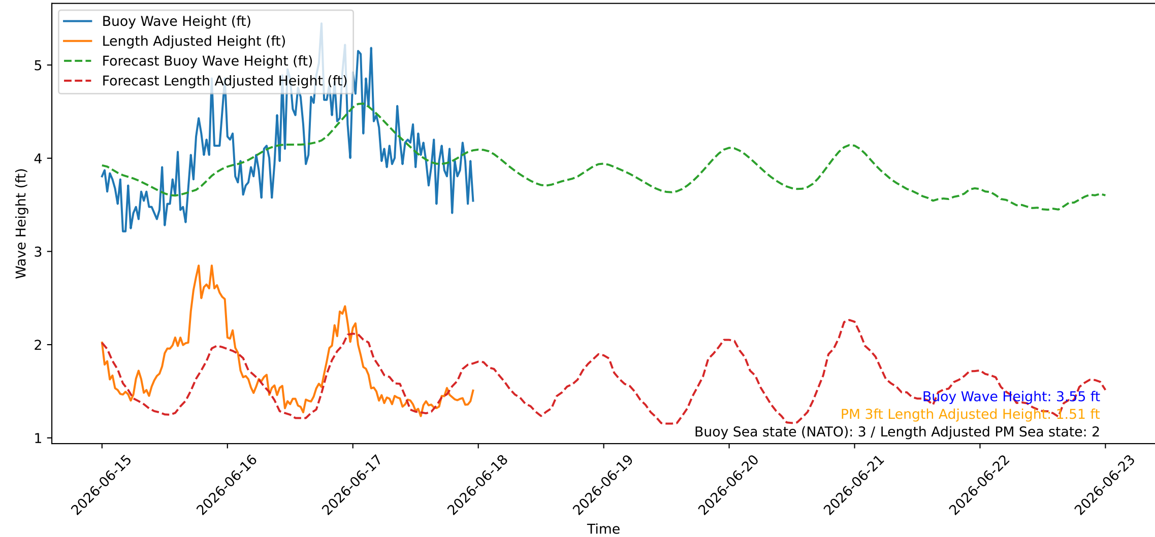
Wave Heights over Time for Oceanside Harbor at 2026-06-17 23:50:26
