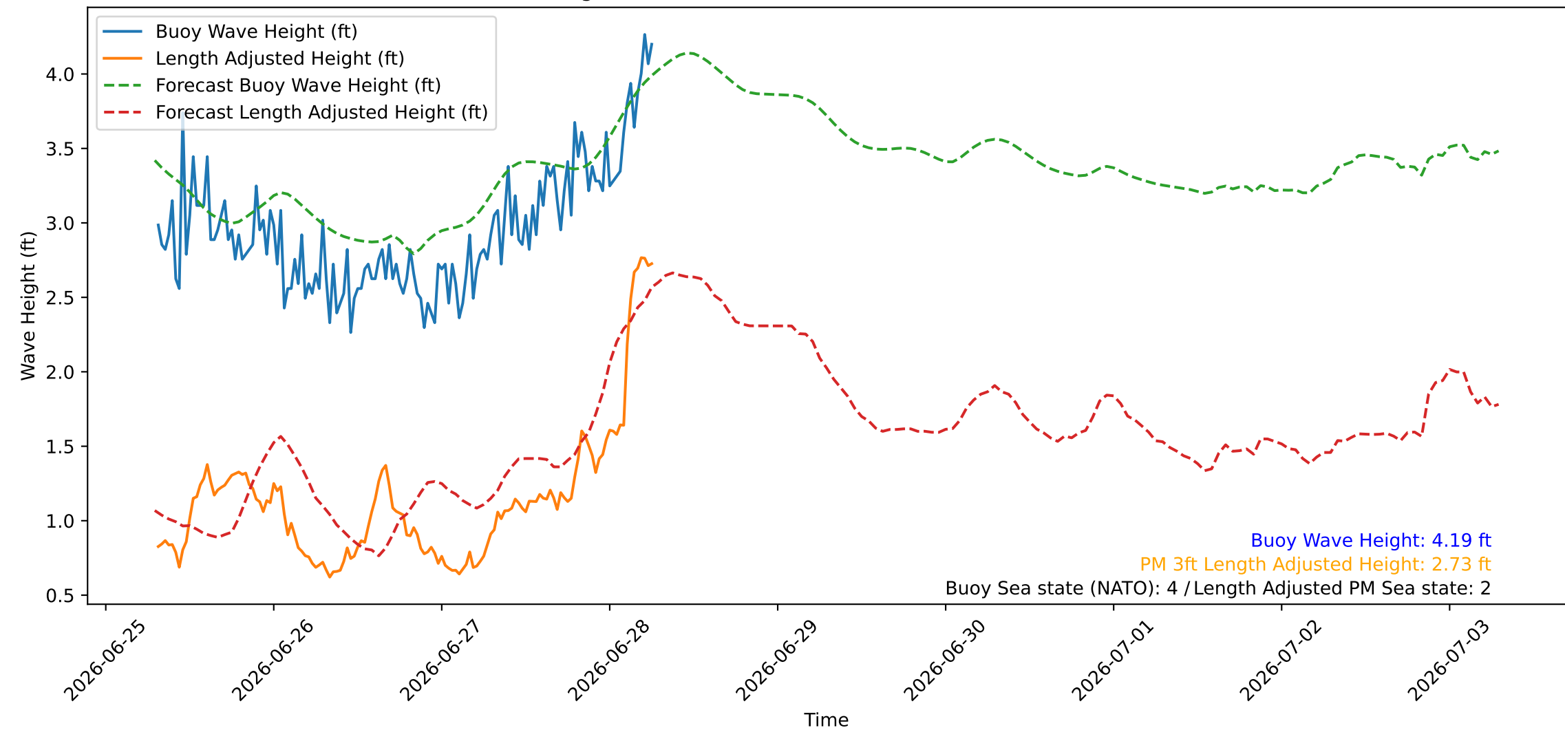
Wave Heights over Time for Red Beach at 2026-06-28 07:00:45
