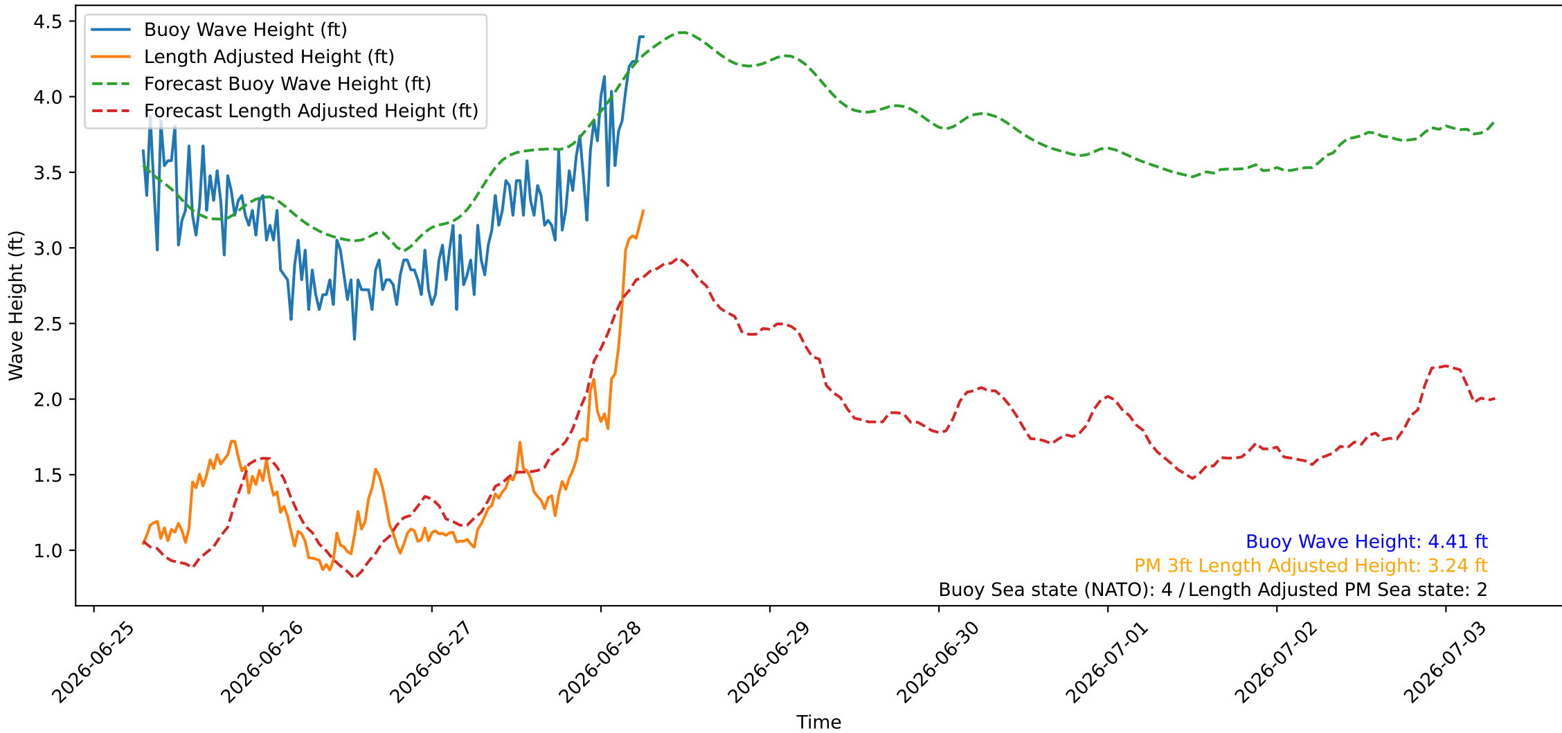
Wave Heights over Time for Oceanside Harbor at 2026-06-28 07:00:26
