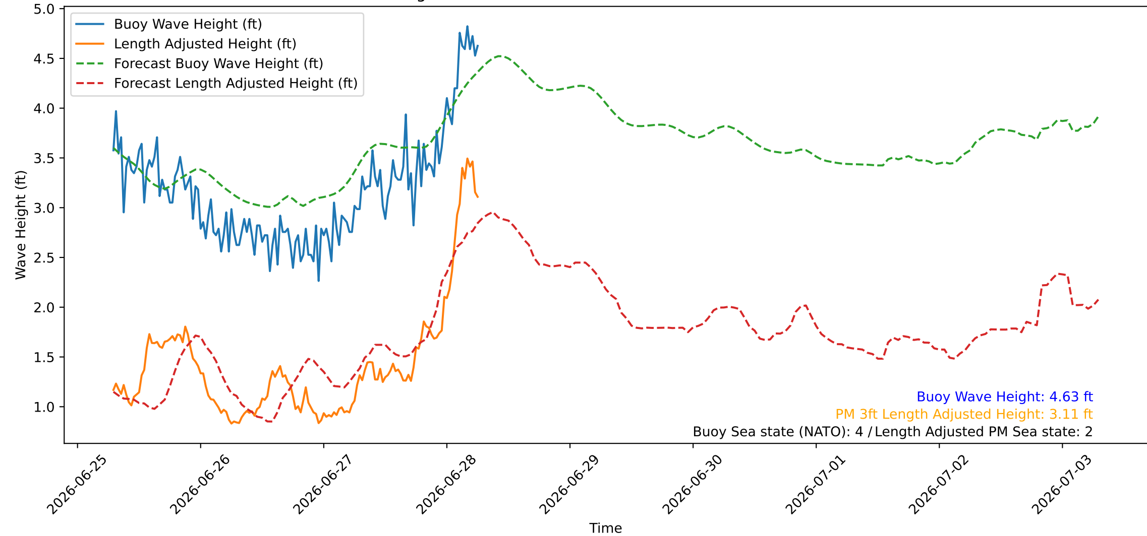
Wave Heights over Time for Green Beach at 2026-06-28 07:01:07
