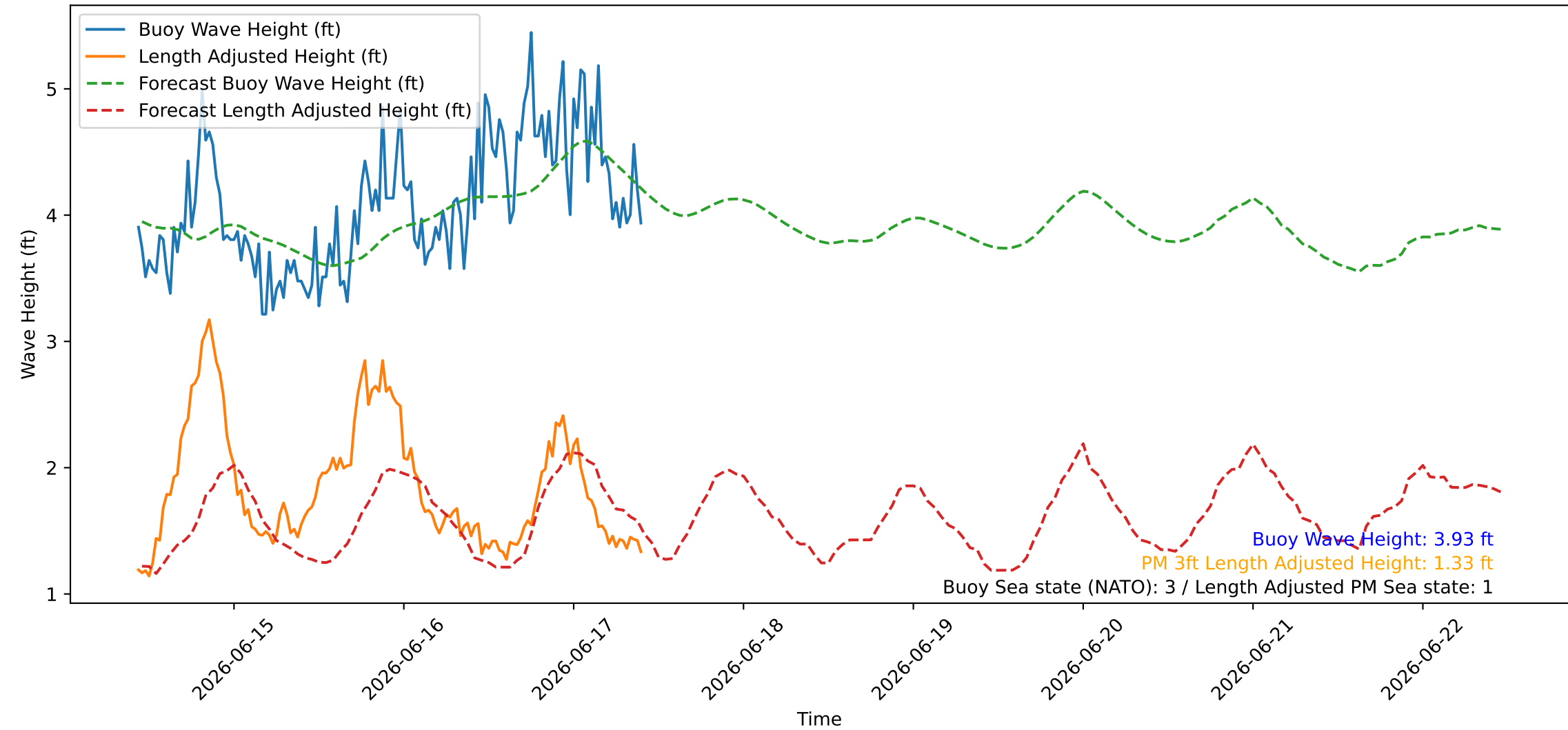
Wave Heights over Time for Oceanside Harbor at 2026-06-17 10:30:26
