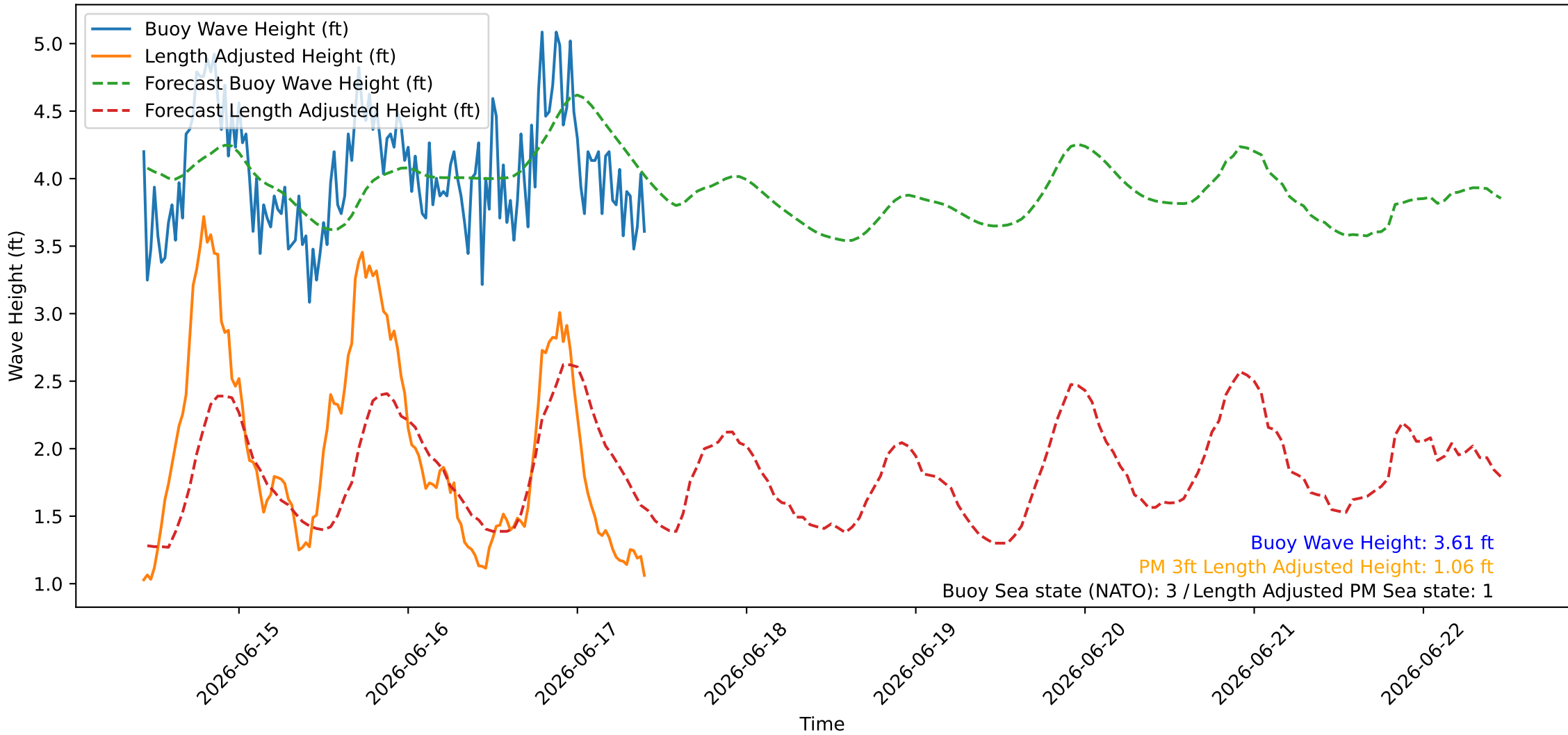
Wave Heights over Time for Green Beach at 2026-06-17 10:31:10
