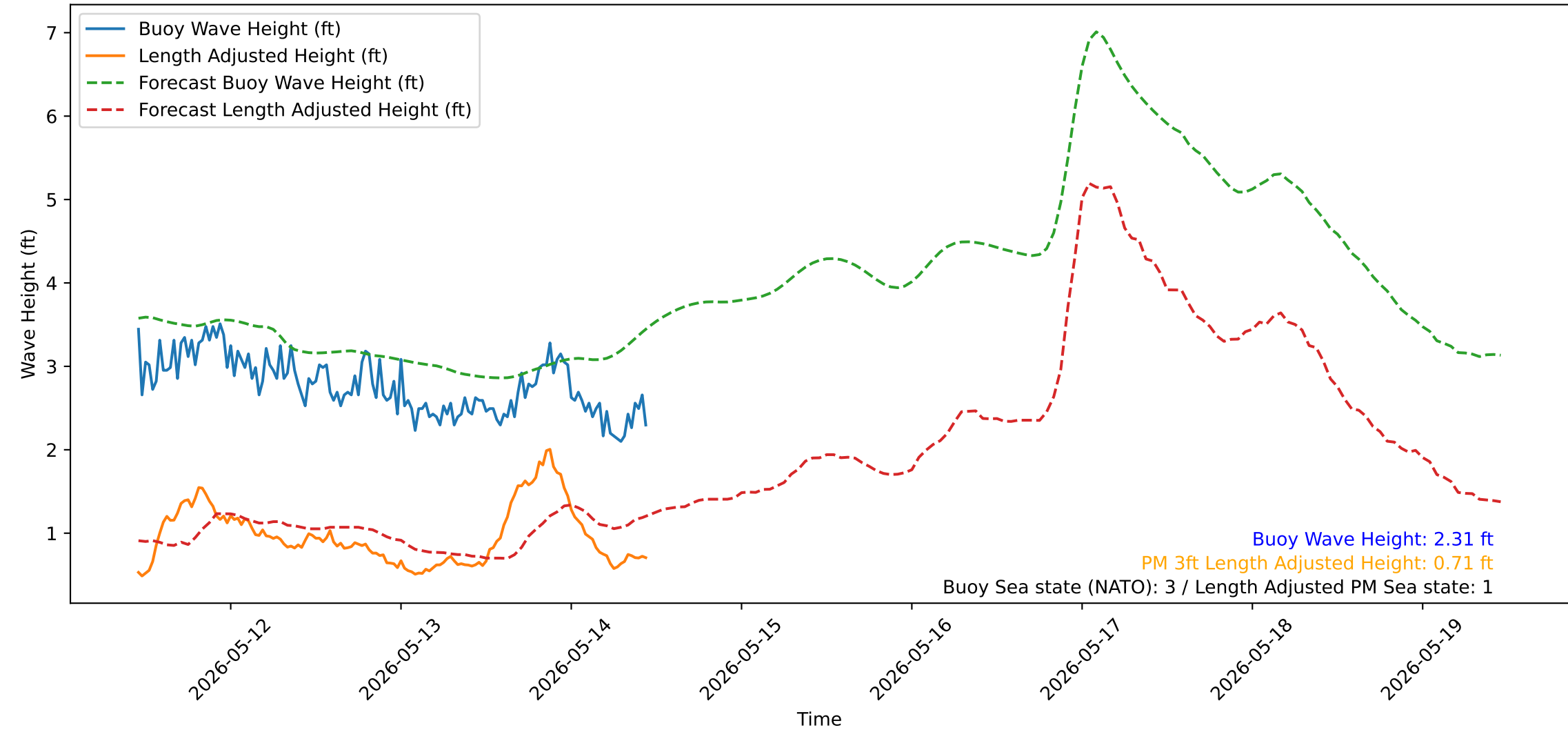
Wave Heights over Time for Green Beach at 2026-05-14 11:11:13
