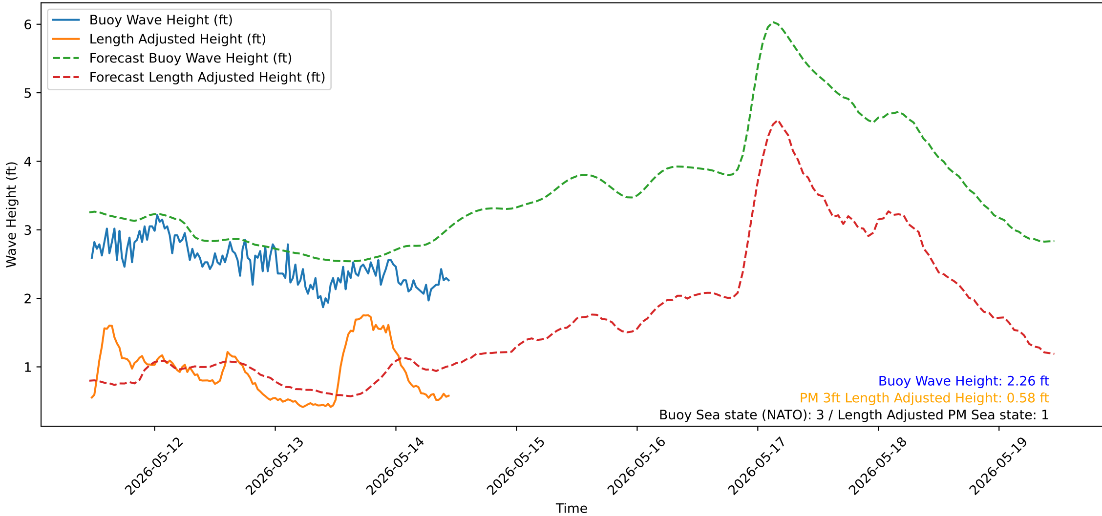
Wave Heights over Time for Red Beach at 2026-05-14 11:10:51
