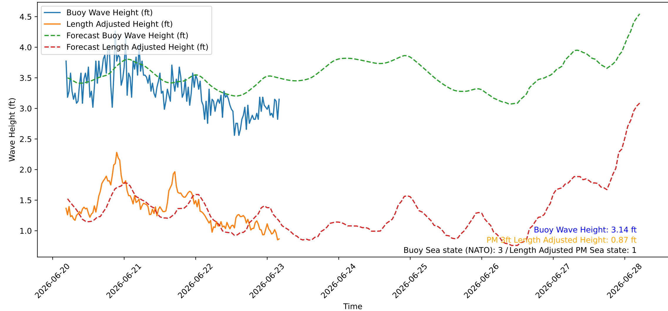
Wave Heights over Time for Oceanside Harbor at 2026-06-23 04:30:27
