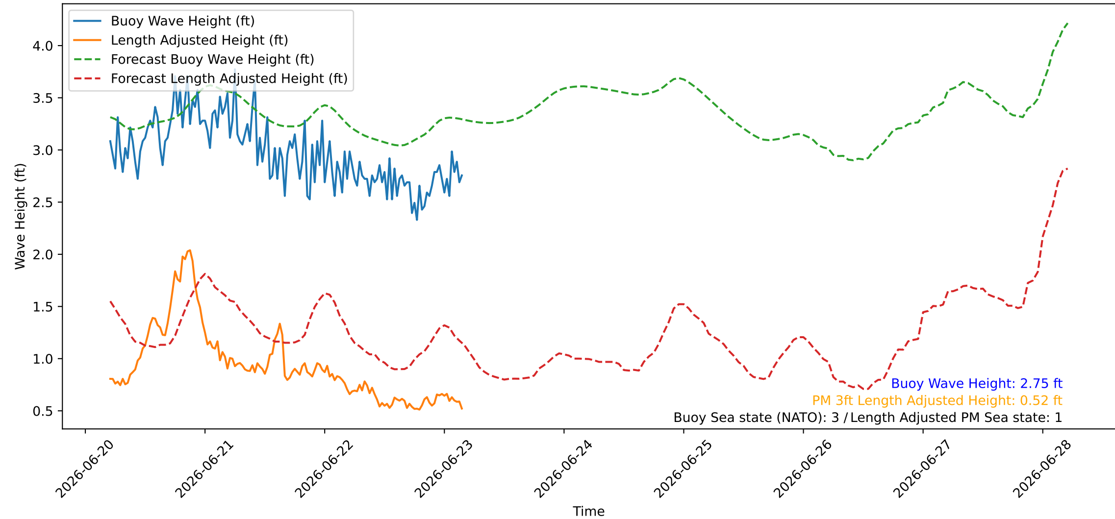
Wave Heights over Time for Red Beach at 2026-06-23 04:30:45
