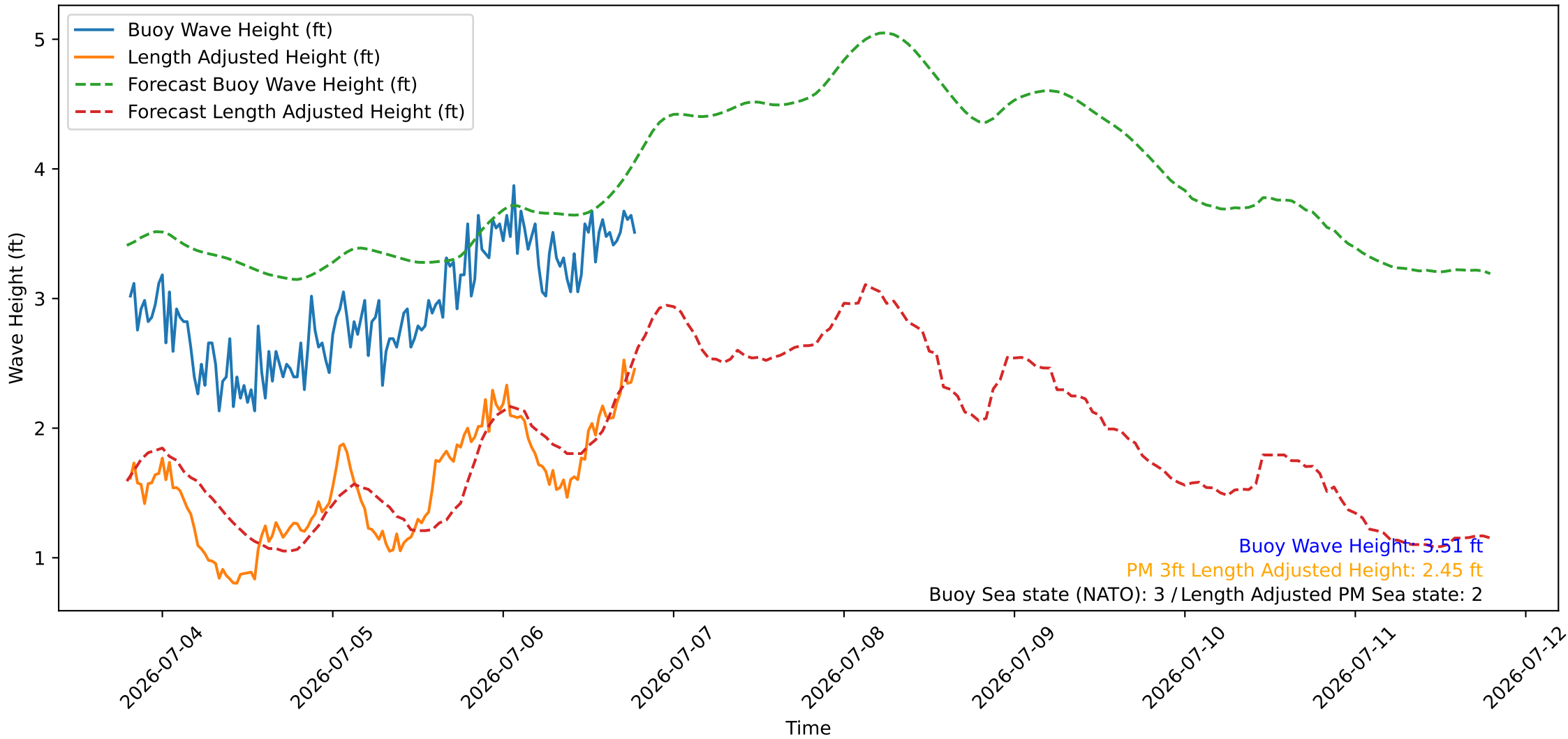
Wave Heights over Time for Oceanside Harbor at 2026-07-06 19:20:27
