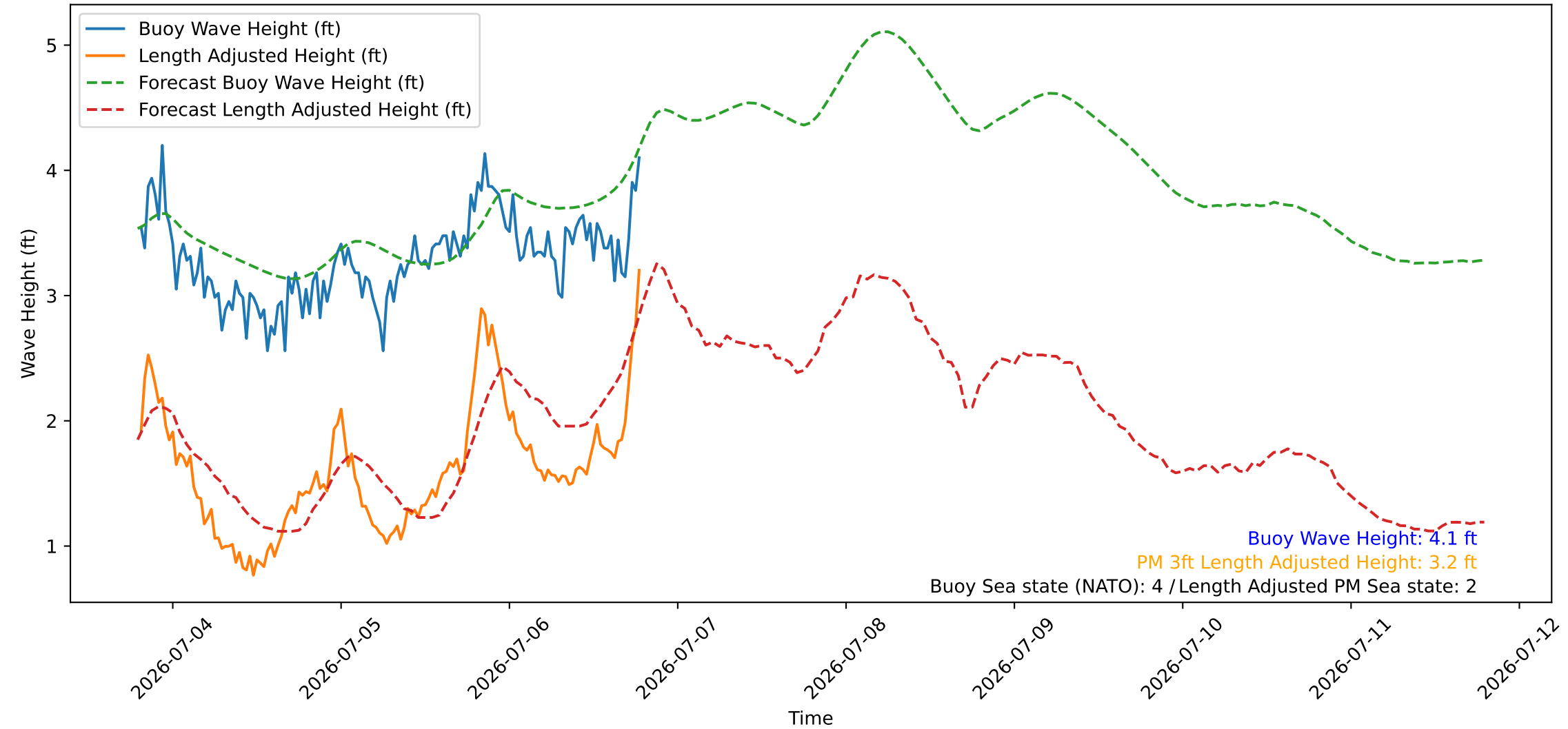
Wave Heights over Time for Green Beach at 2026-07-06 19:21:10
