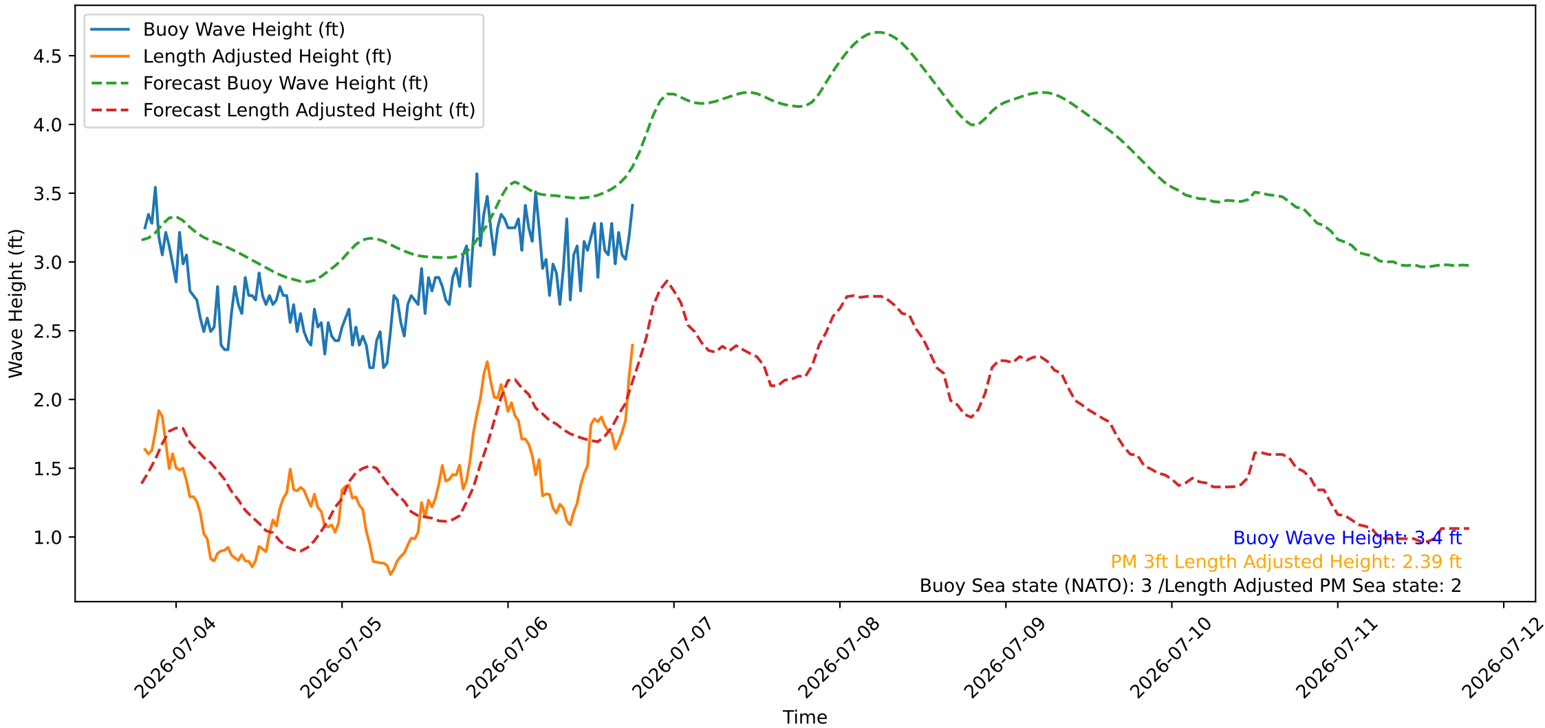
Wave Heights over Time for Red Beach at 2026-07-06 19:20:48
