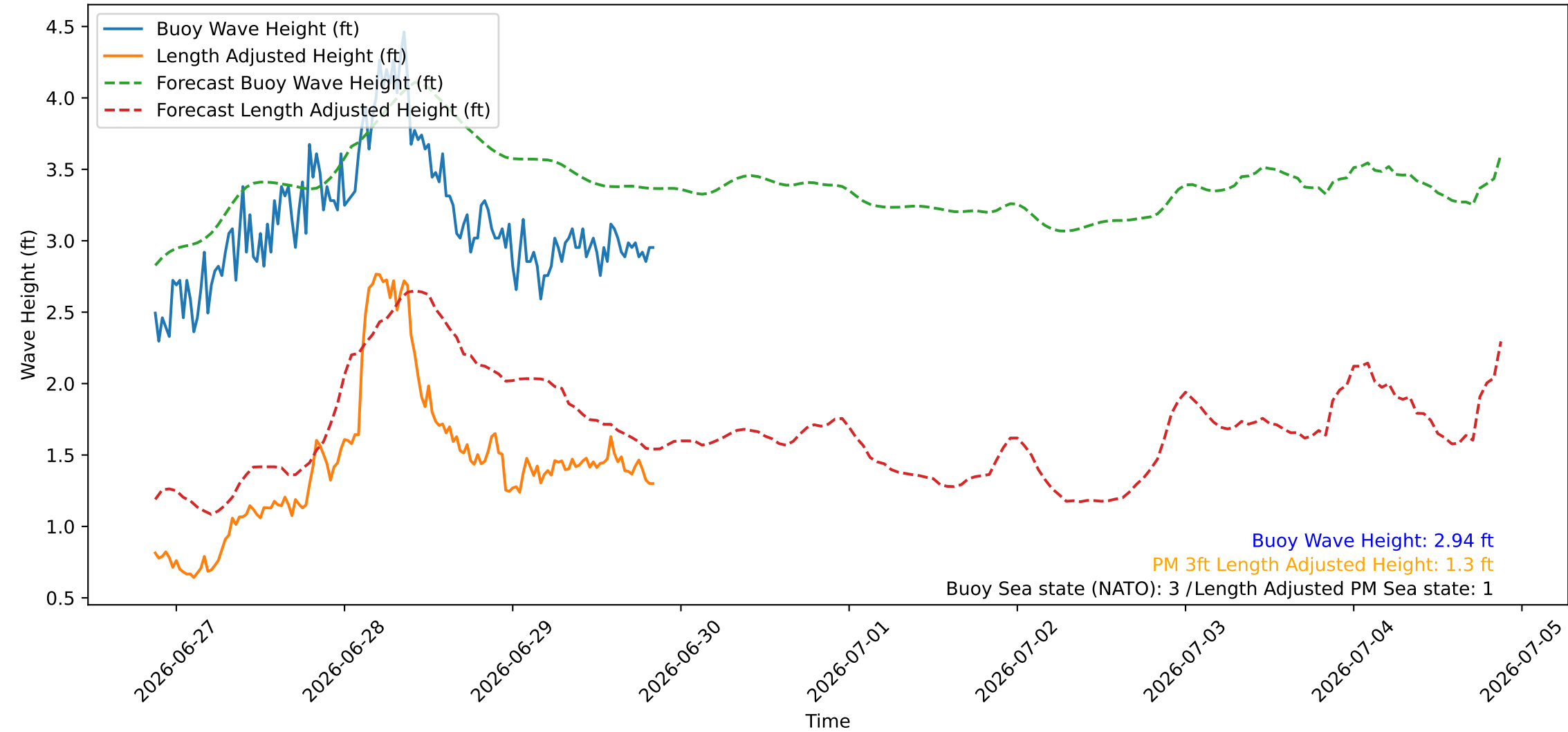
Wave Heights over Time for Red Beach at 2026-06-29 20:50:46
