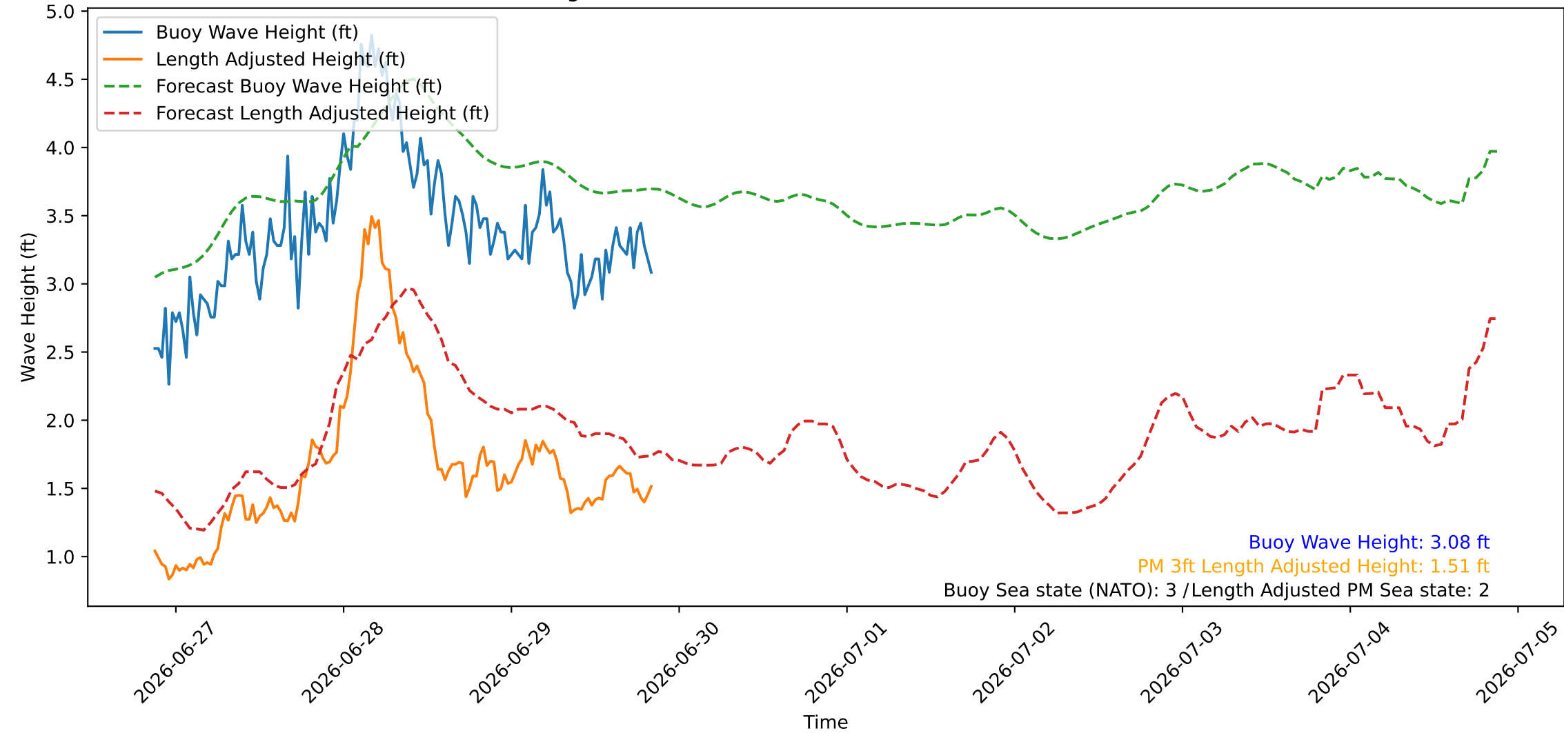
Wave Heights over Time for Green Beach at 2026-06-29 20:51:08
