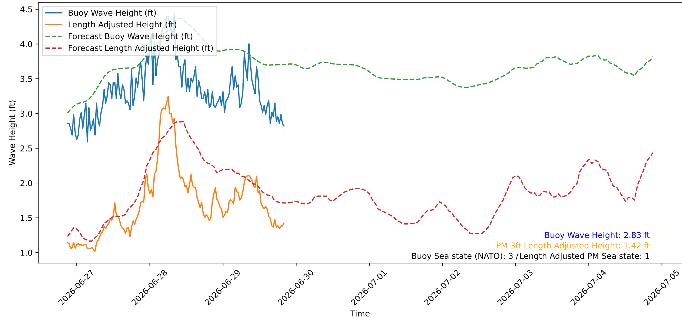
Wave Heights over Time for Oceanside Harbor at 2026-06-29 20:50:25
