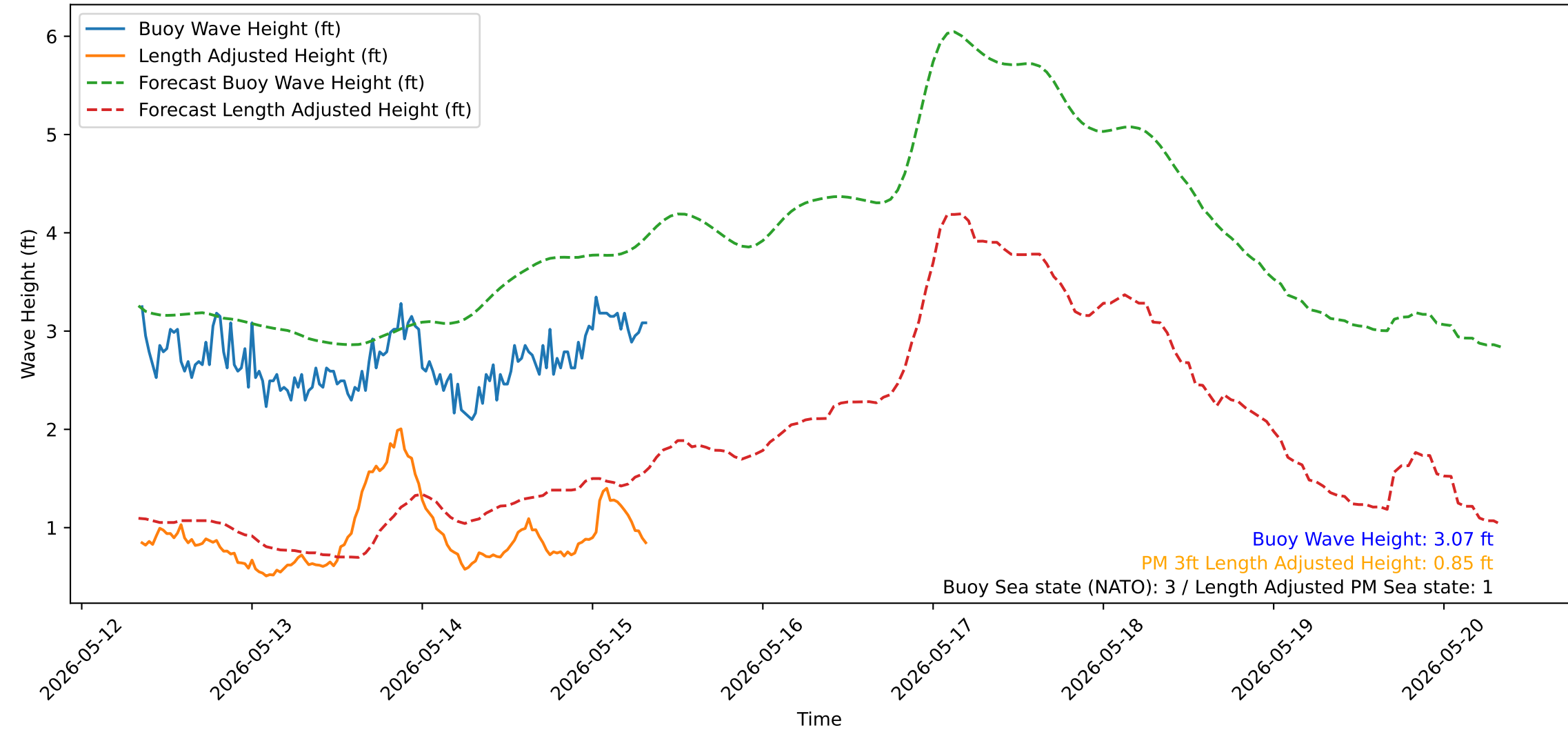
Wave Heights over Time for Green Beach at 2026-05-15 08:21:15
