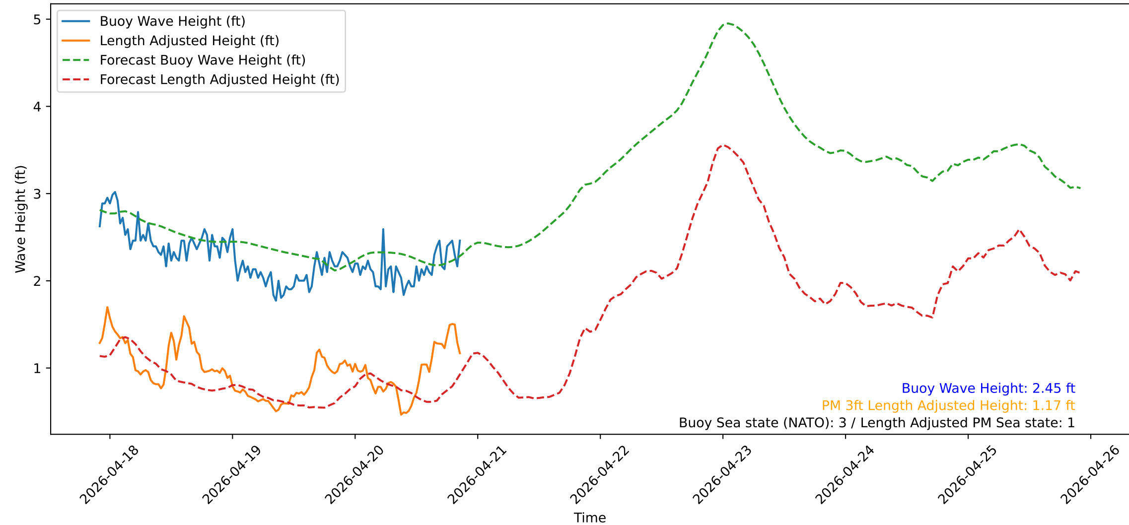
Wave Heights over Time for Red Beach at 2026-04-20 21:50:51
