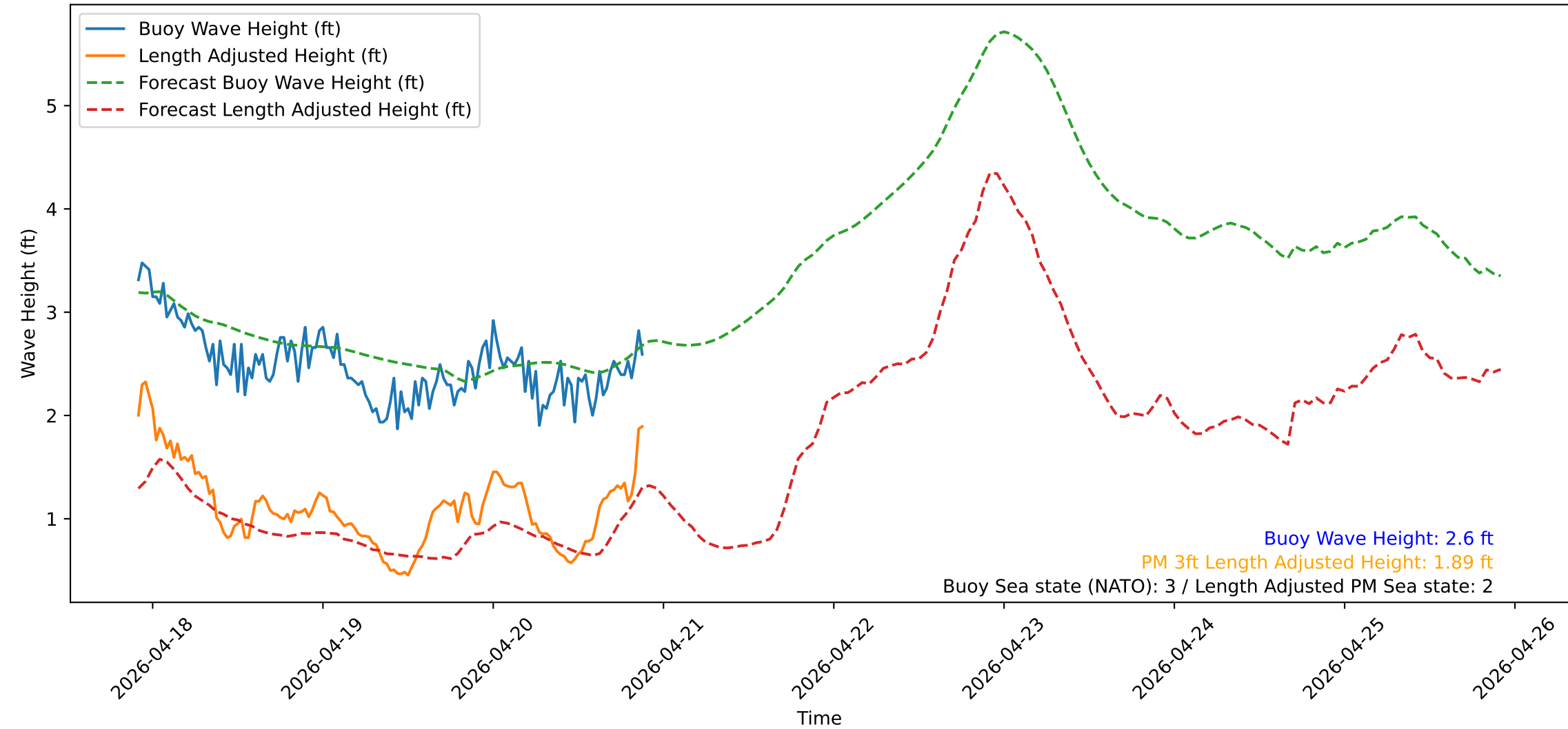
Wave Heights over Time for Green Beach at 2026-04-20 21:51:14
