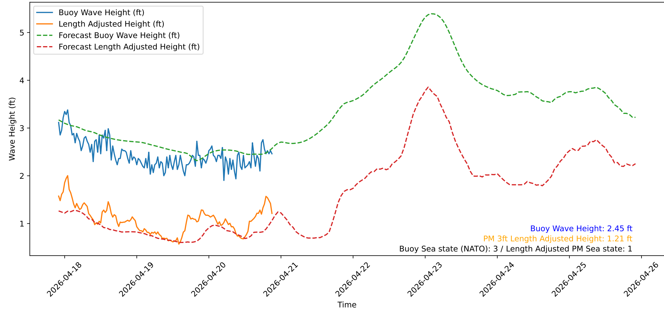
Wave Heights over Time for Oceanside Harbor at 2026-04-20 21:50:31
