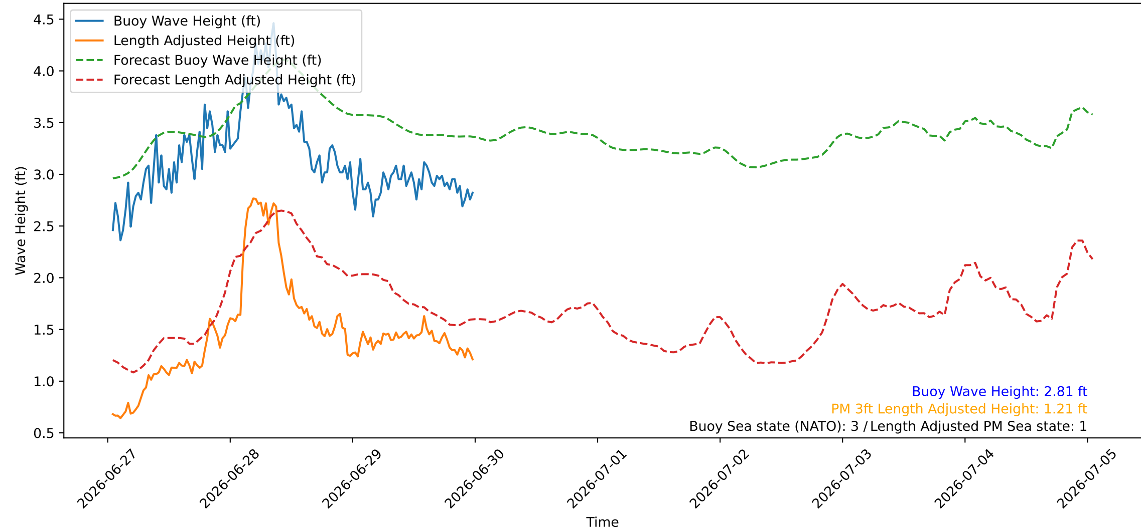
Wave Heights over Time for Red Beach at 2026-06-30 00:30:45
