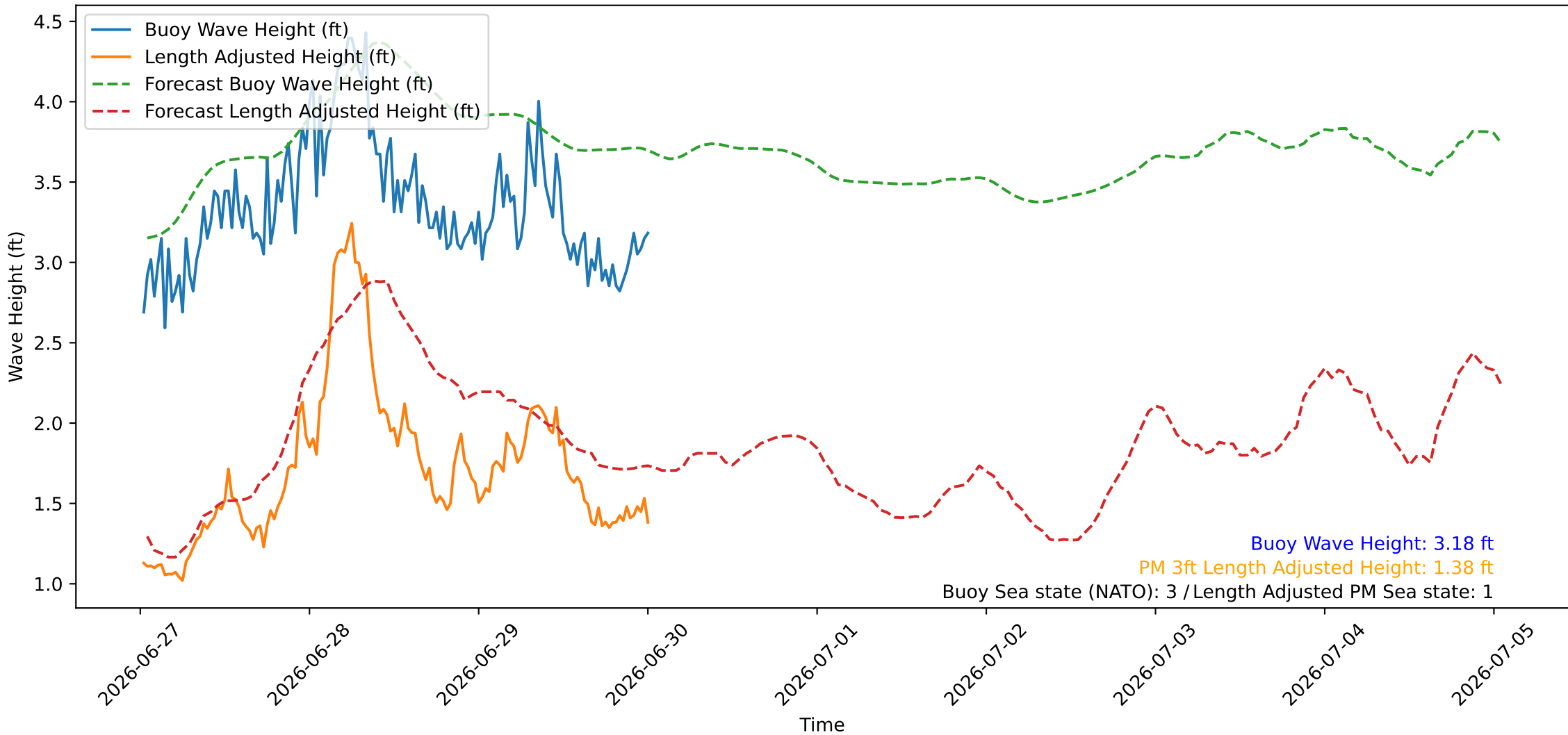
Wave Heights over Time for Oceanside Harbor at 2026-06-30 00:30:26
