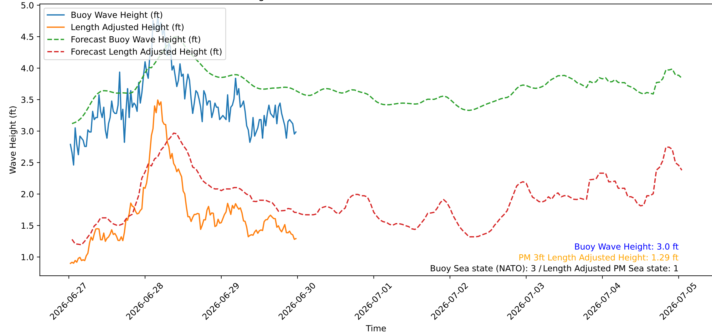
Wave Heights over Time for Green Beach at 2026-06-30 00:31:07
