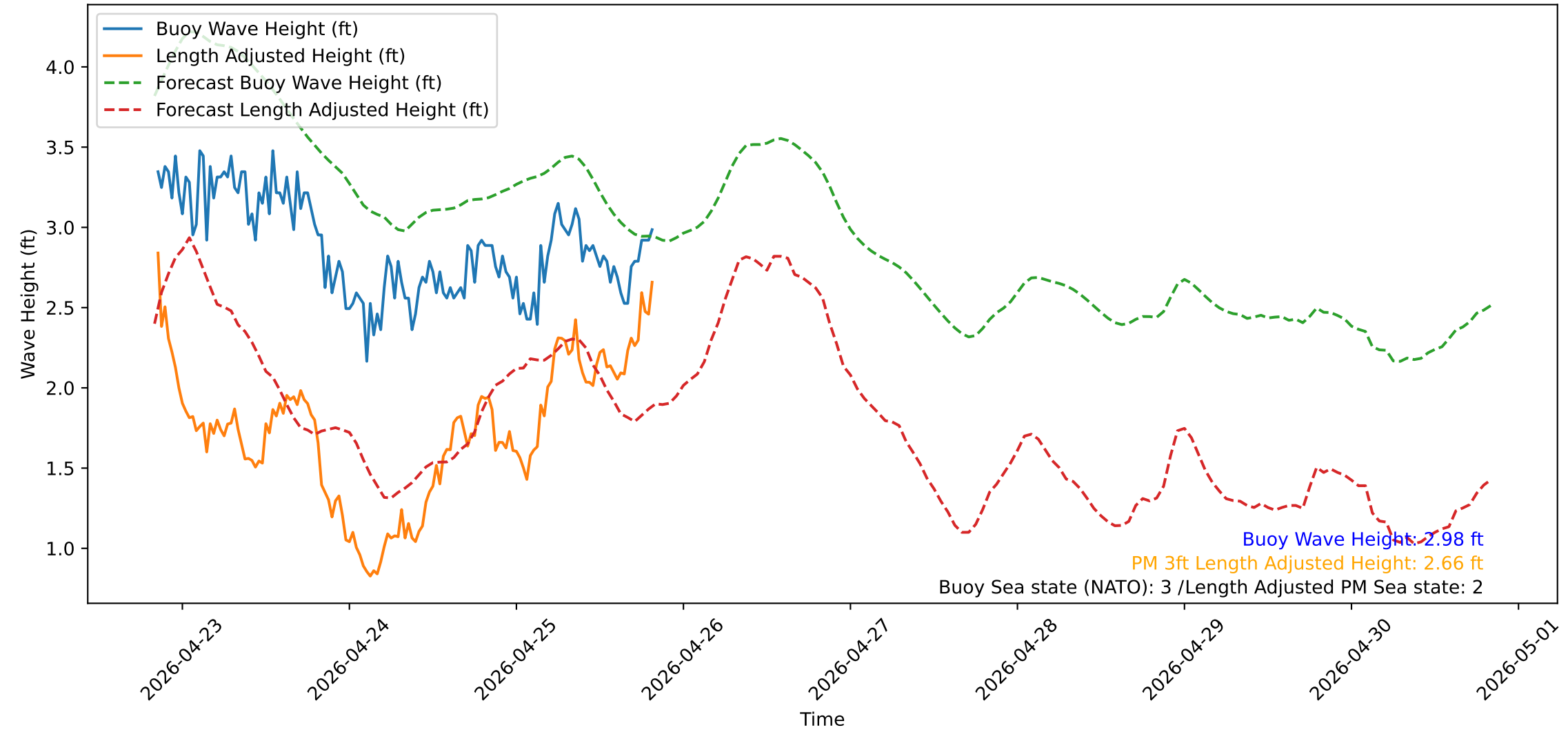
Wave Heights over Time for Red Beach at 2026-04-25 20:20:51
