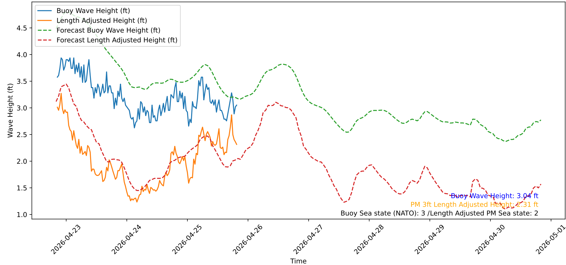
Wave Heights over Time for Green Beach at 2026-04-25 20:21:13
