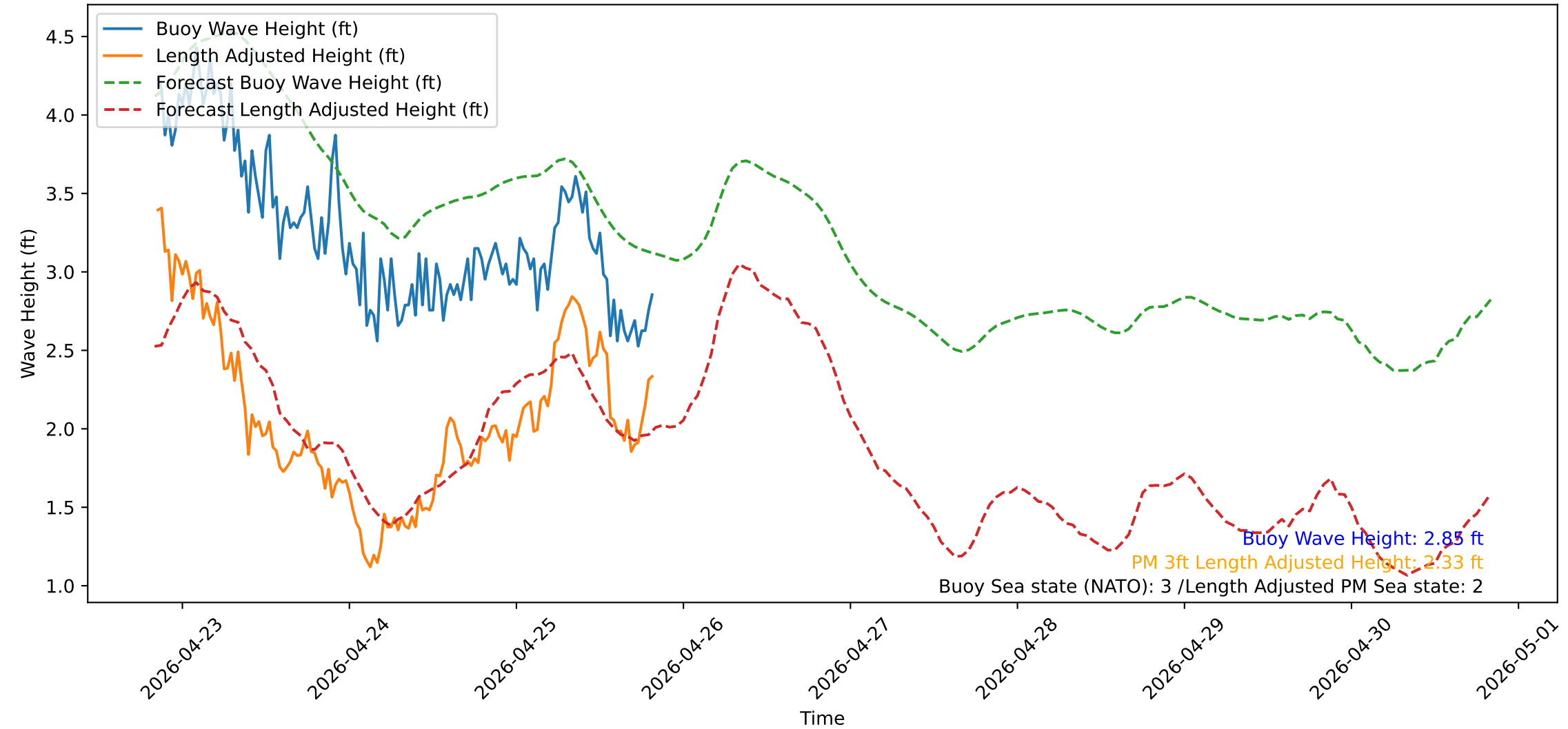
Wave Heights over Time for Oceanside Harbor at 2026-04-25 20:20:31
