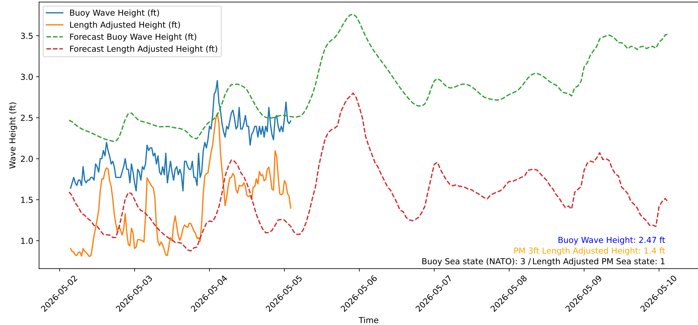
Wave Heights over Time for Red Beach at 2026-05-05 03:00:51
