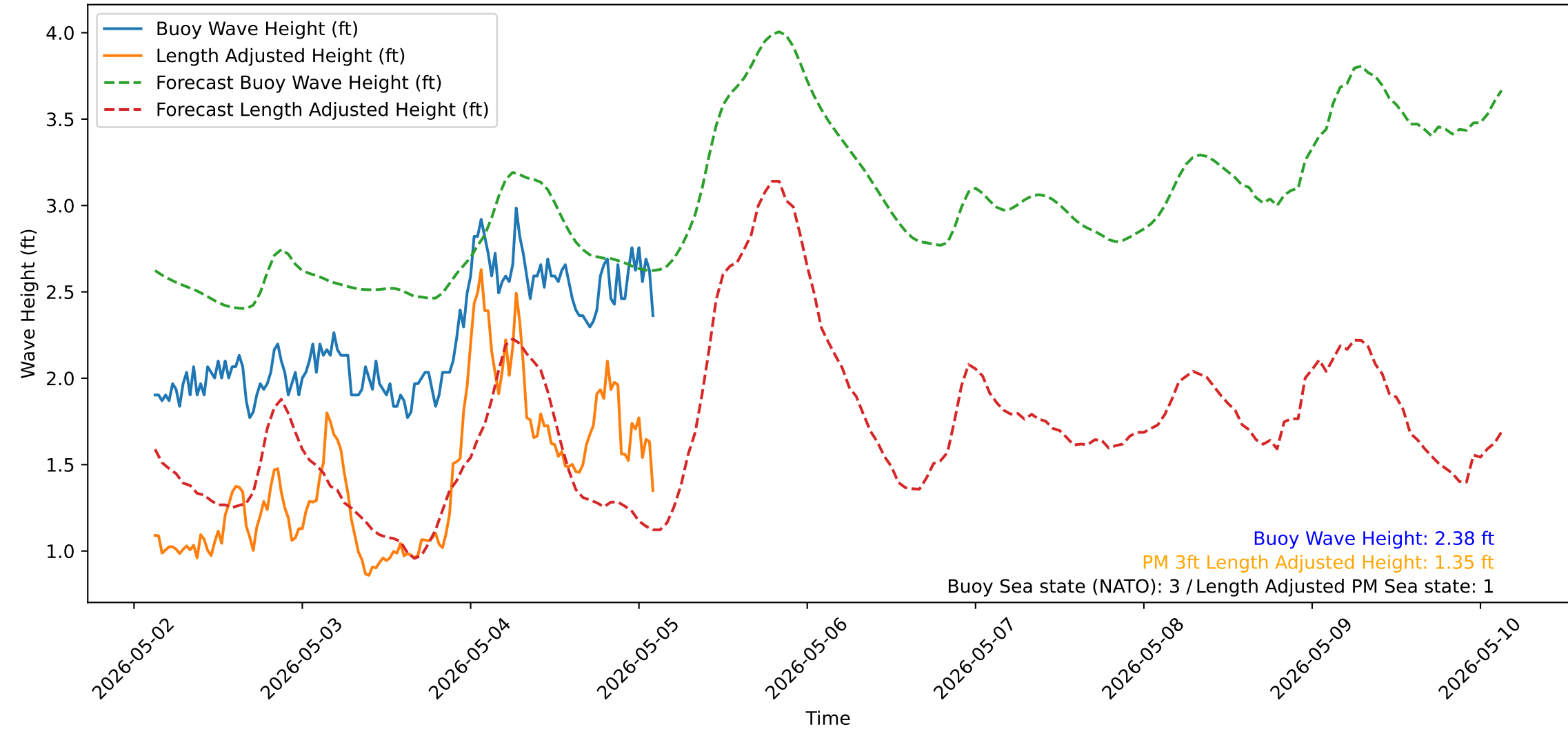
Wave Heights over Time for Green Beach at 2026-05-05 03:01:13
