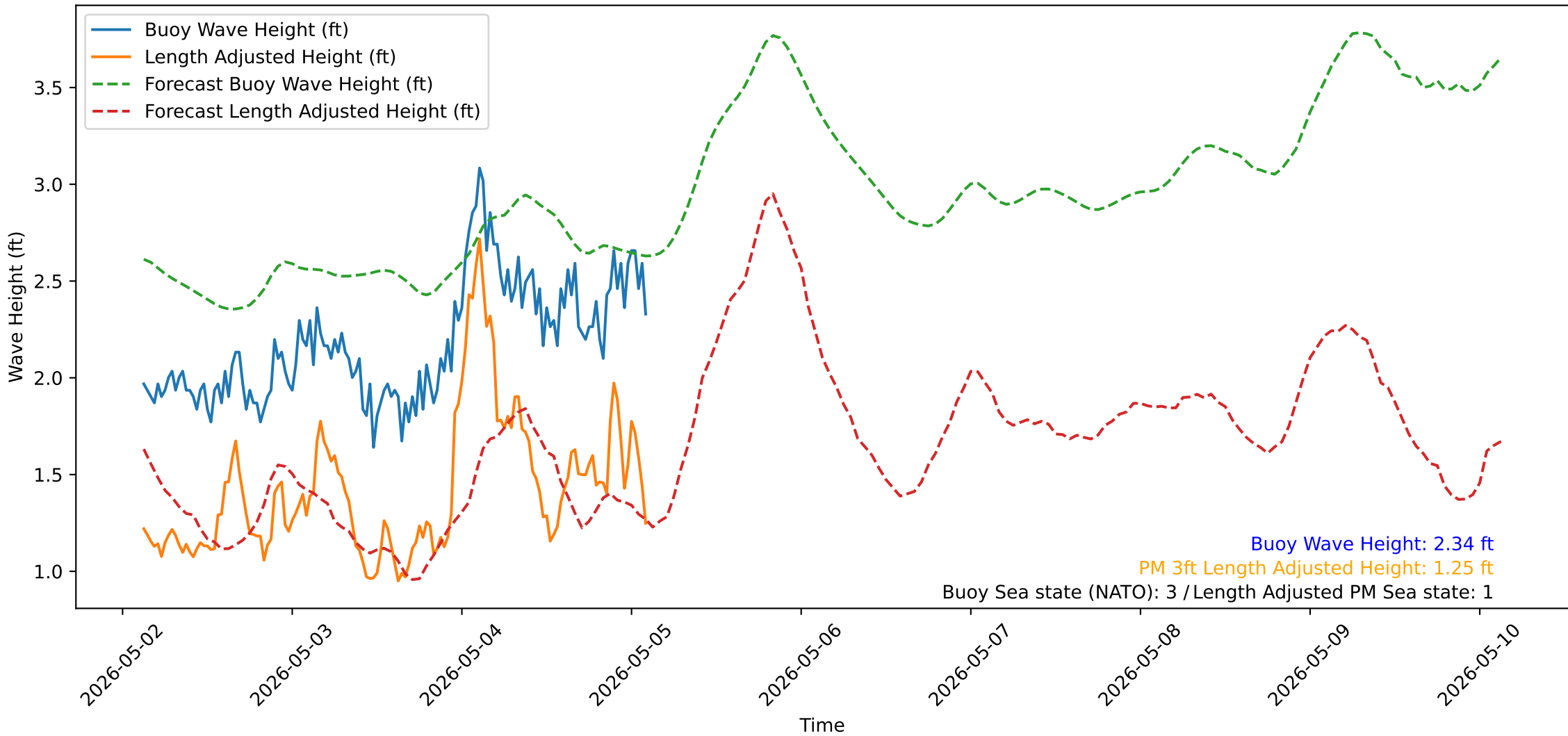
Wave Heights over Time for Oceanside Harbor at 2026-05-05 03:00:31
