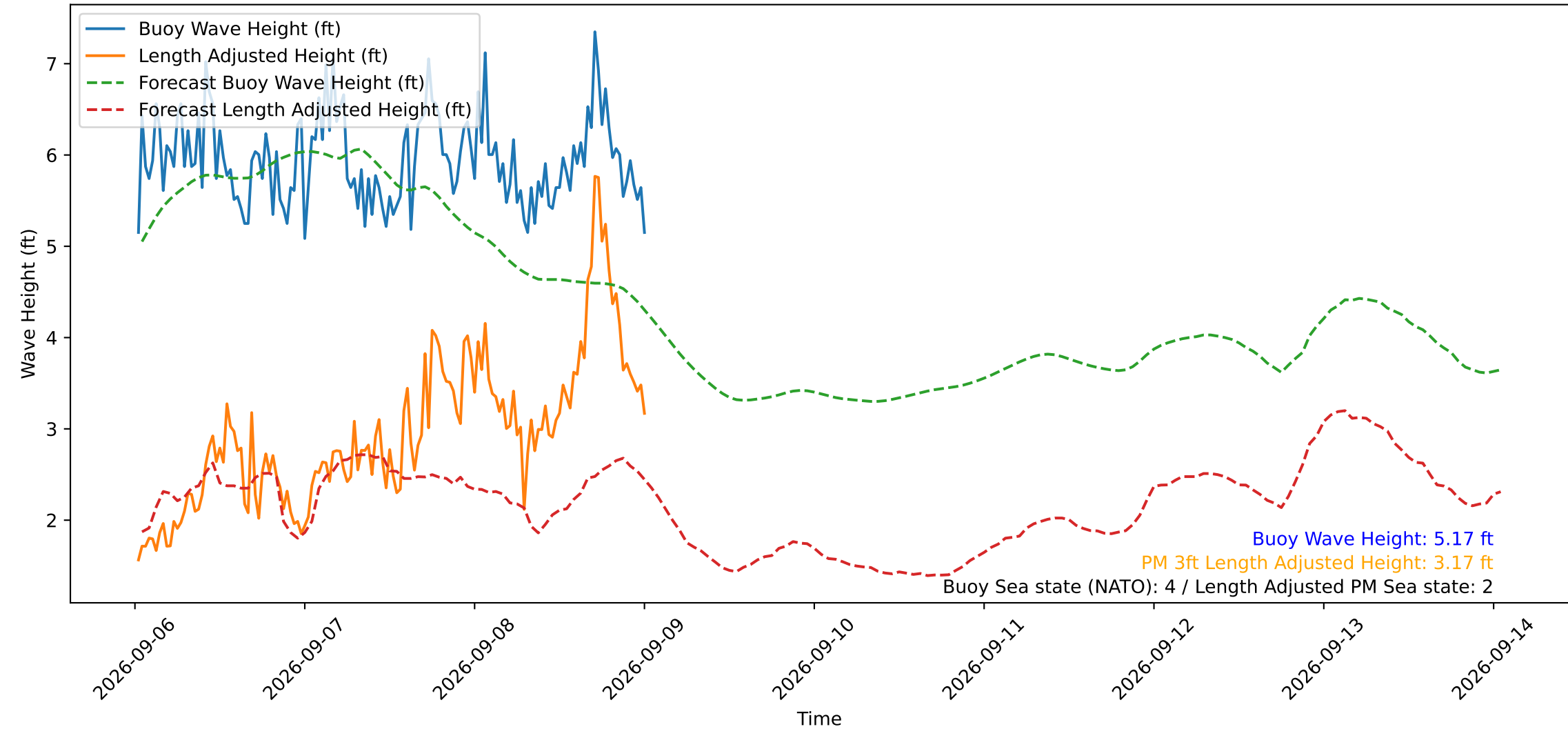
Wave Heights over Time for Oceanside Harbor at 2026-09-09 00:40:29
