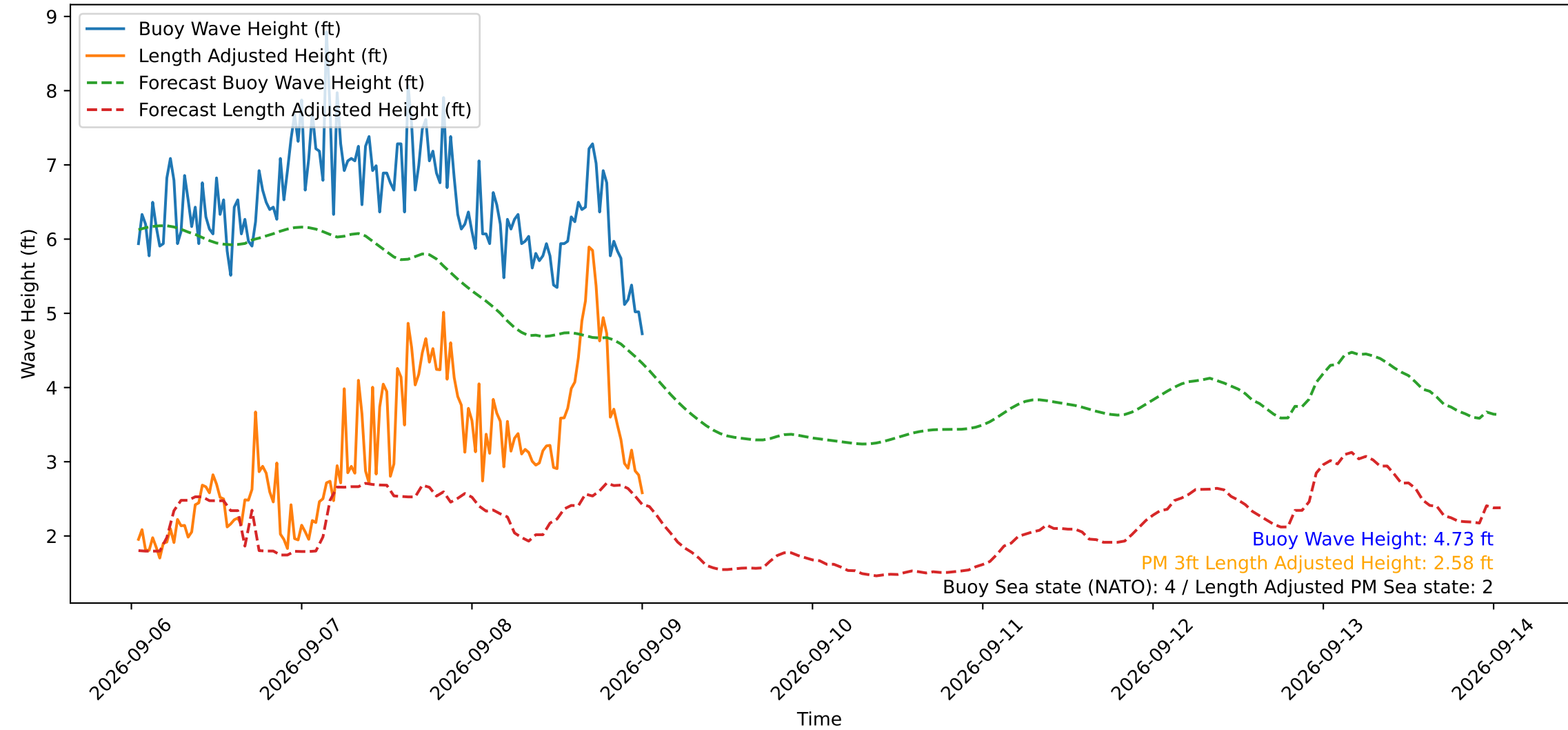
Wave Heights over Time for Green Beach at 2026-09-09 00:41:10
