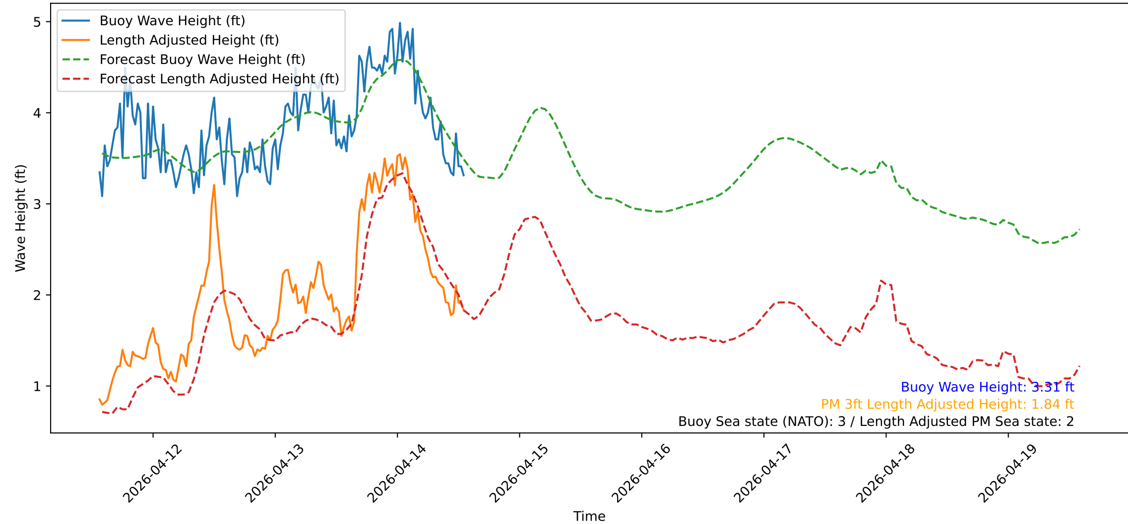
Wave Heights over Time for Green Beach at 2026-04-14 13:41:13
