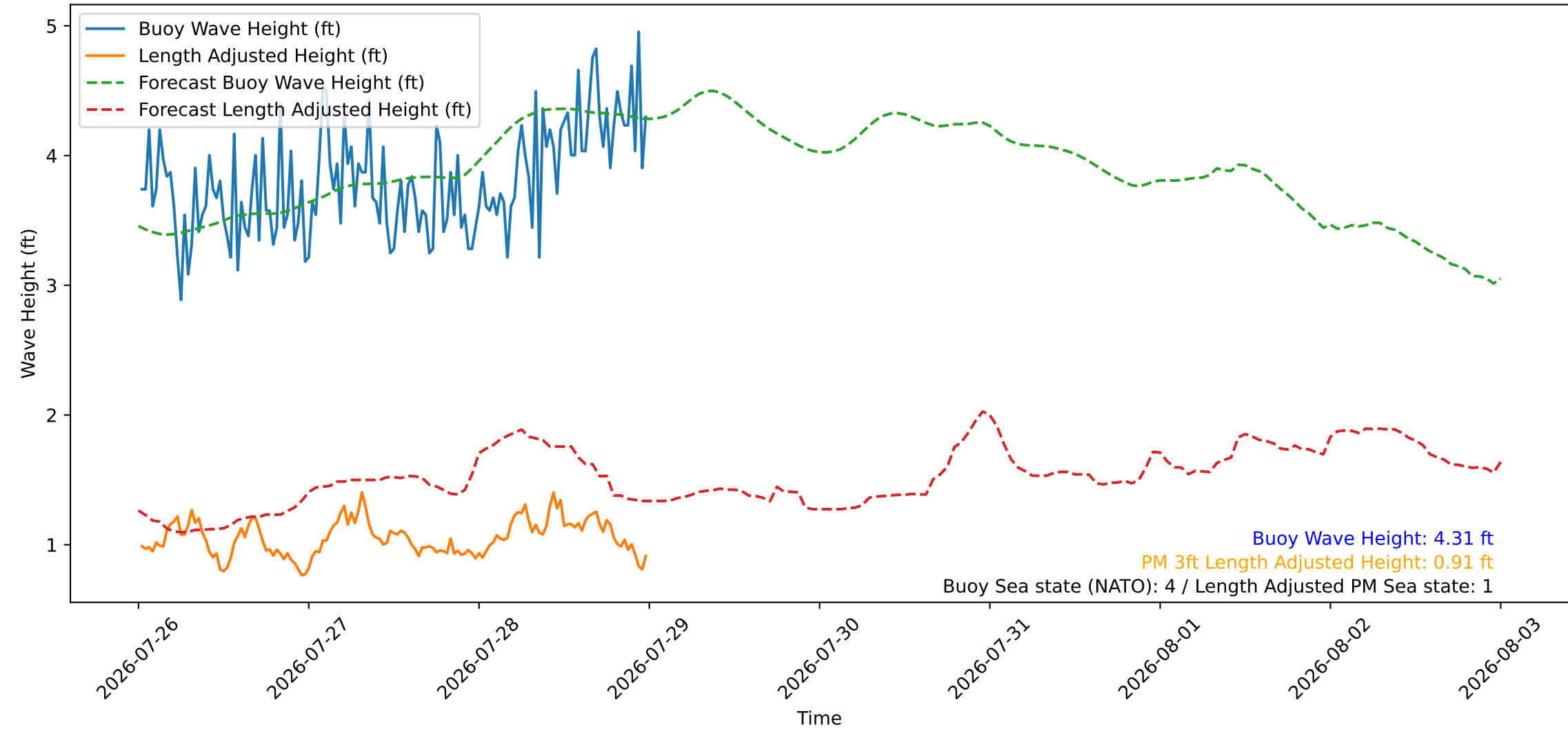
Wave Heights over Time for Red Beach at 2026-07-29 00:10:46
