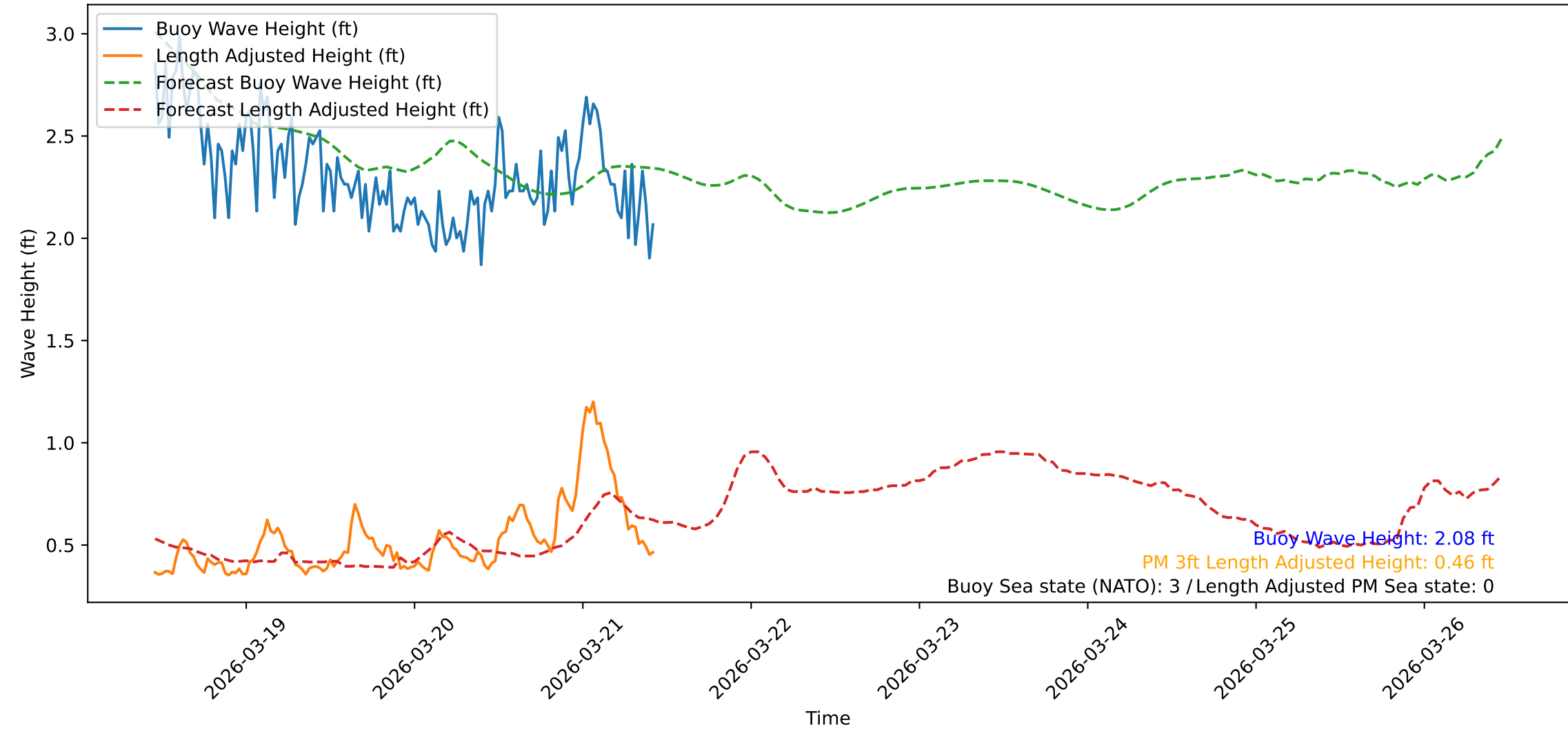
Wave Heights over Time for Red Beach at 2026-03-21 10:50:47
