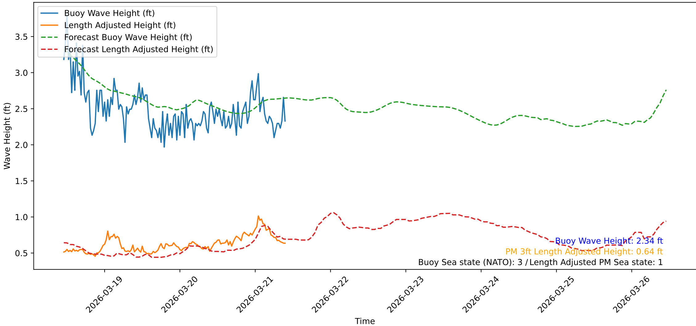
Wave Heights over Time for Oceanside Harbor at 2026-03-21 10:50:31
