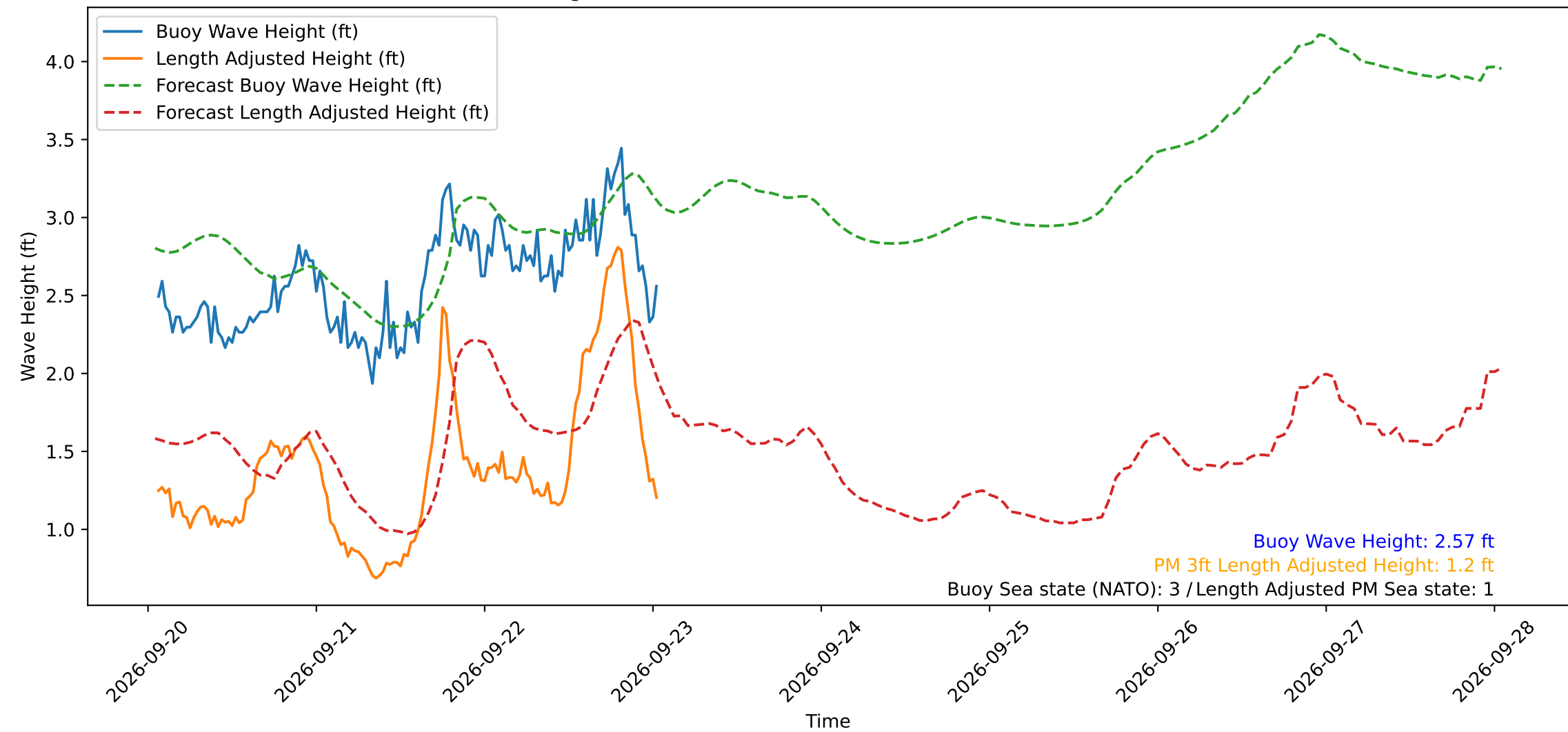
Wave Heights over Time for Green Beach at 2026-09-23 01:11:10
