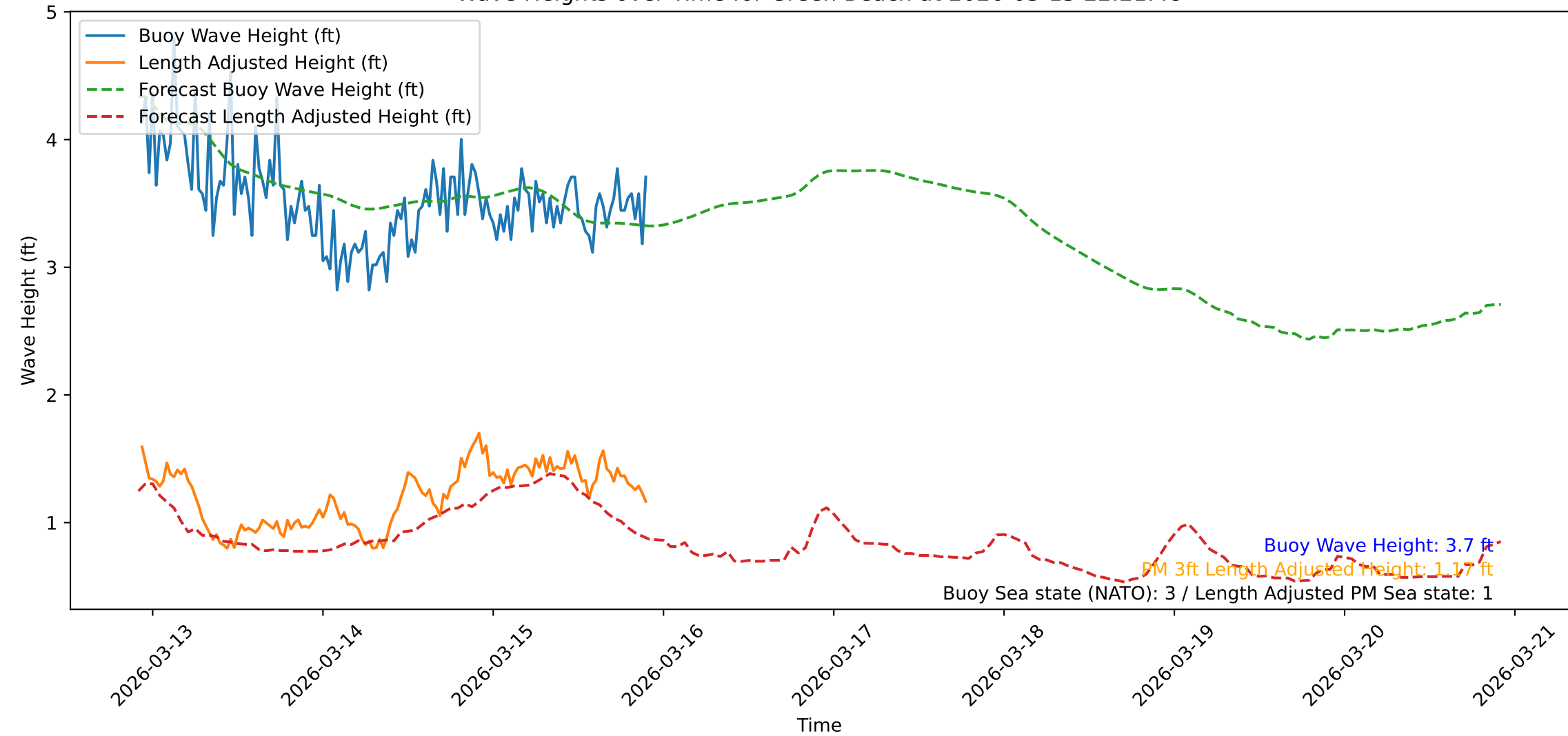
Wave Heights over Time for Green Beach at 2026-03-15 22:21:48
