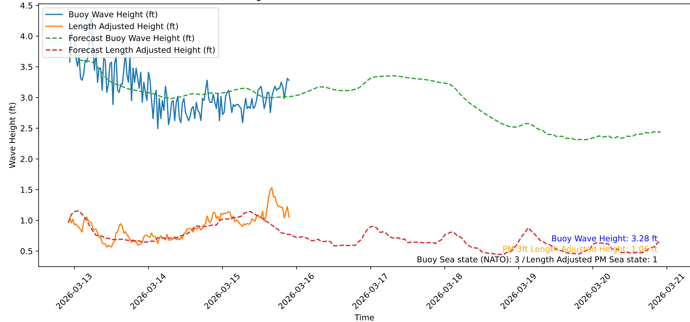
Wave Heights over Time for Red Beach at 2026-03-15 22:21:09
