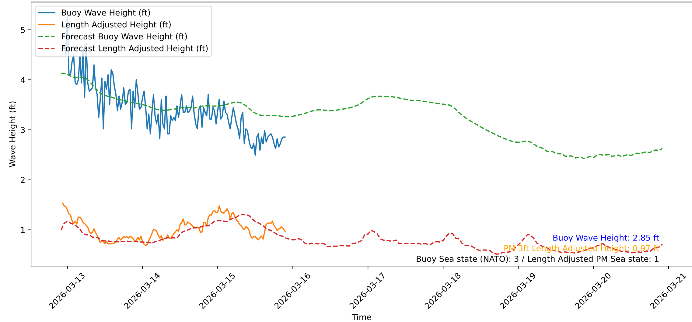
Wave Heights over Time for Oceanside Harbor at 2026-03-15 22:20:41
