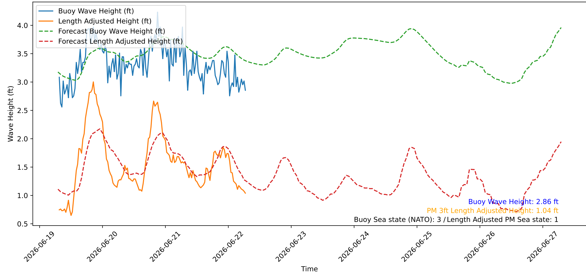
Wave Heights over Time for Green Beach at 2026-06-22 07:21:09
