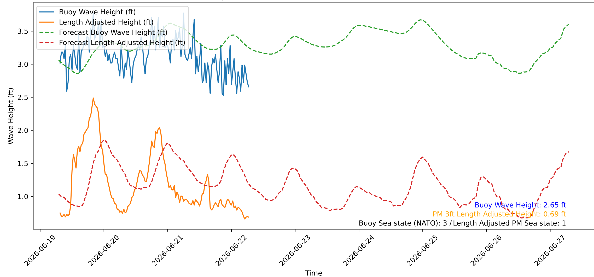
Wave Heights over Time for Red Beach at 2026-06-22 07:20:47
