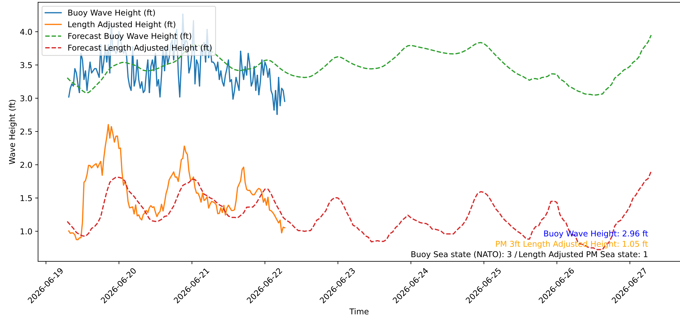
Wave Heights over Time for Oceanside Harbor at 2026-06-22 07:20:26
