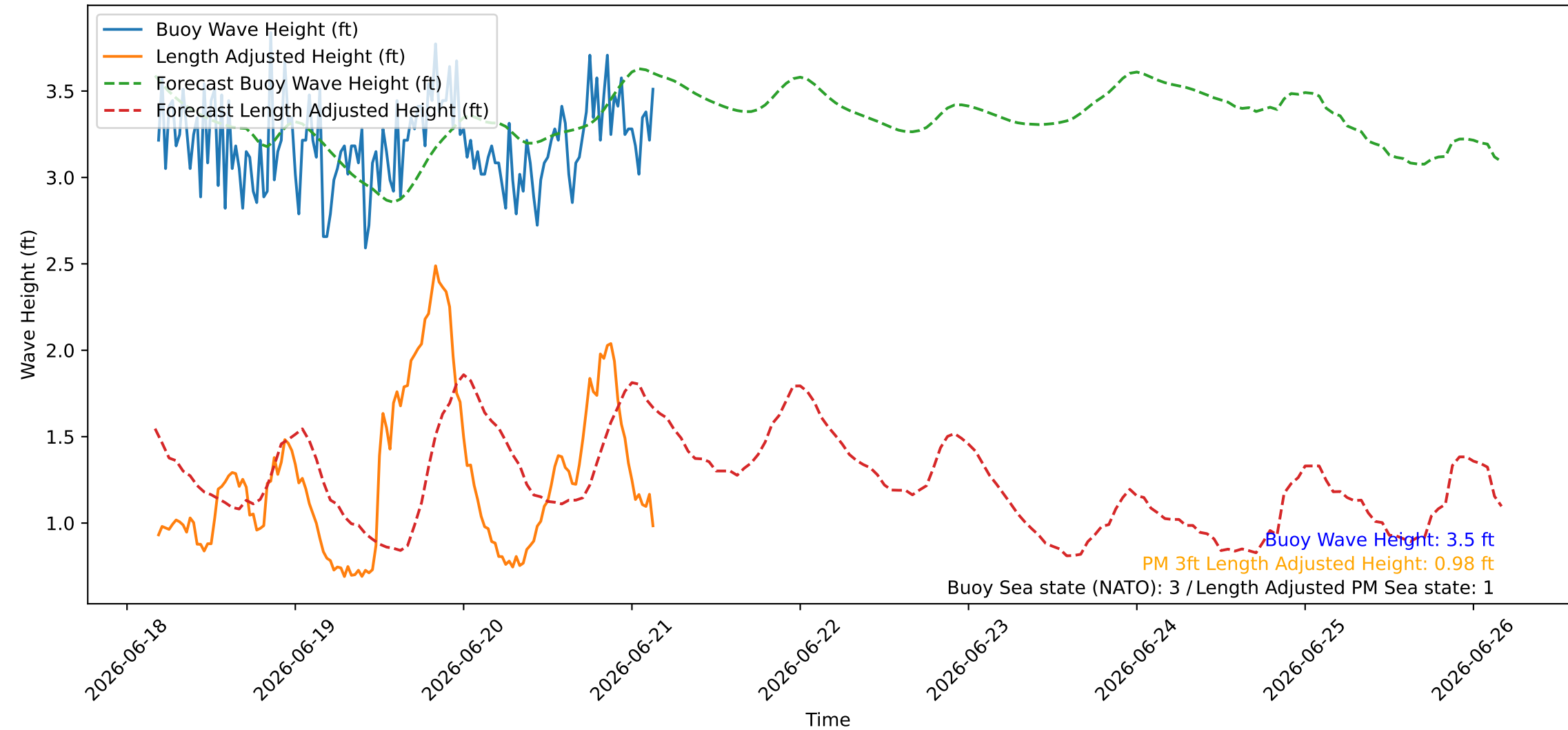
Wave Heights over Time for Red Beach at 2026-06-21 04:00:44
