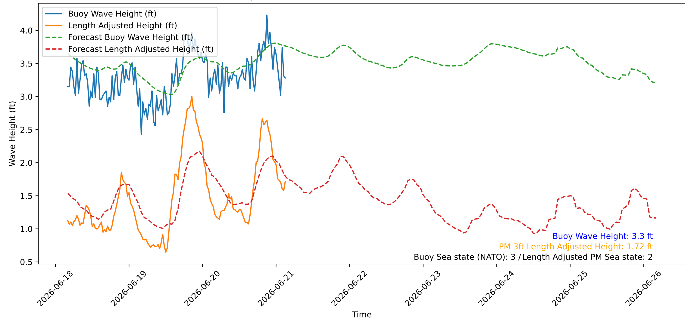
Wave Heights over Time for Green Beach at 2026-06-21 04:01:07
