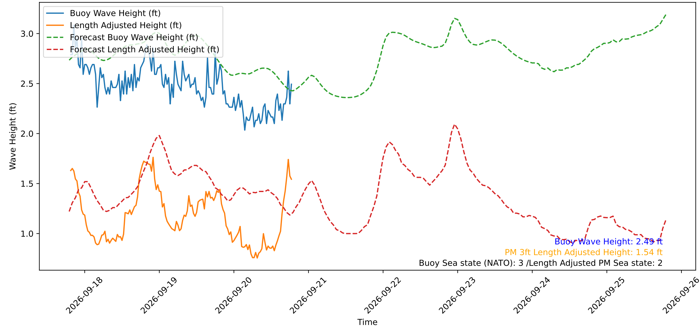
Wave Heights over Time for Red Beach at 2026-09-20 19:10:49
