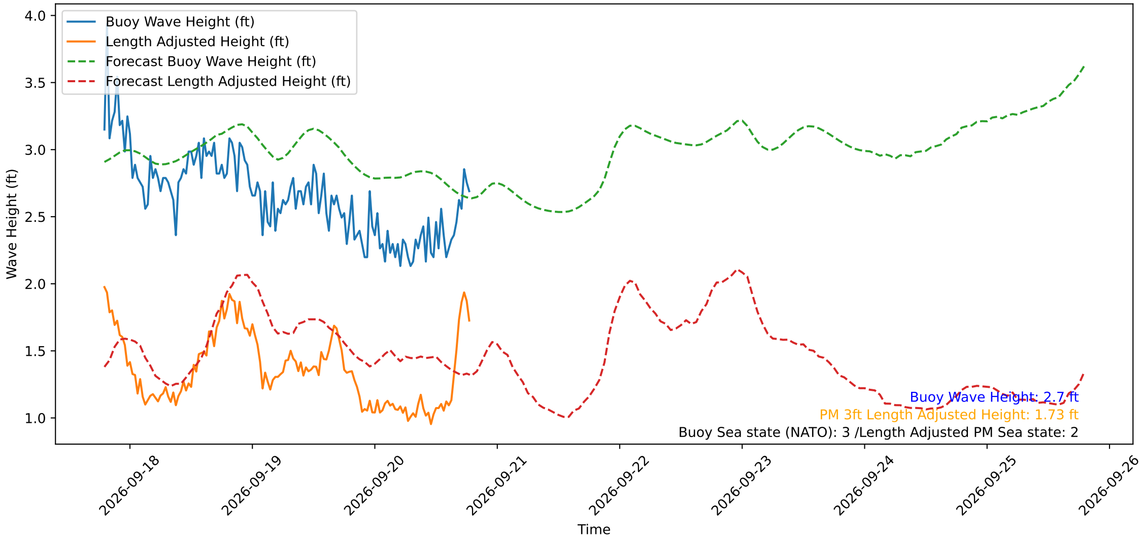
Wave Heights over Time for Oceanside Harbor at 2026-09-20 19:10:29
