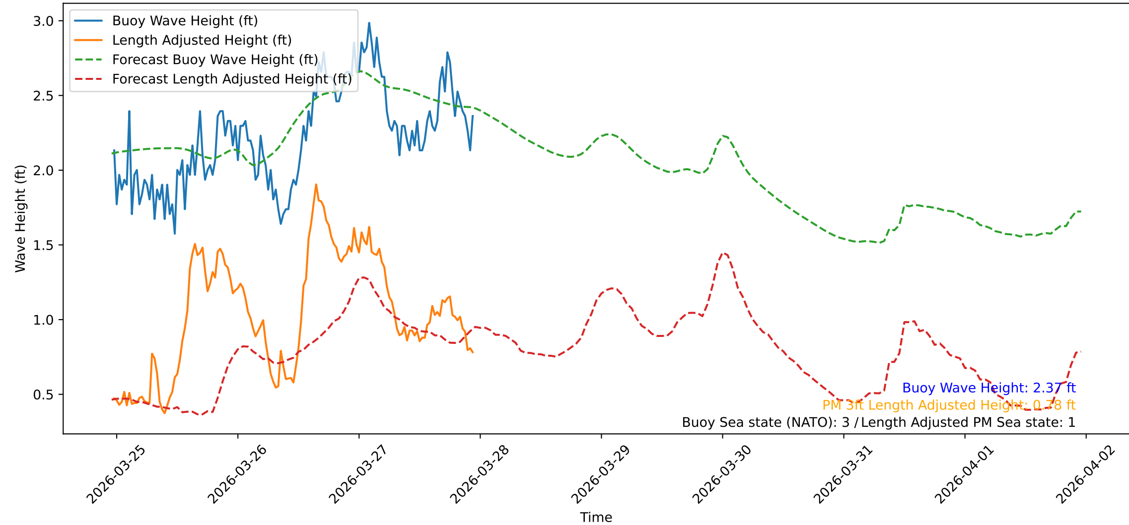
Wave Heights over Time for Red Beach at 2026-03-27 23:20:47
