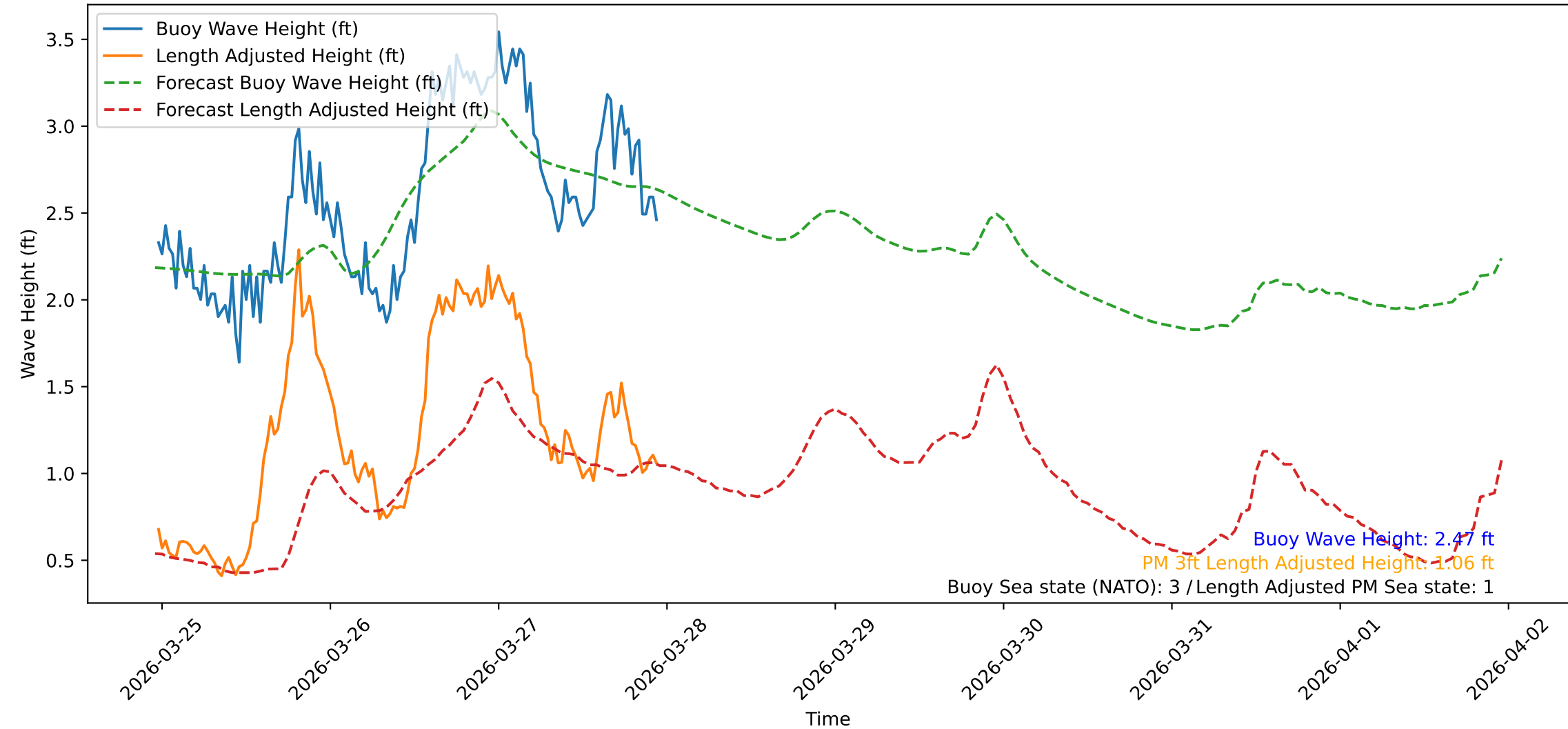
Wave Heights over Time for Green Beach at 2026-03-27 23:21:09
