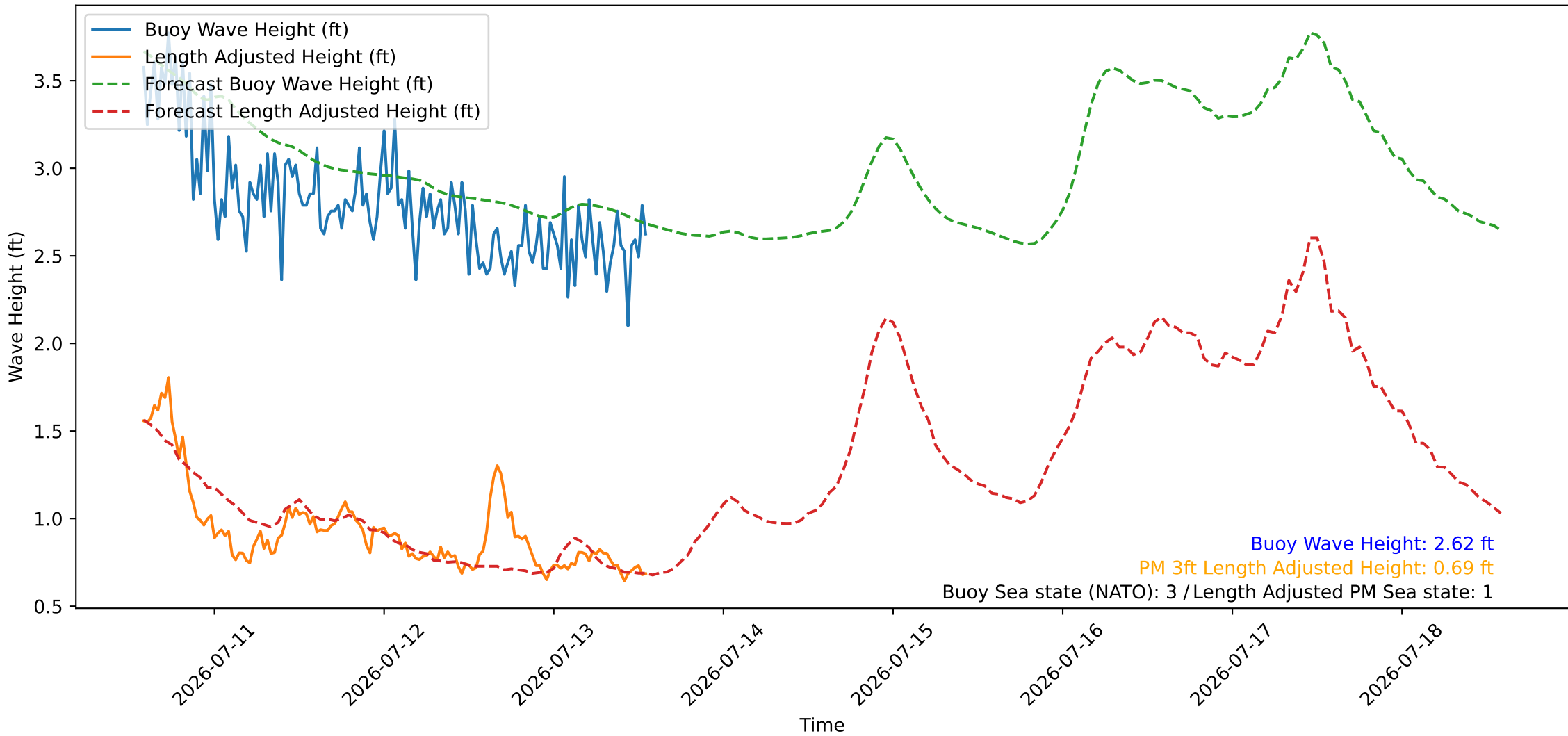
Wave Heights over Time for Oceanside Harbor at 2026-07-13 14:00:26
