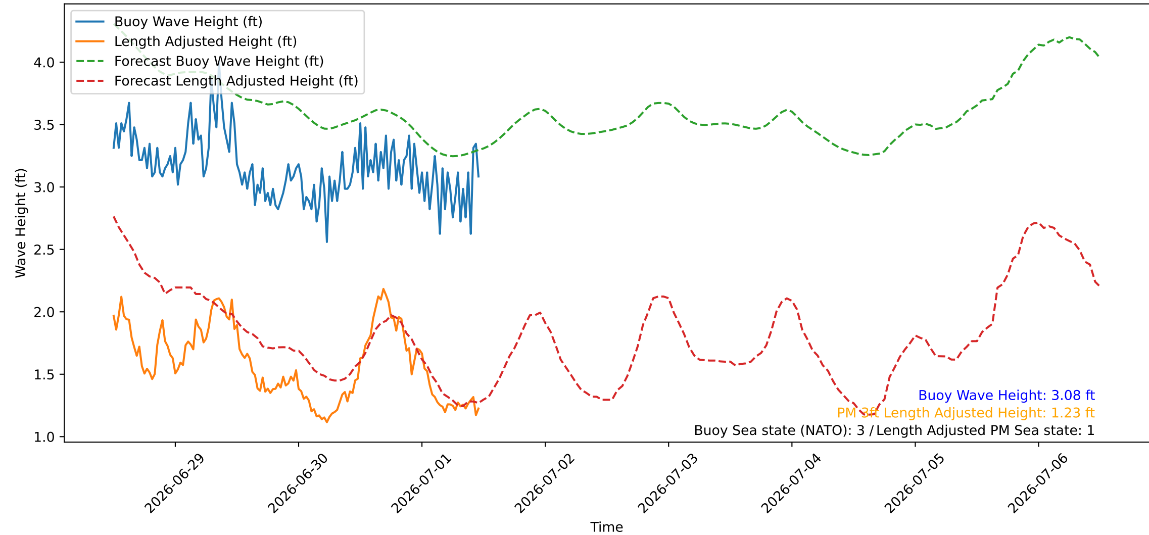
Wave Heights over Time for Oceanside Harbor at 2026-07-01 12:00:26
