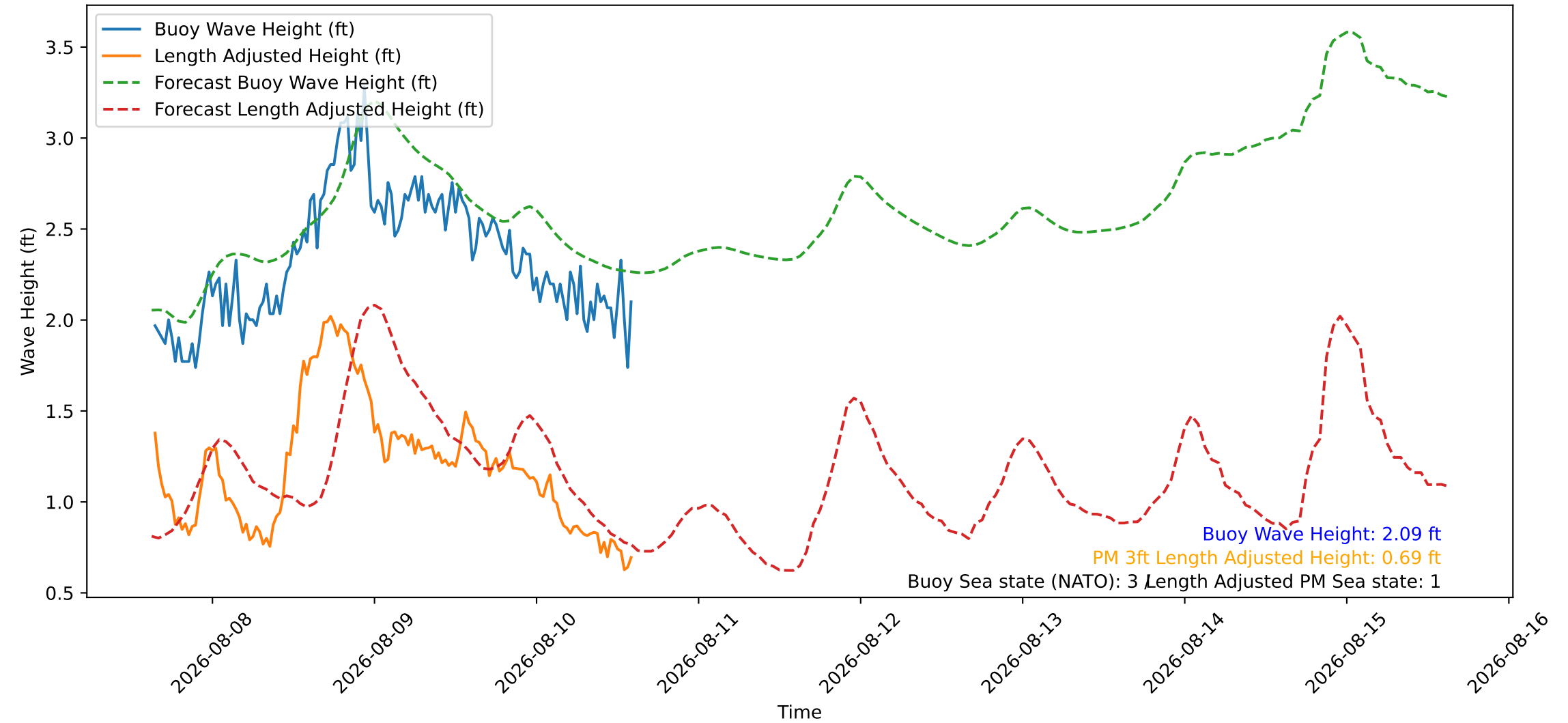
Wave Heights over Time for Red Beach at 2026-08-10 15:00:47
