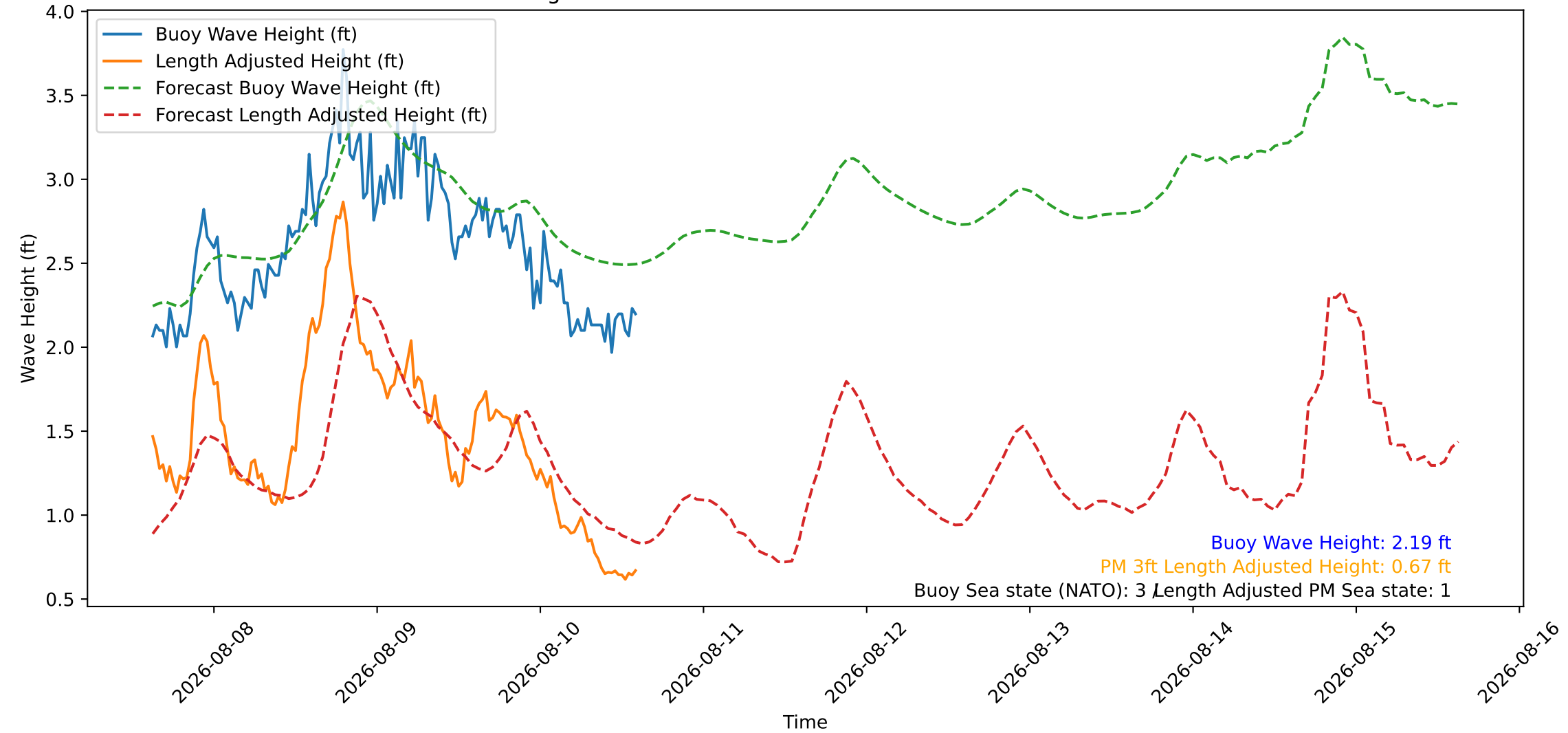
Wave Heights over Time for Green Beach at 2026-08-10 15:01:10
