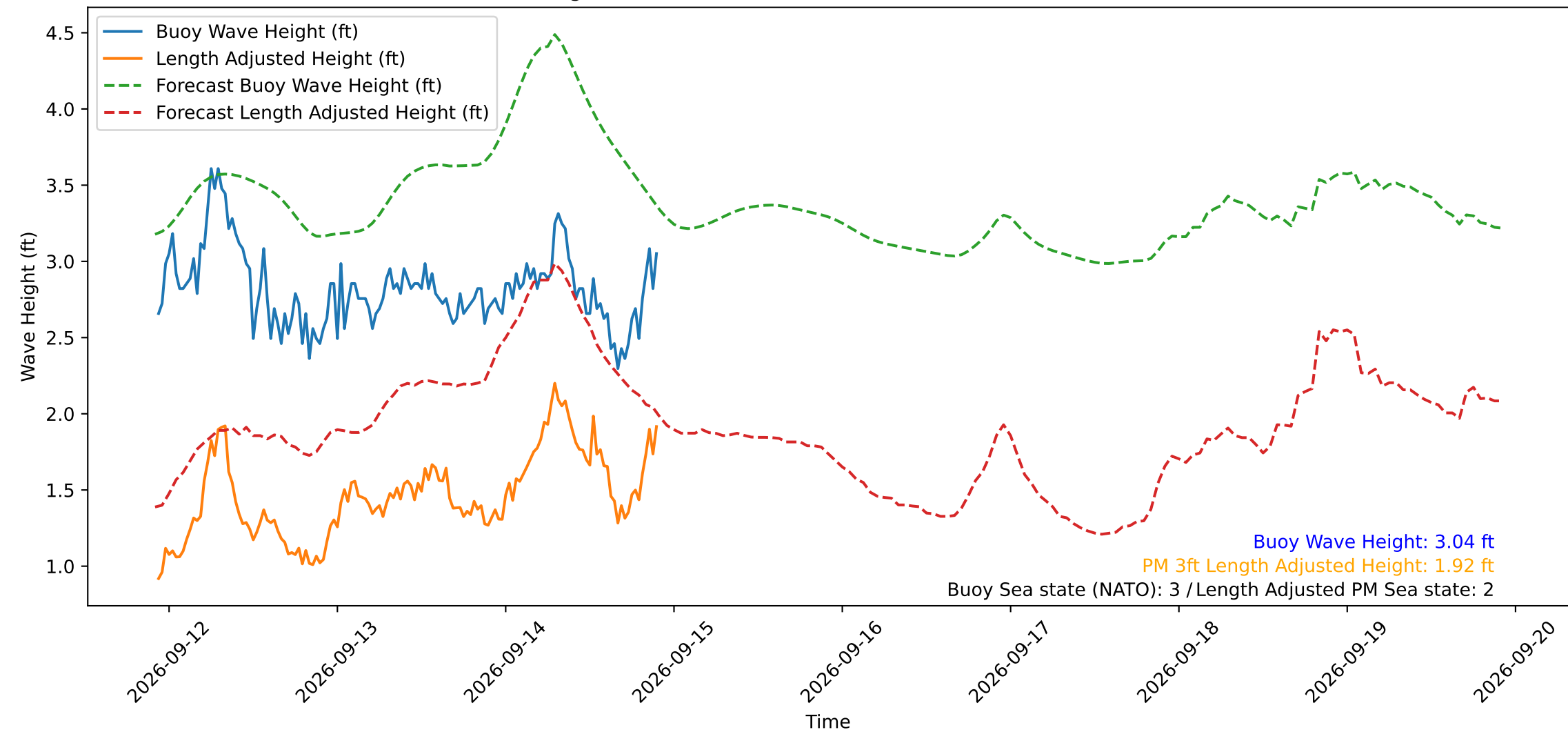
Wave Heights over Time for Green Beach at 2026-09-14 22:11:11
