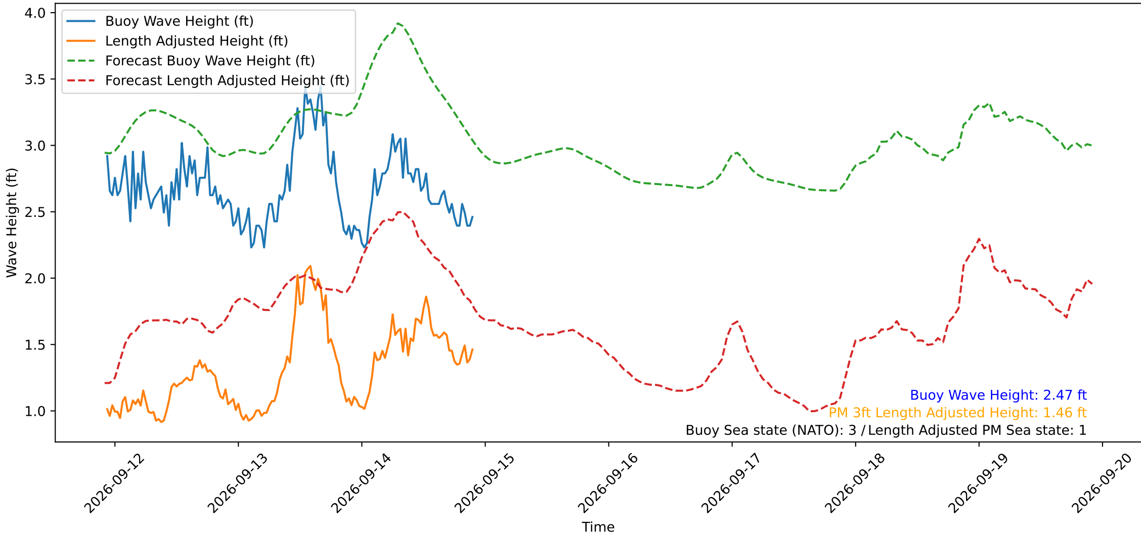
Wave Heights over Time for Red Beach at 2026-09-14 22:10:49
