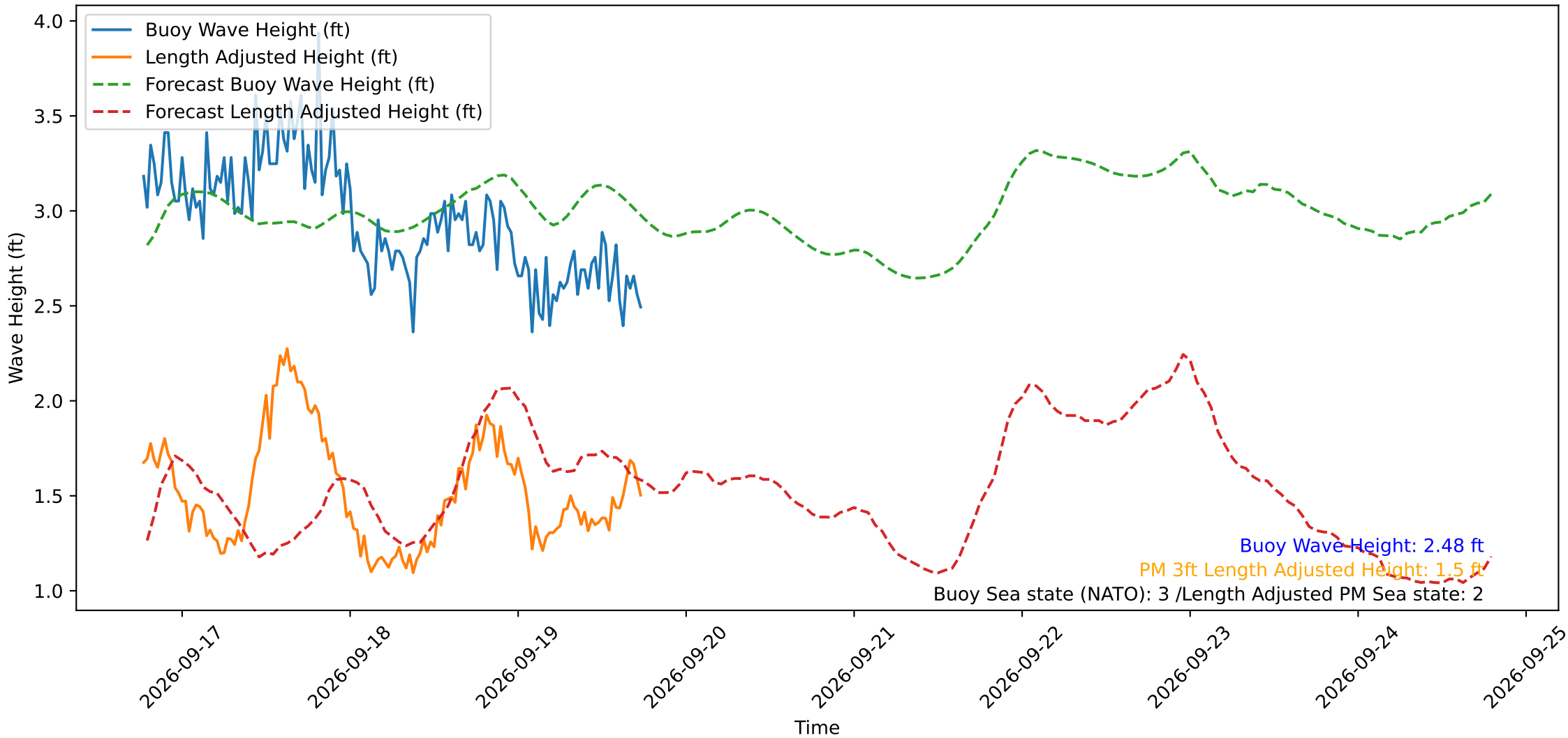
Wave Heights over Time for Oceanside Harbor at 2026-09-19 18:30:29
