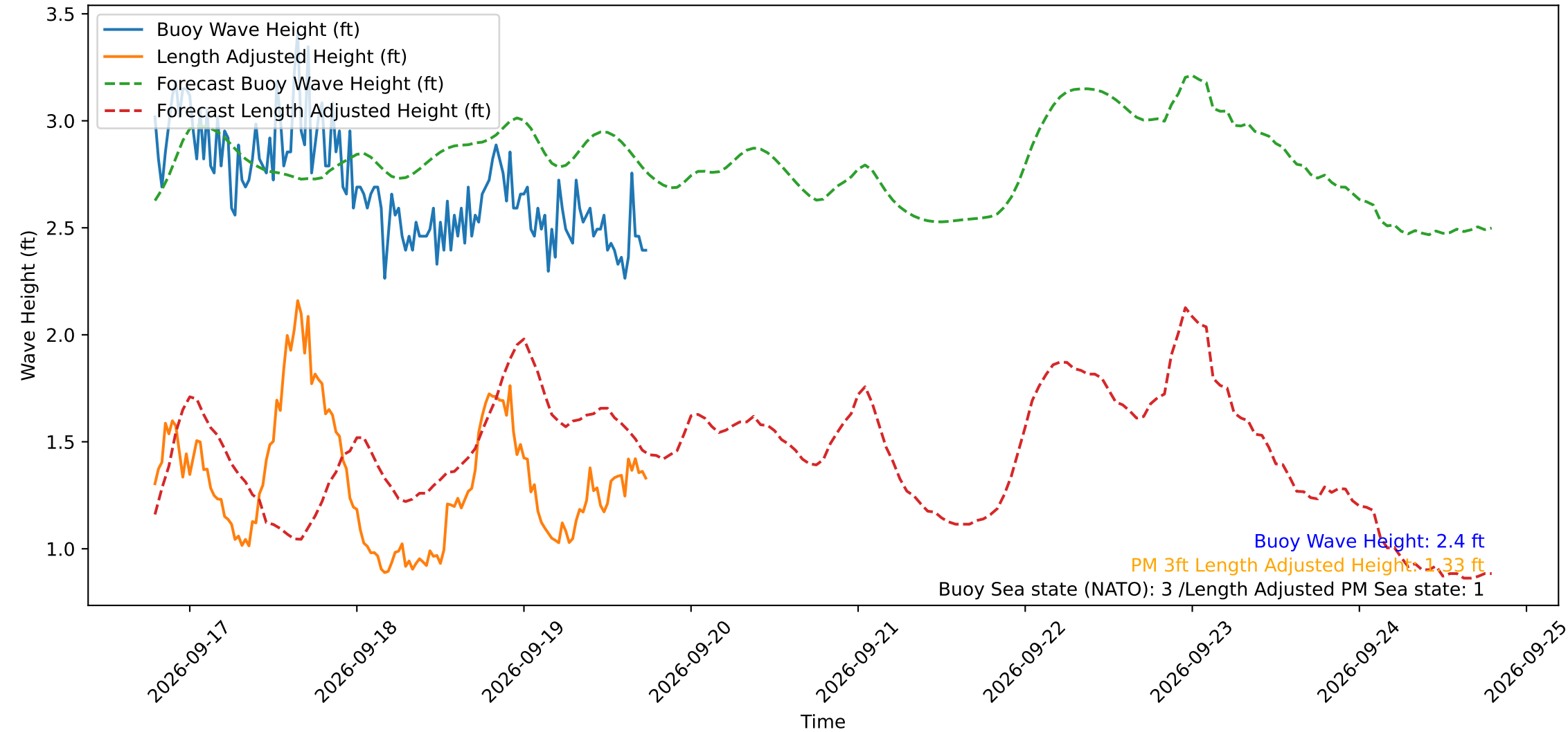
Wave Heights over Time for Red Beach at 2026-09-19 18:30:49
