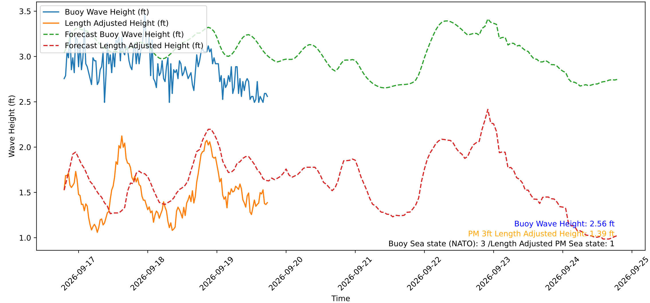
Wave Heights over Time for Green Beach at 2026-09-19 18:31:11
