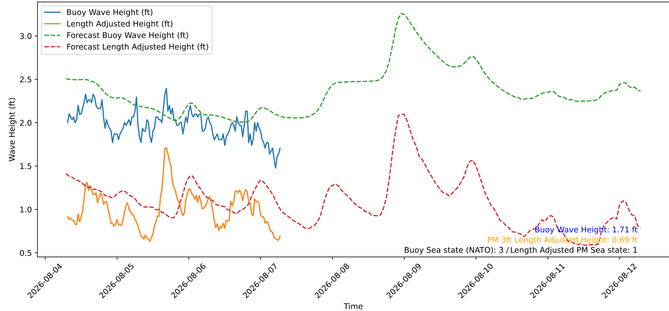
Wave Heights over Time for Red Beach at 2026-08-07 07:10:45
