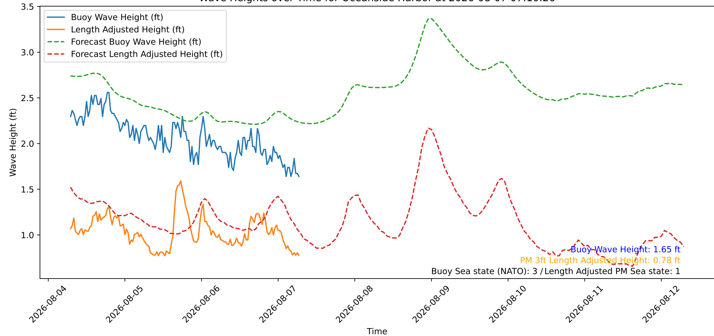
Wave Heights over Time for Oceanside Harbor at 2026-08-07 07:10:26
