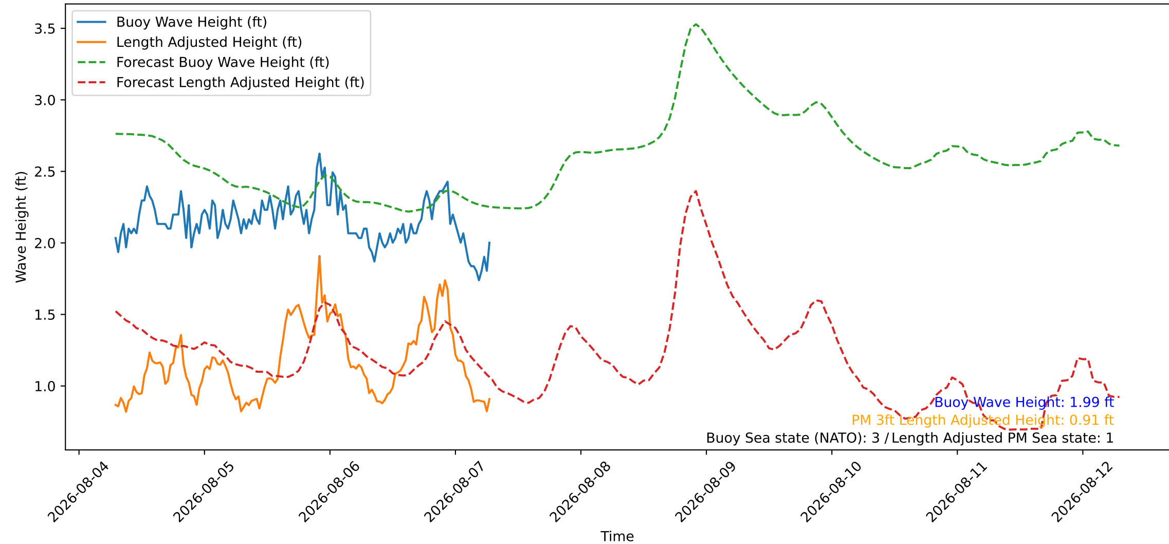
Wave Heights over Time for Green Beach at 2026-08-07 07:11:08
