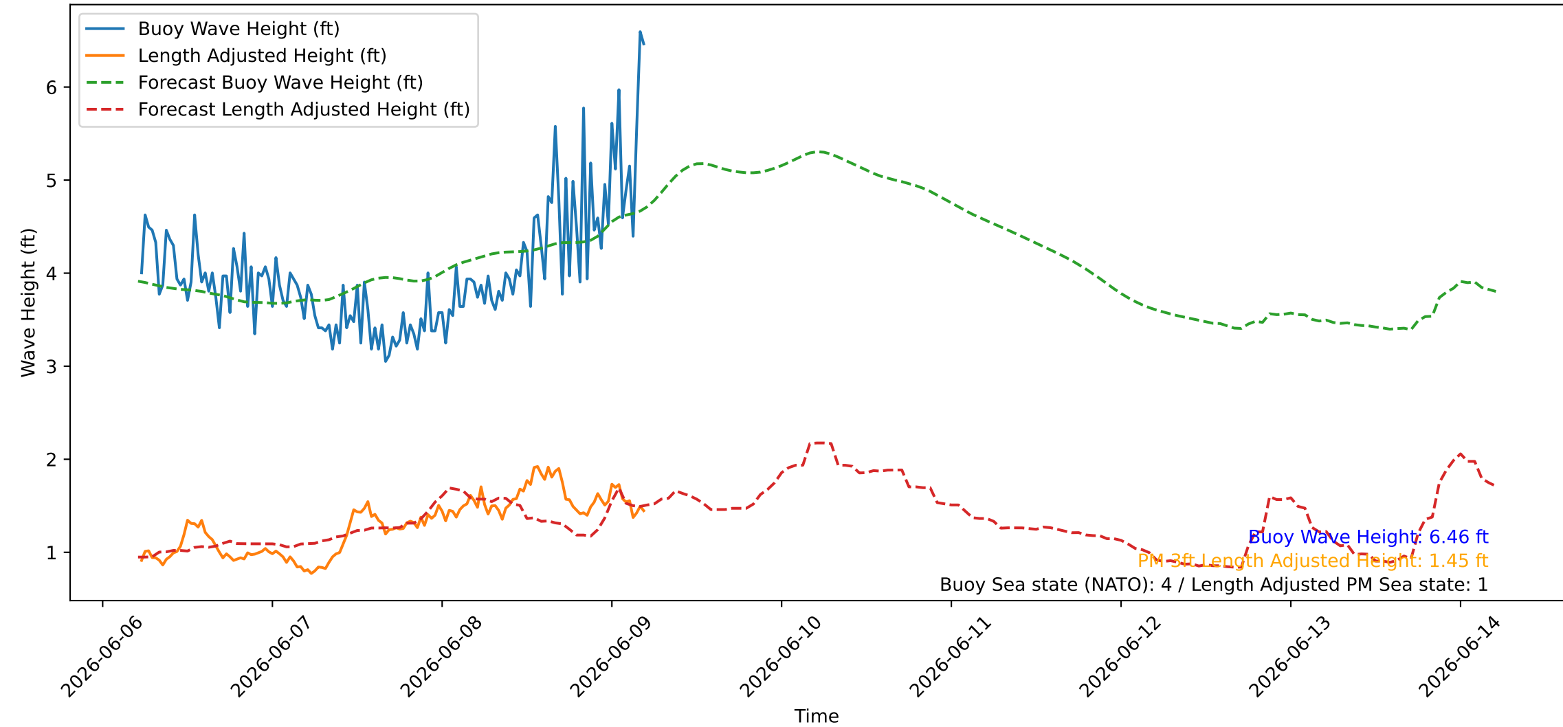
Wave Heights over Time for Red Beach at 2026-06-09 05:20:46
