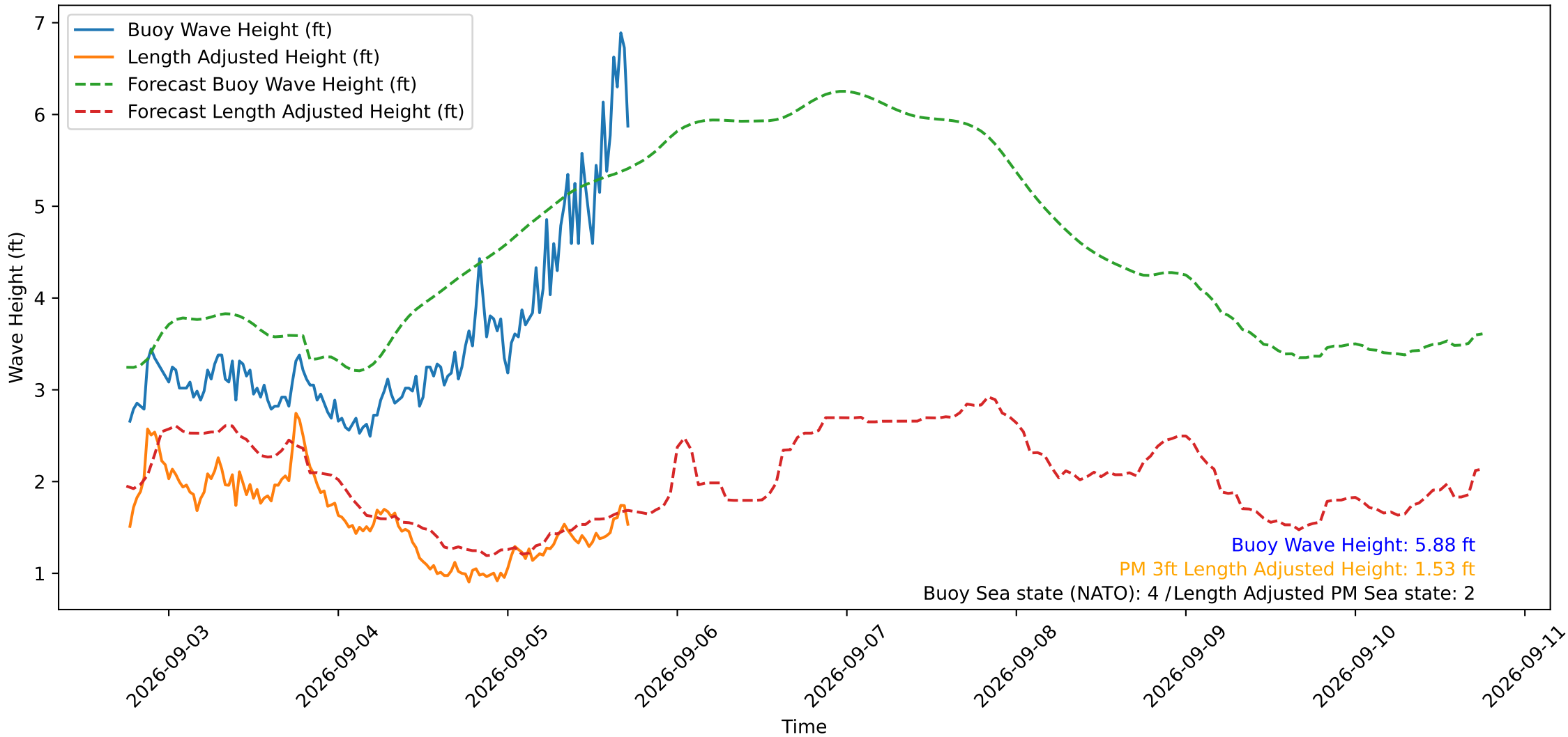
Wave Heights over Time for Green Beach at 2026-09-05 18:01:13
