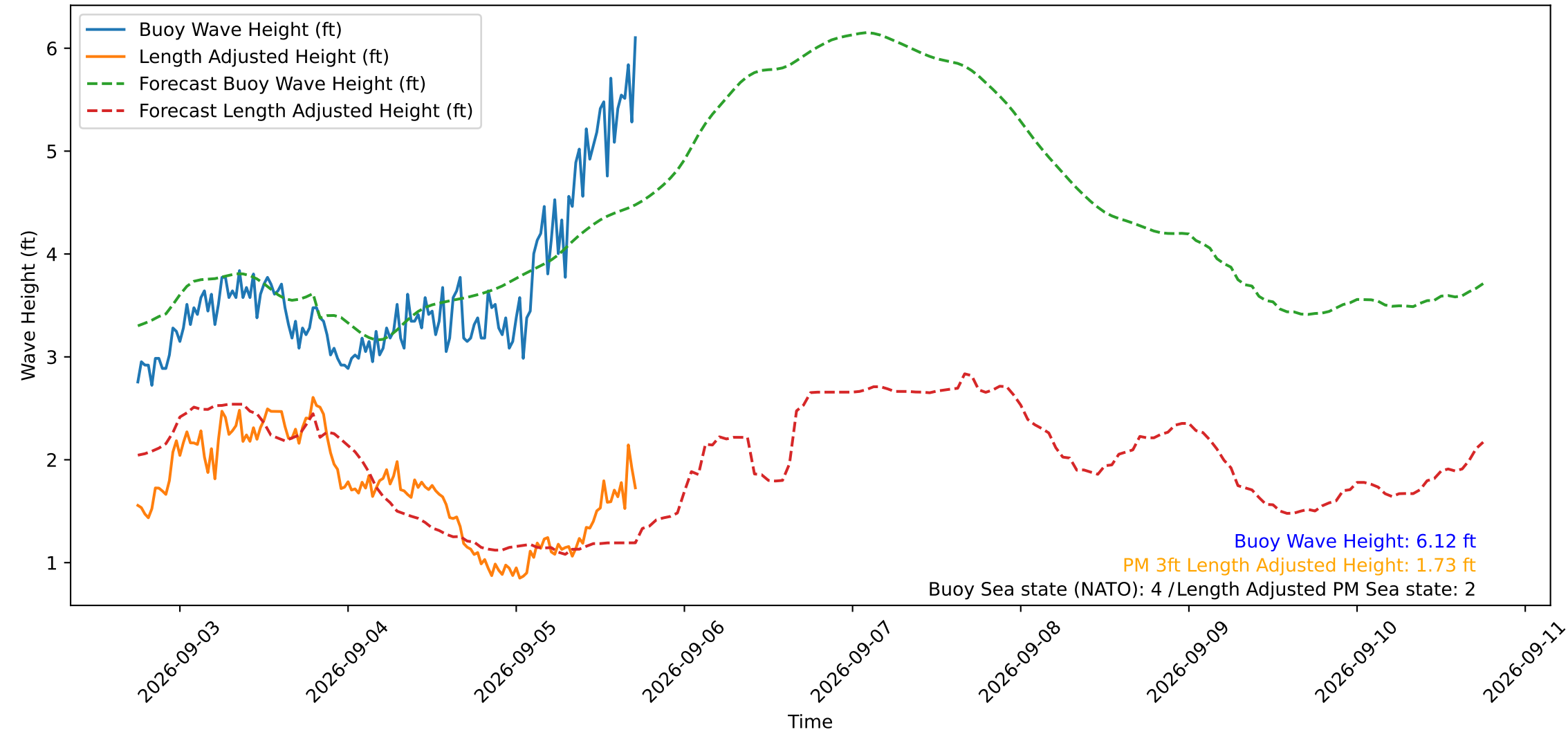
Wave Heights over Time for Oceanside Harbor at 2026-09-05 18:00:30
