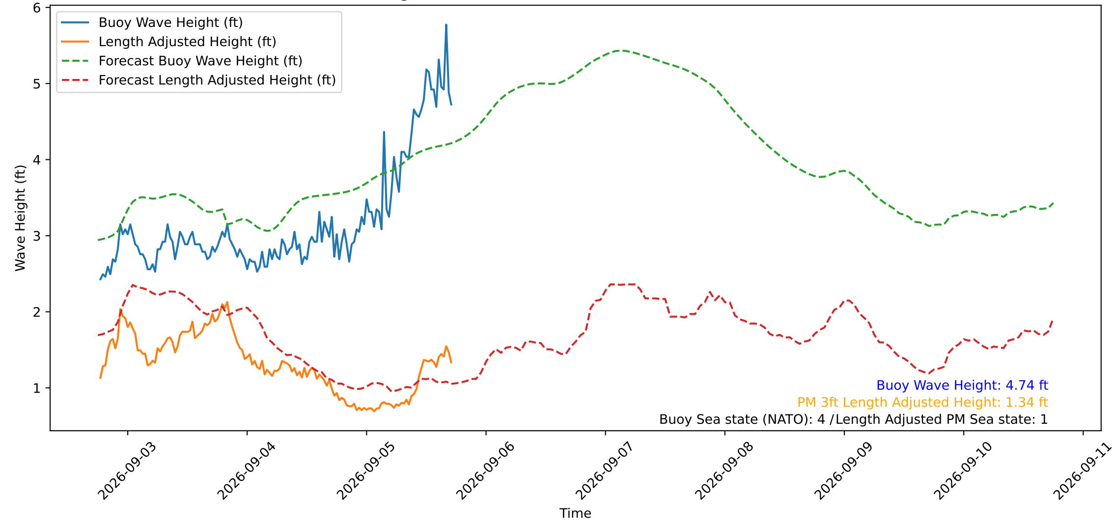
Wave Heights over Time for Red Beach at 2026-09-05 18:00:50
