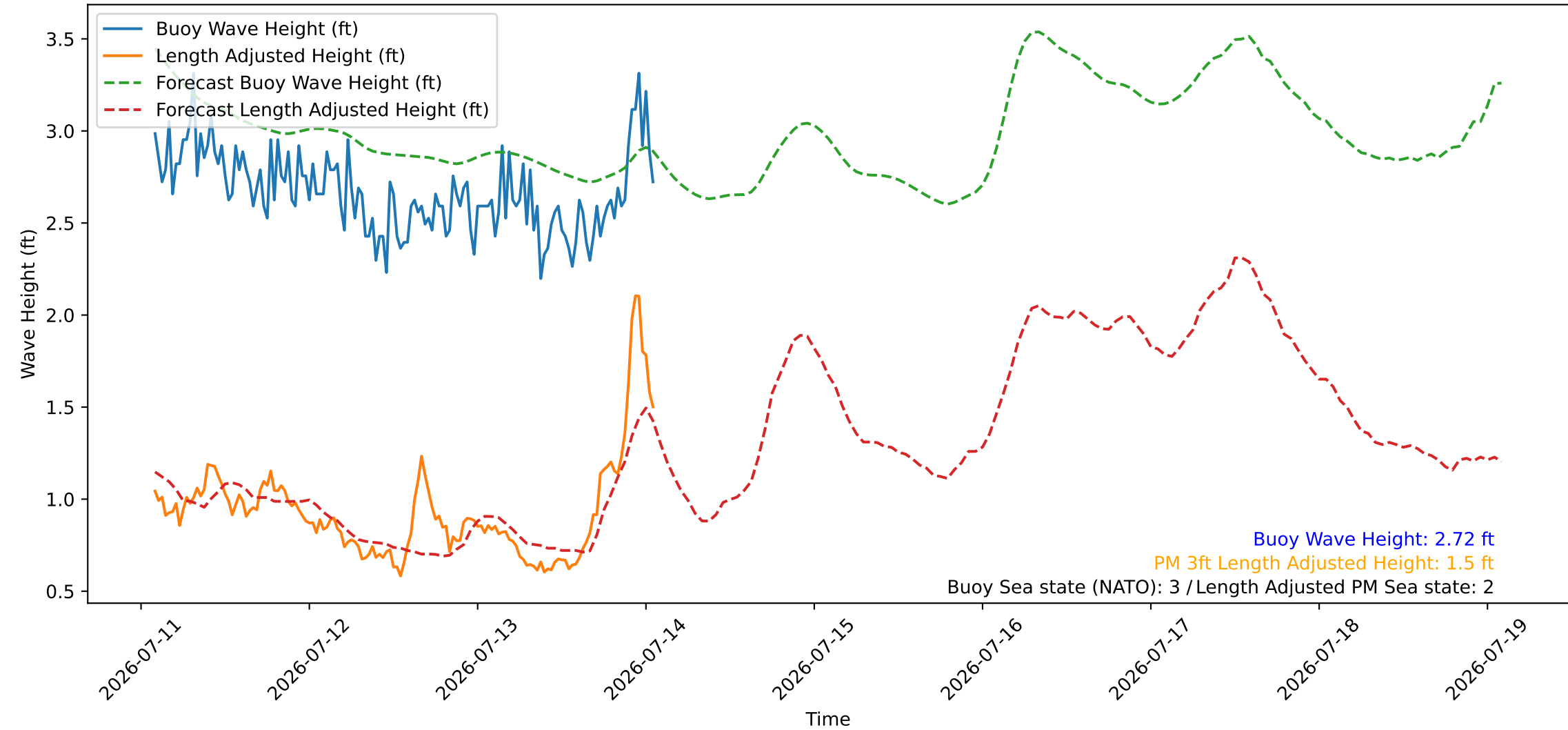
Wave Heights over Time for Green Beach at 2026-07-14 02:01:08
