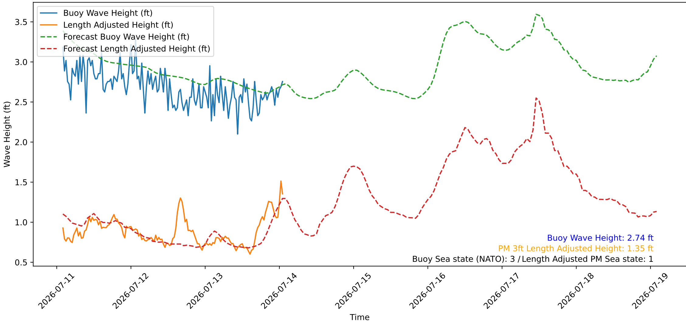
Wave Heights over Time for Oceanside Harbor at 2026-07-14 02:00:26
