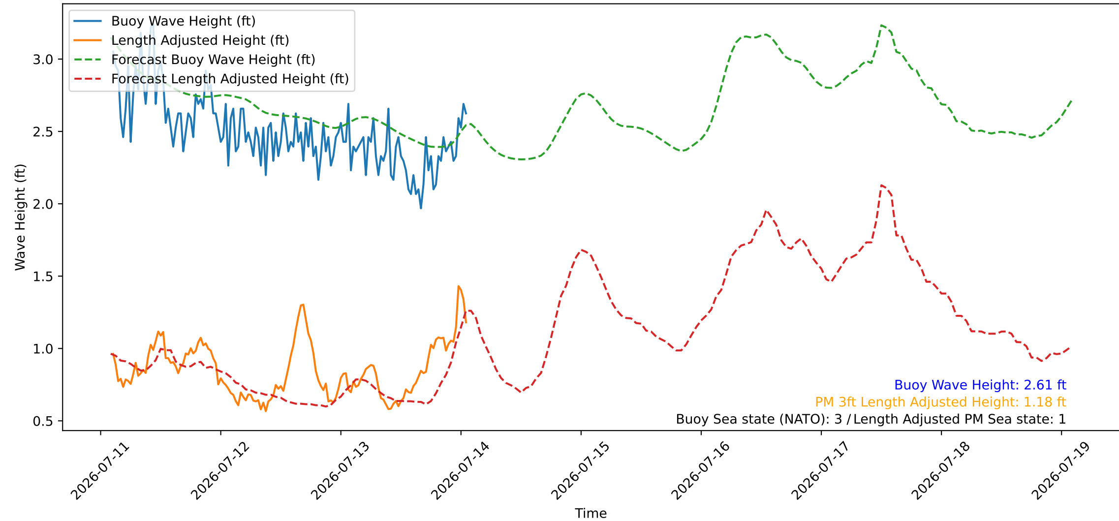
Wave Heights over Time for Red Beach at 2026-07-14 02:00:46
