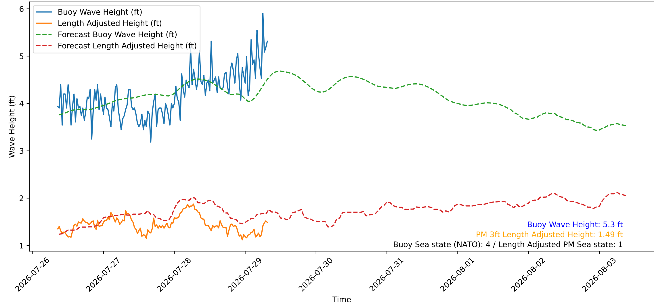
Wave Heights over Time for Oceanside Harbor at 2026-07-29 08:30:26
