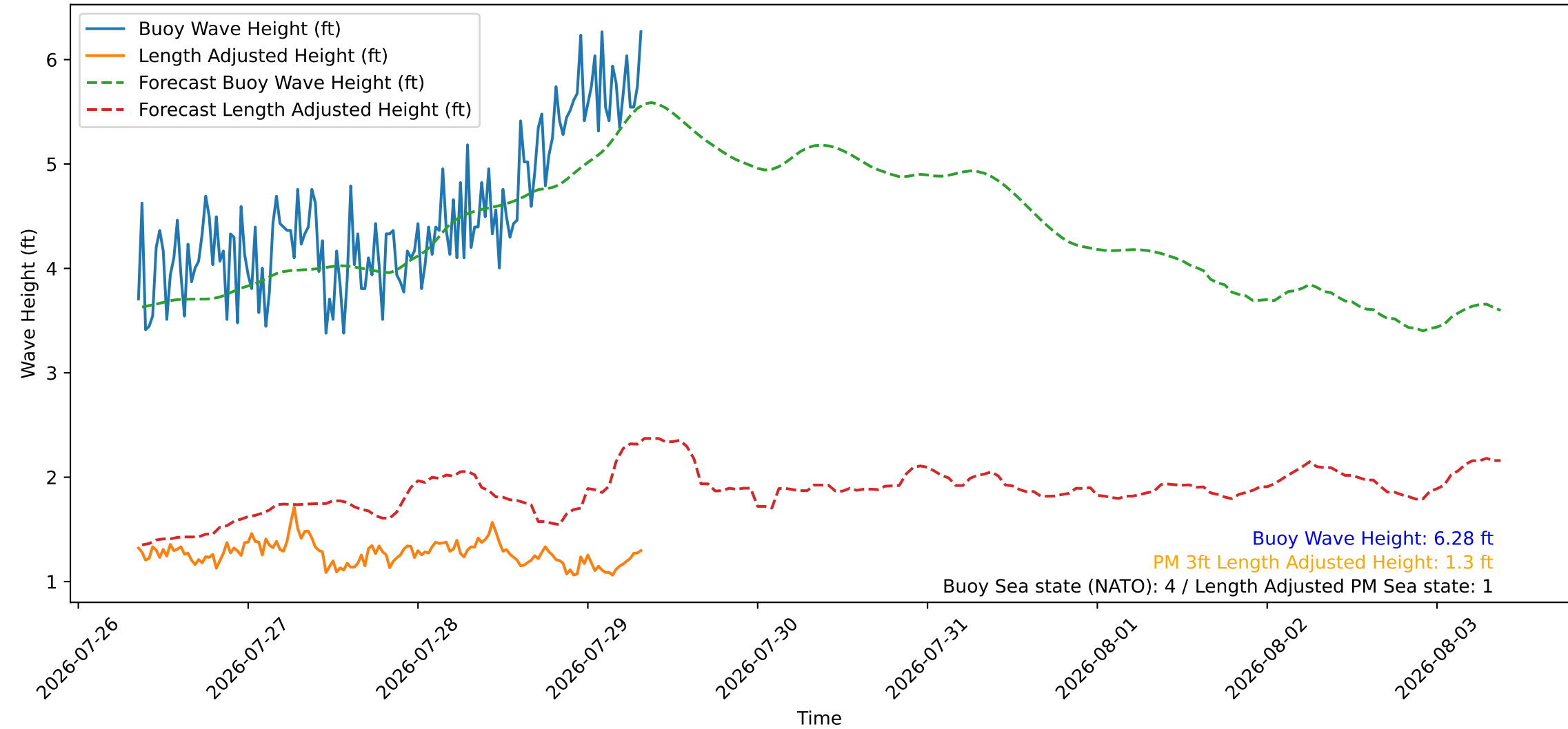
Wave Heights over Time for Green Beach at 2026-07-29 08:31:08
