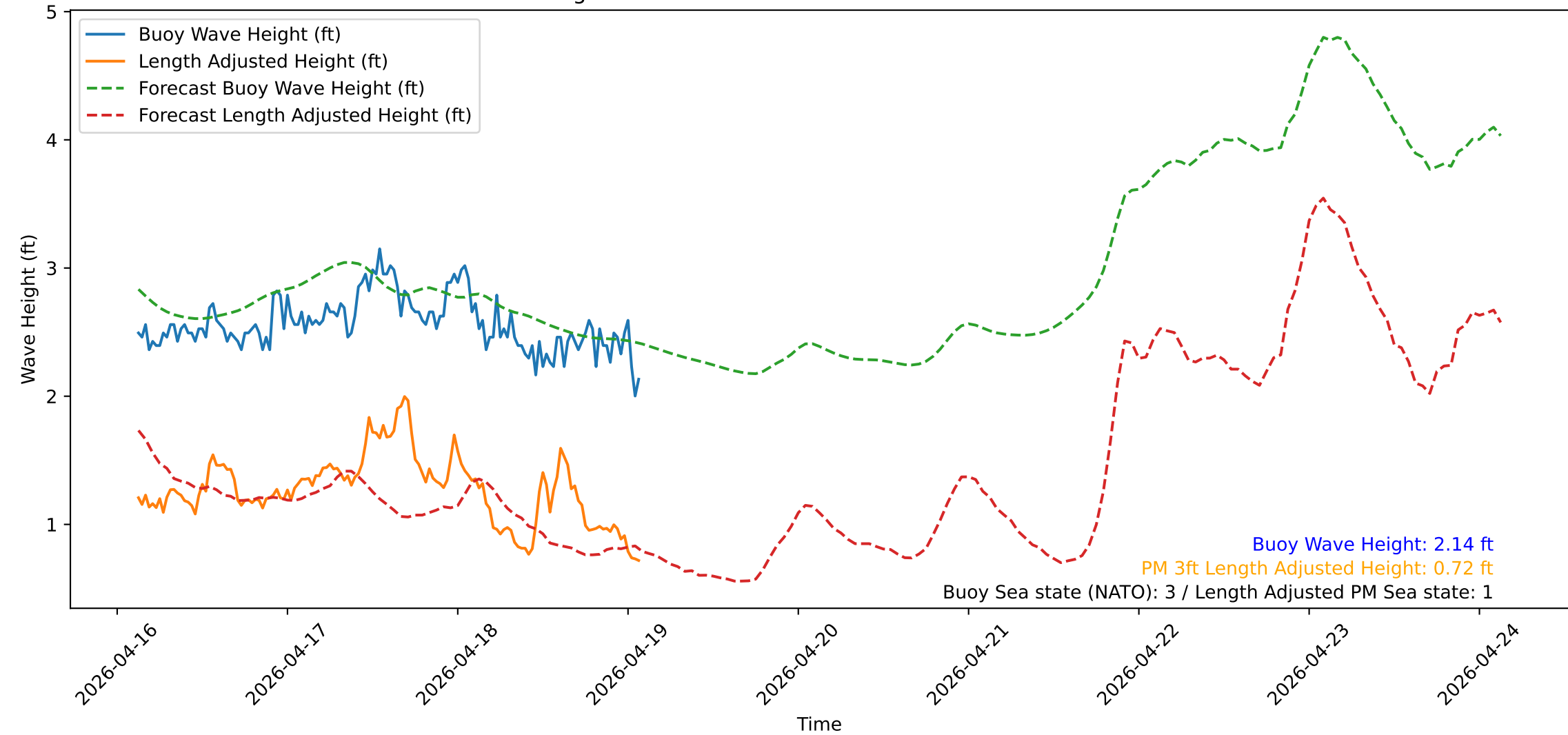
Wave Heights over Time for Red Beach at 2026-04-19 02:30:50
