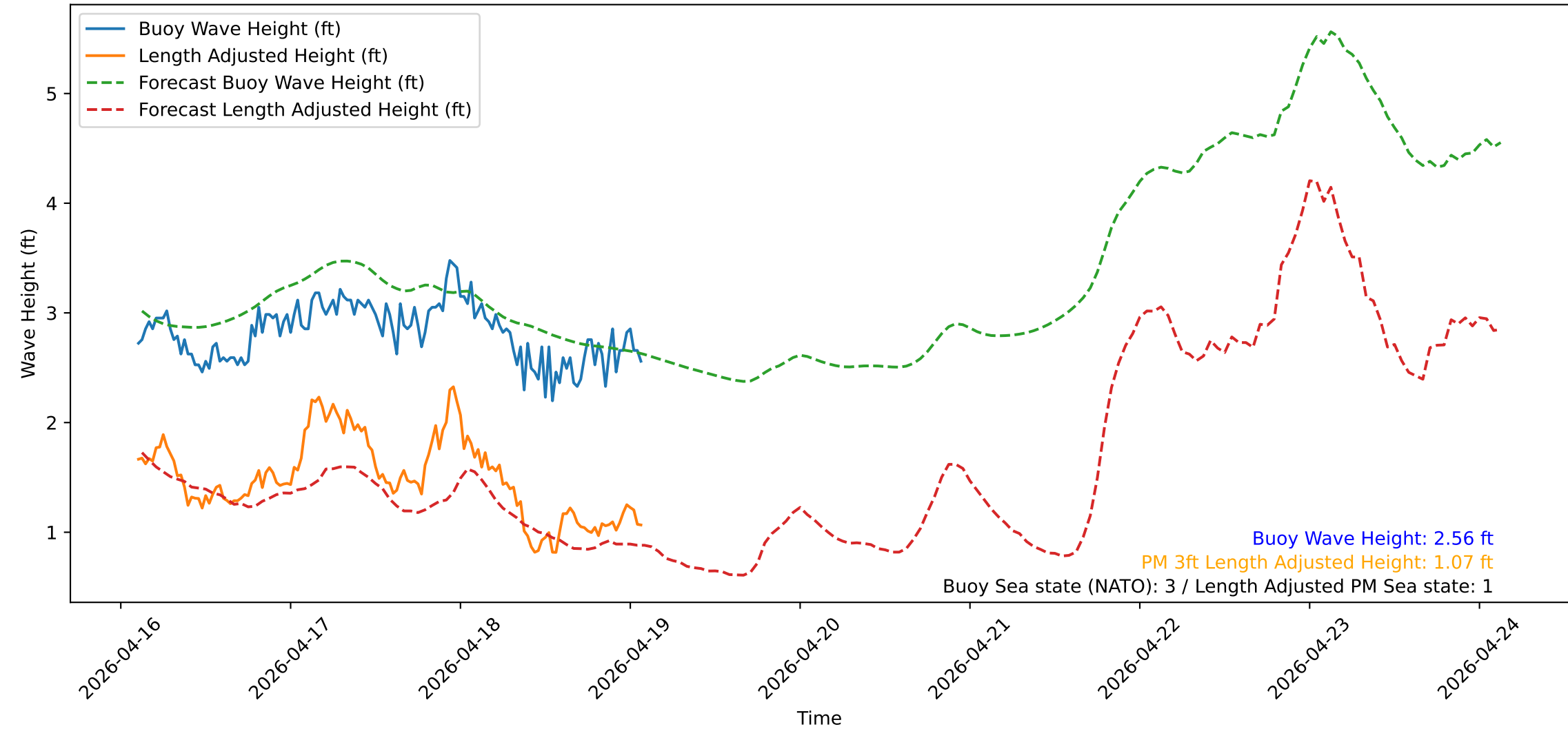
Wave Heights over Time for Green Beach at 2026-04-19 02:31:12
