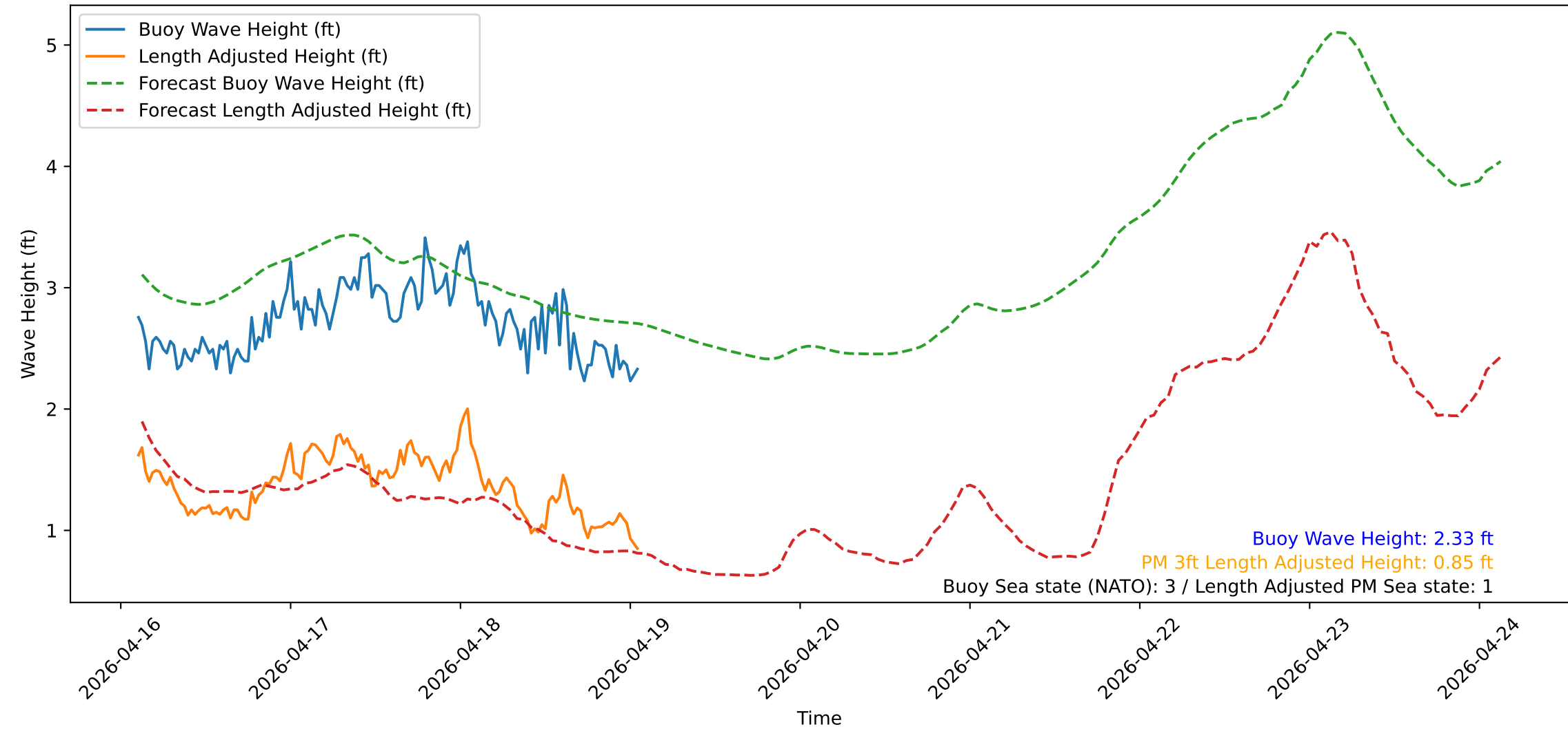
Wave Heights over Time for Oceanside Harbor at 2026-04-19 02:30:31
