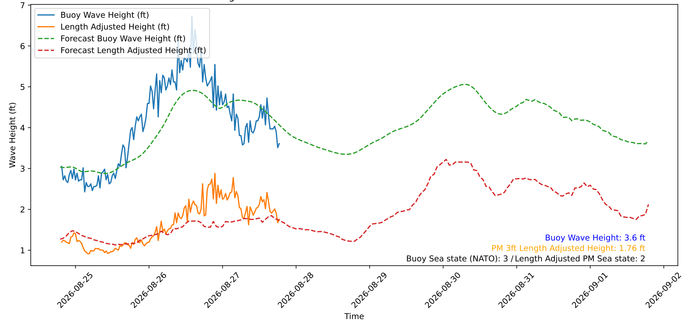
Wave Heights over Time for Oceanside Harbor at 2026-08-27 19:20:30
