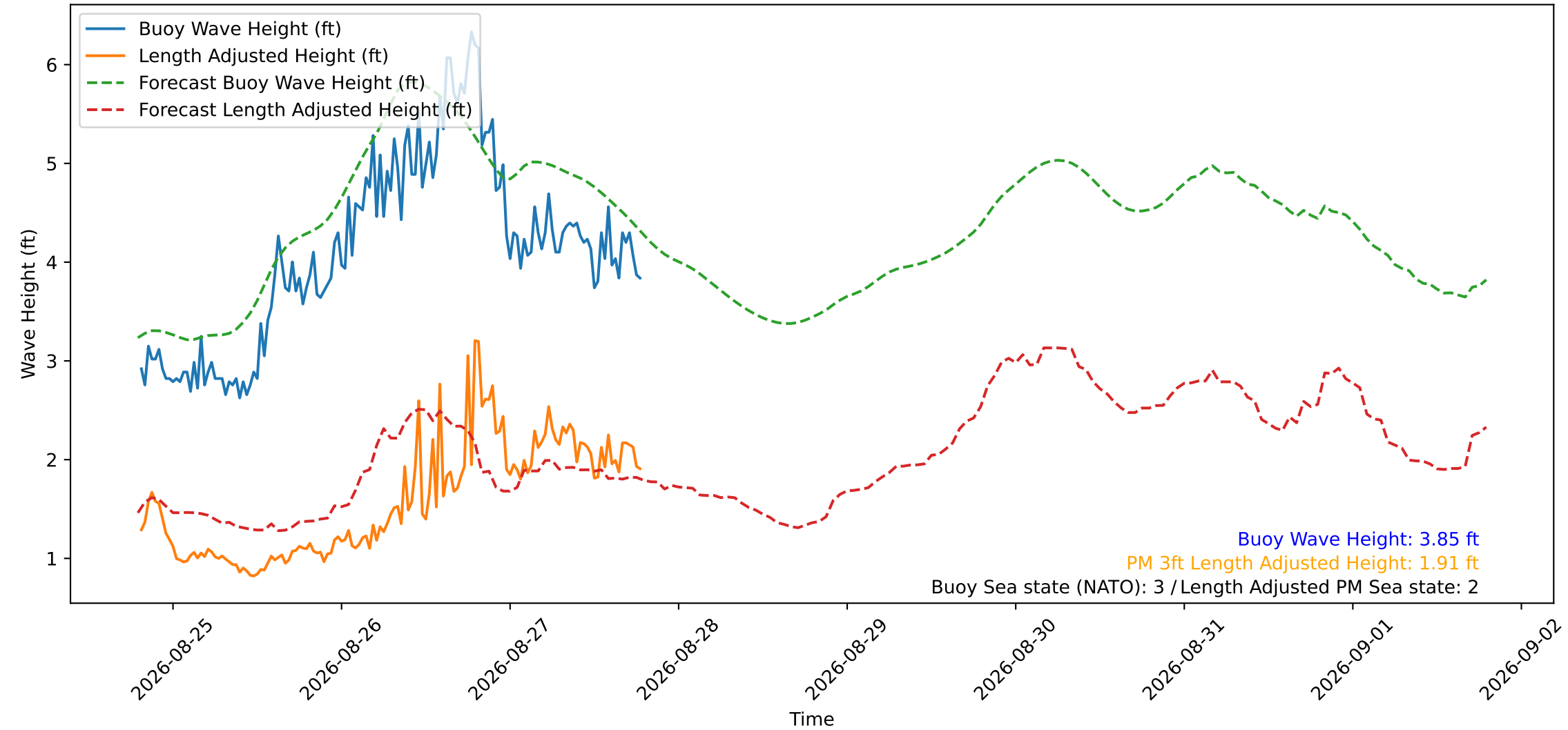
Wave Heights over Time for Green Beach at 2026-08-27 19:21:14
