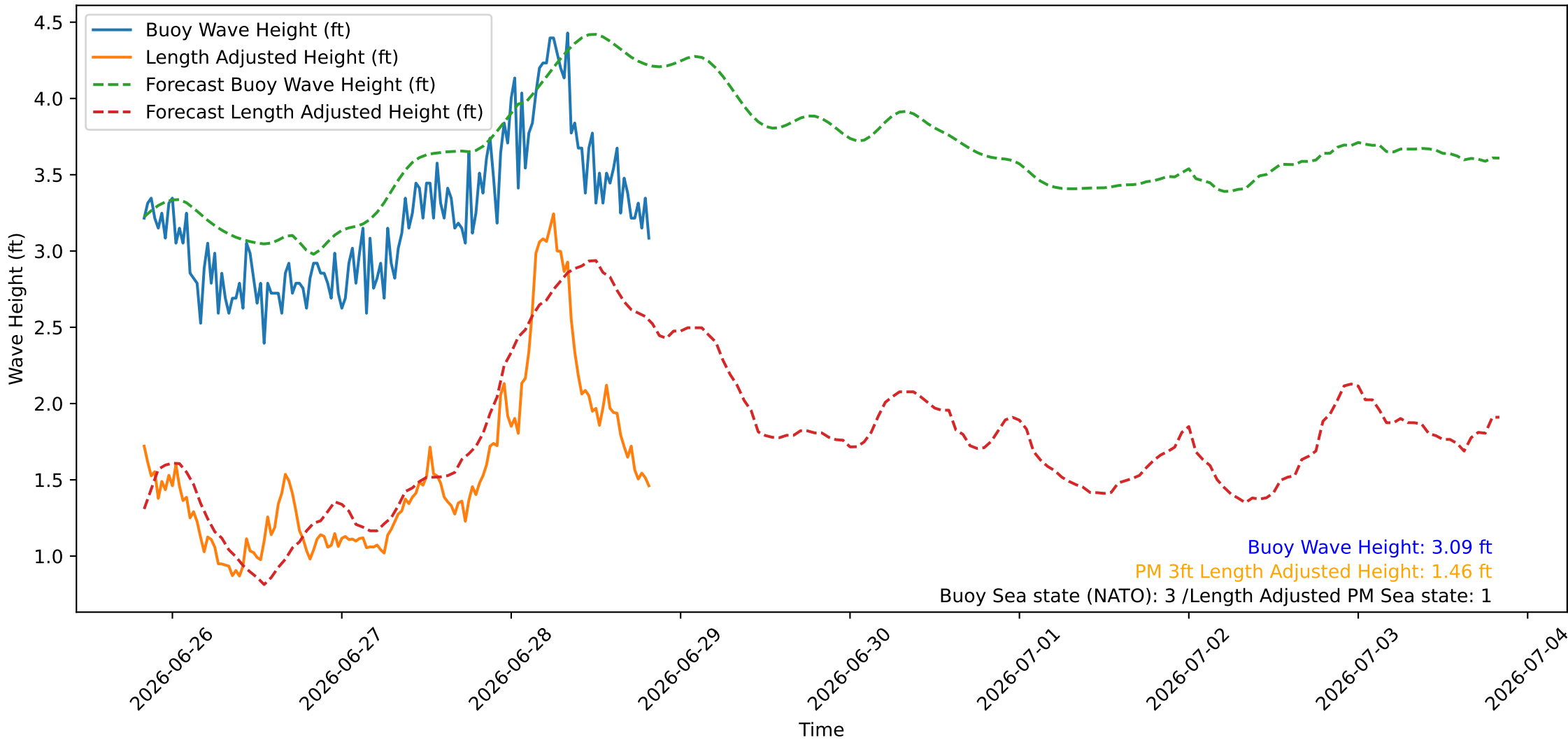
Wave Heights over Time for Oceanside Harbor at 2026-06-28 20:00:26
