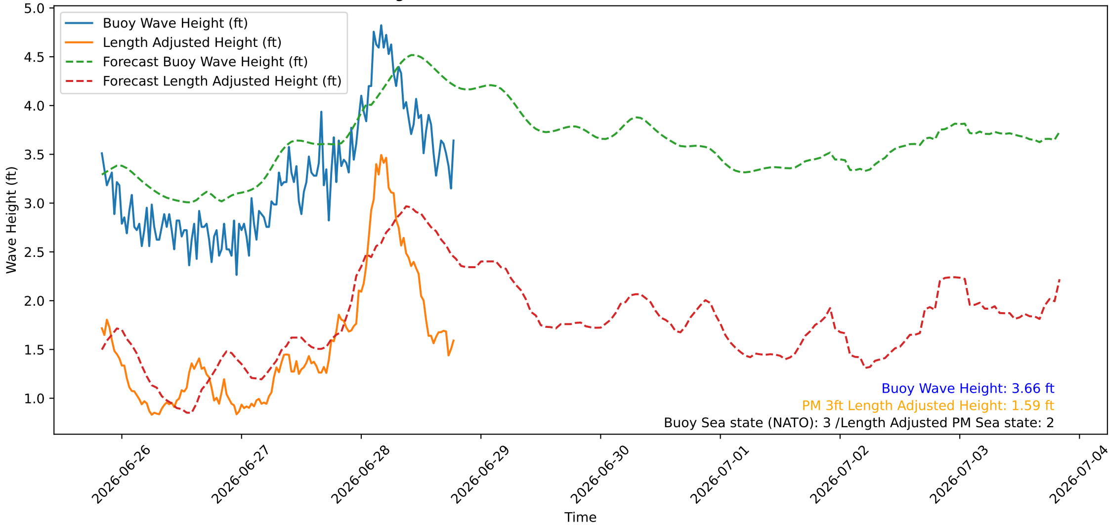
Wave Heights over Time for Green Beach at 2026-06-28 20:01:08
