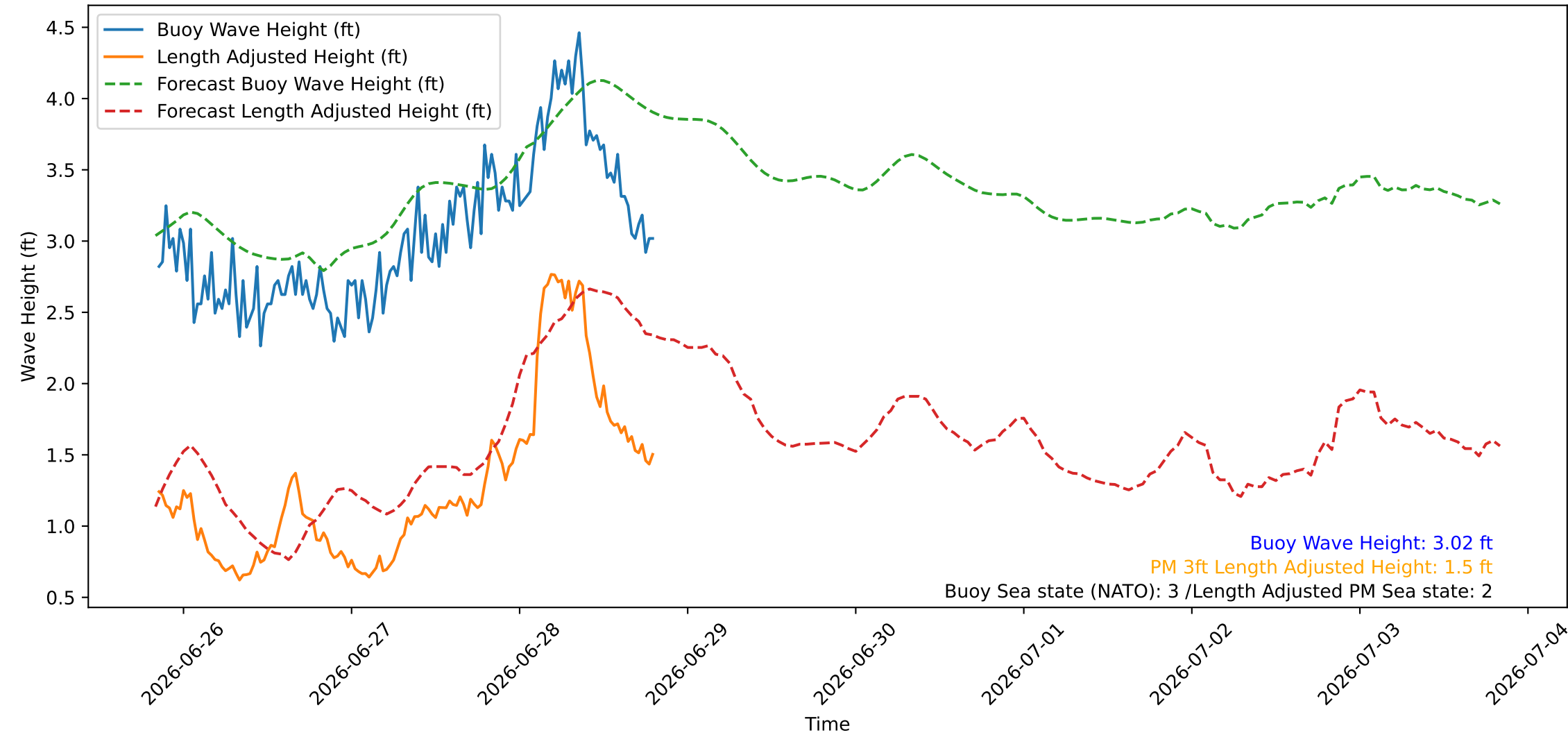
Wave Heights over Time for Red Beach at 2026-06-28 20:00:45
