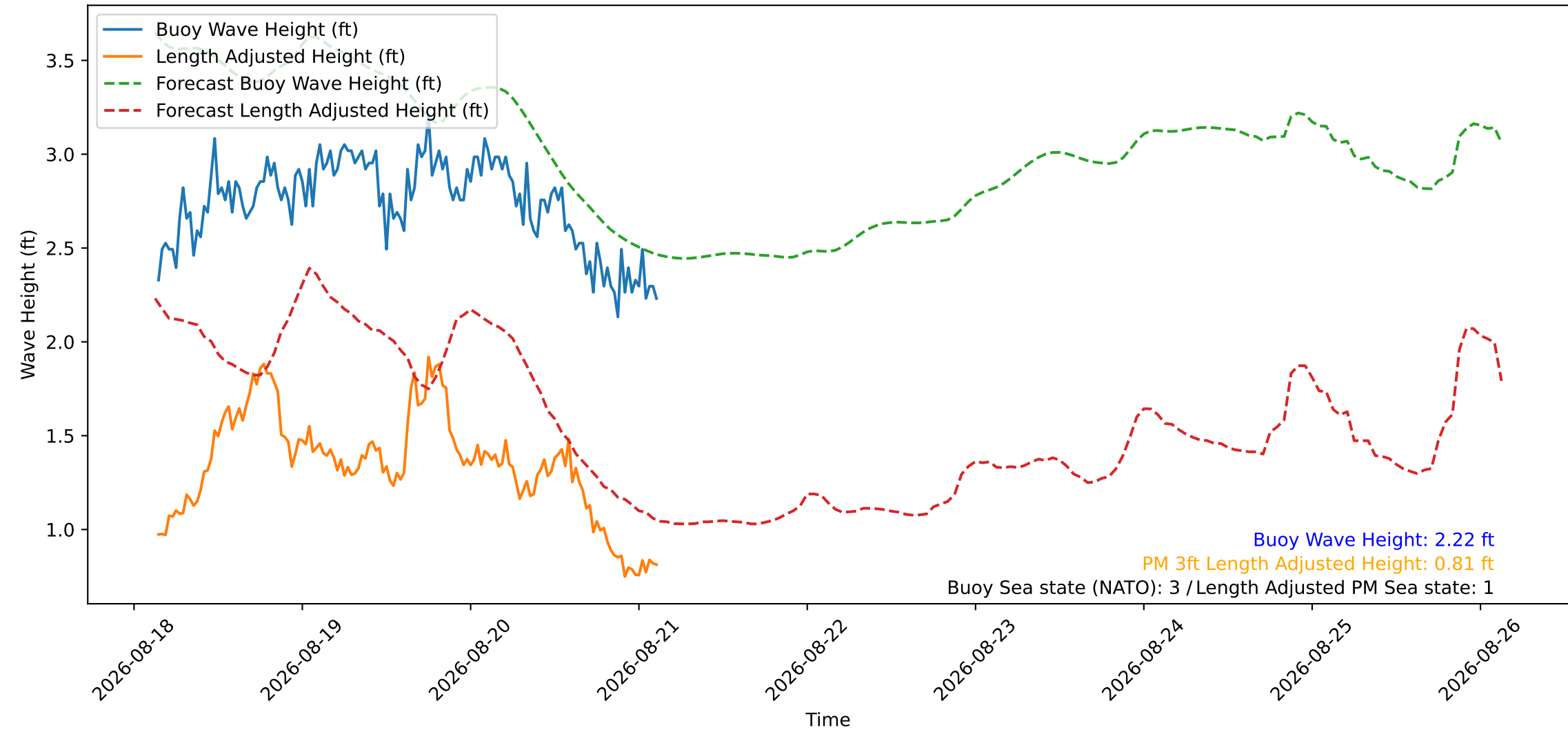
Wave Heights over Time for Red Beach at 2026-08-21 03:10:46
