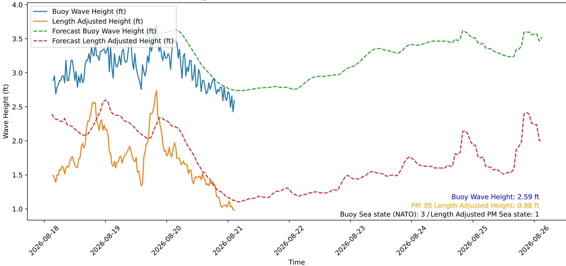
Wave Heights over Time for Green Beach at 2026-08-21 03:11:08
