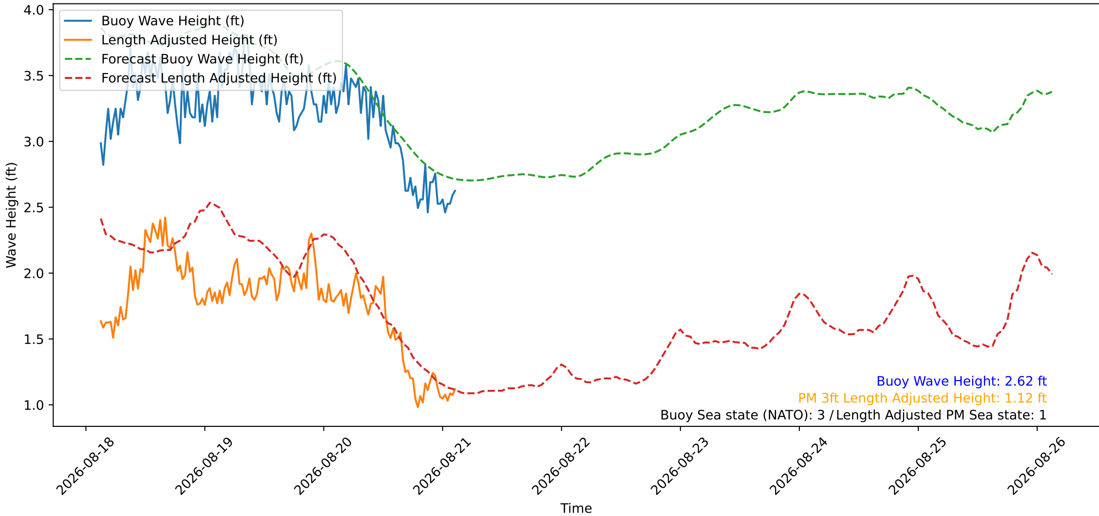
Wave Heights over Time for Oceanside Harbor at 2026-08-21 03:10:26
