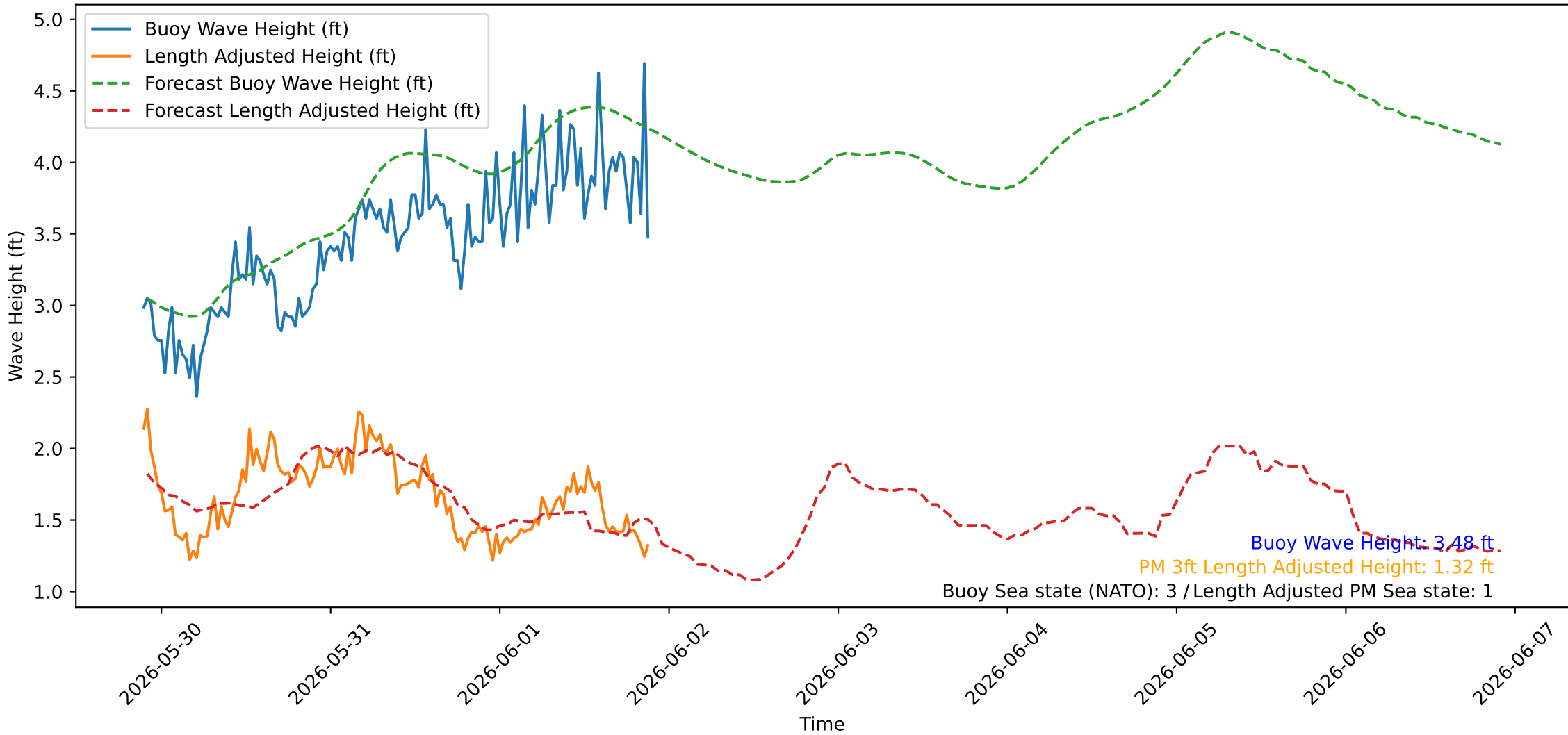
Wave Heights over Time for Oceanside Harbor at 2026-06-01 21:30:26
