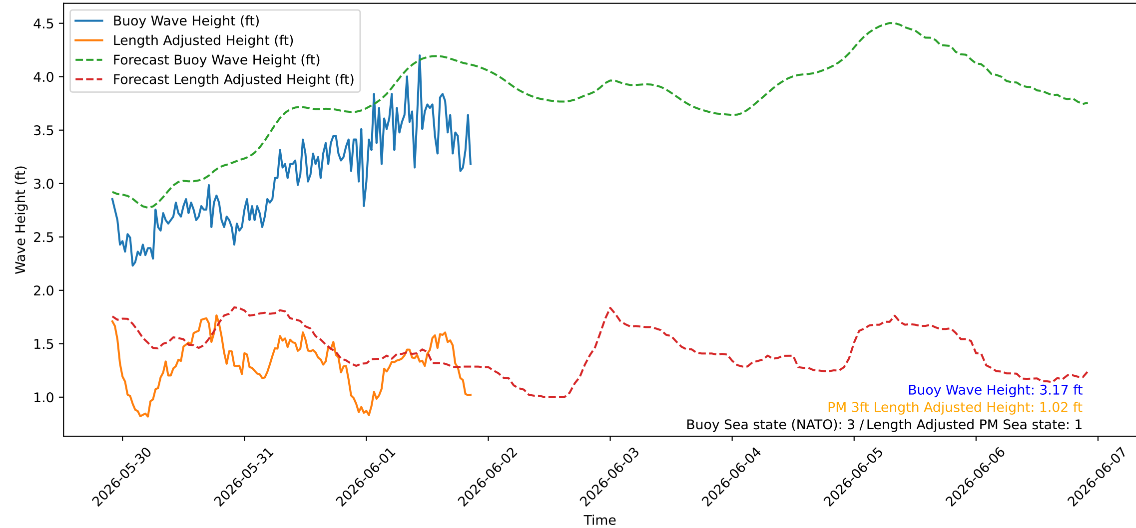
Wave Heights over Time for Red Beach at 2026-06-01 21:30:46
