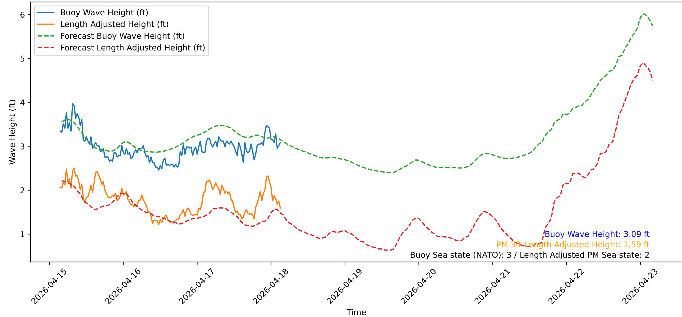
Wave Heights over Time for Green Beach at 2026-04-18 03:41:13
