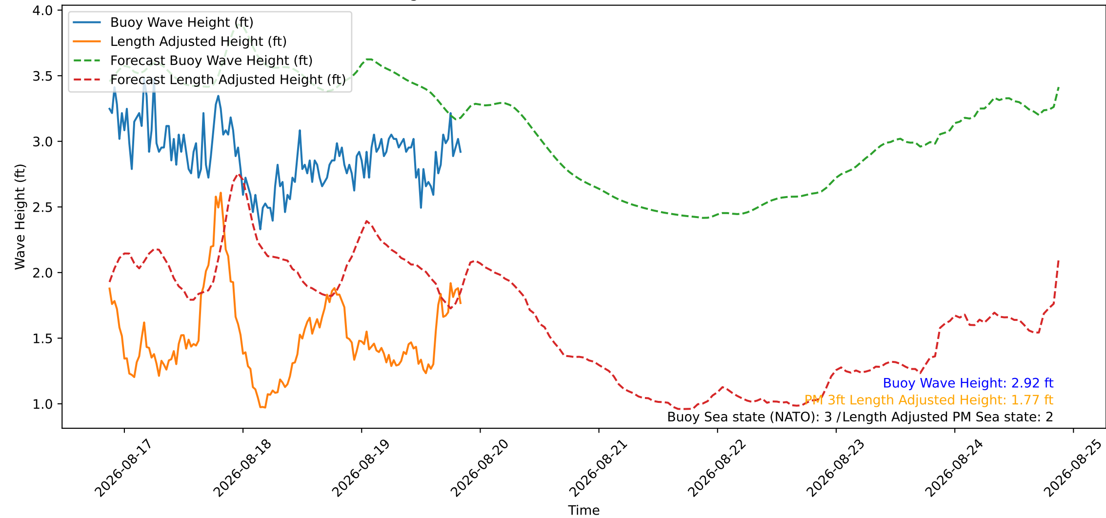
Wave Heights over Time for Red Beach at 2026-08-19 20:50:47
