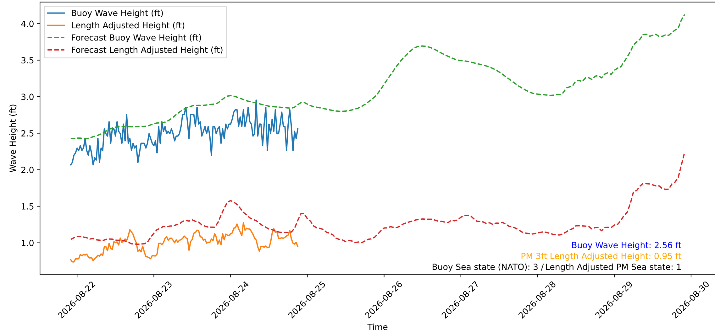
Wave Heights over Time for Red Beach at 2026-08-24 21:40:49
