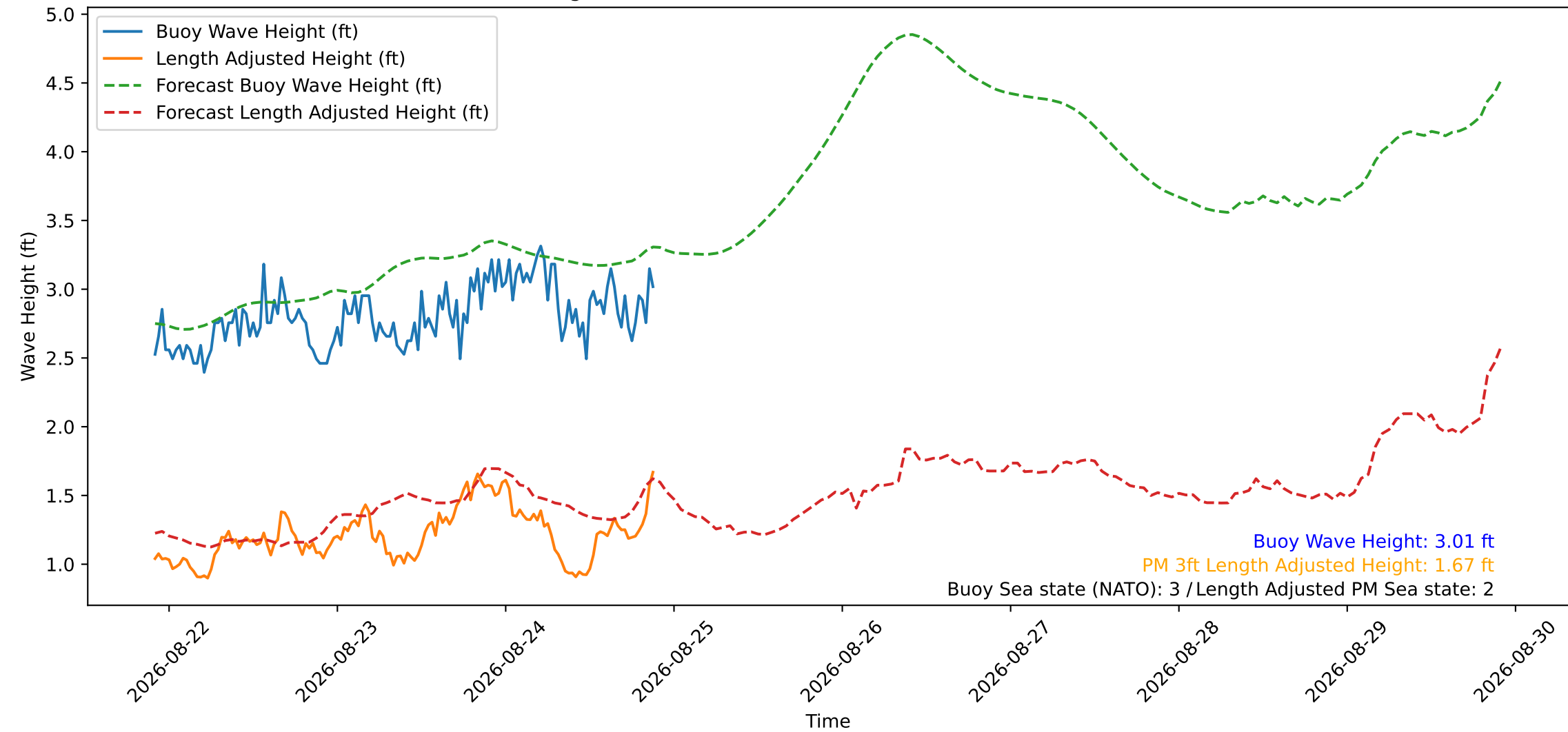
Wave Heights over Time for Green Beach at 2026-08-24 21:41:12
