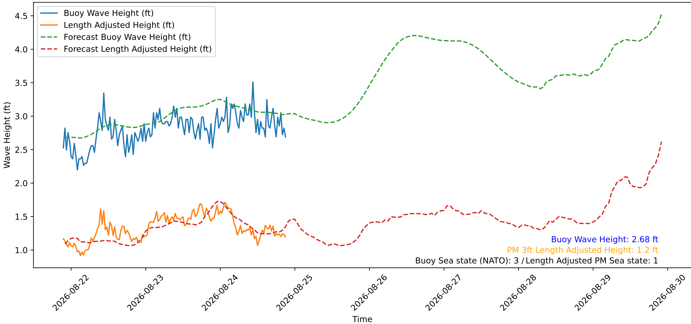
Wave Heights over Time for Oceanside Harbor at 2026-08-24 21:40:29
