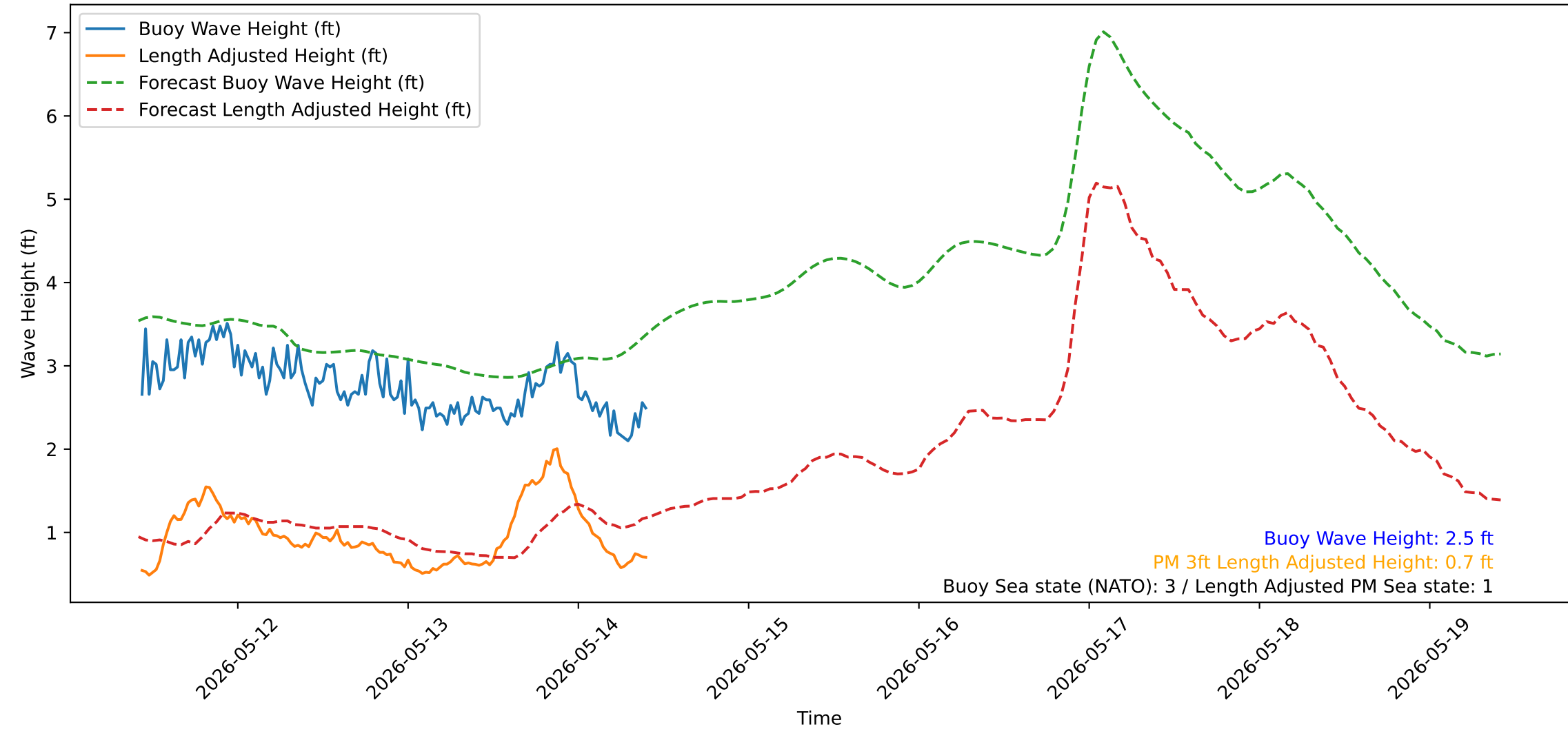
Wave Heights over Time for Green Beach at 2026-05-14 10:21:15
