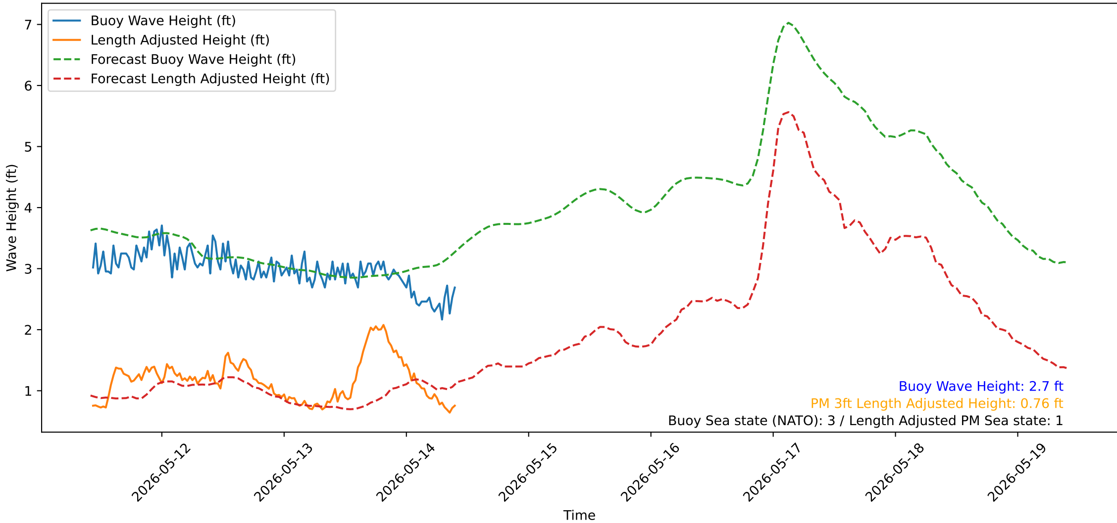
Wave Heights over Time for Oceanside Harbor at 2026-05-14 10:20:31
