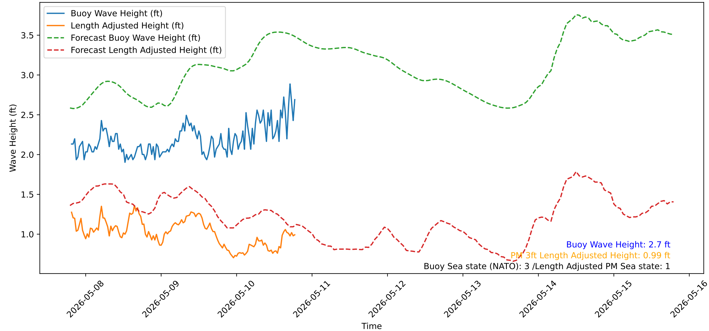
Wave Heights over Time for Red Beach at 2026-05-10 19:10:50
