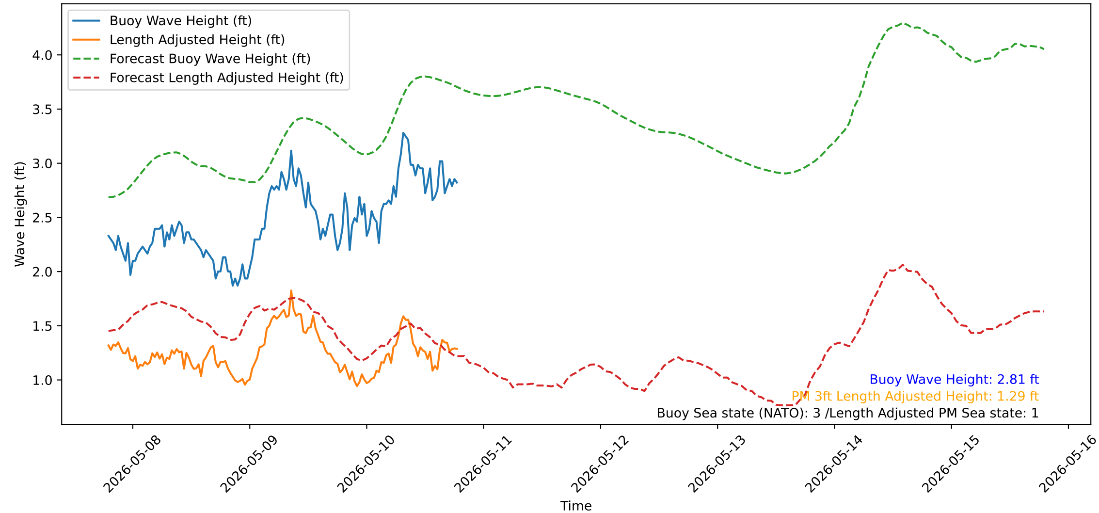
Wave Heights over Time for Oceanside Harbor at 2026-05-10 19:10:31
