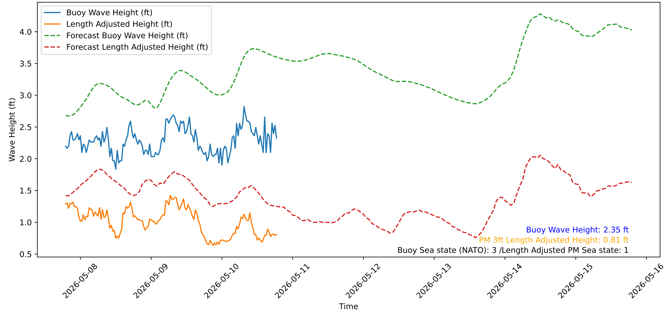
Wave Heights over Time for Green Beach at 2026-05-10 19:11:12
