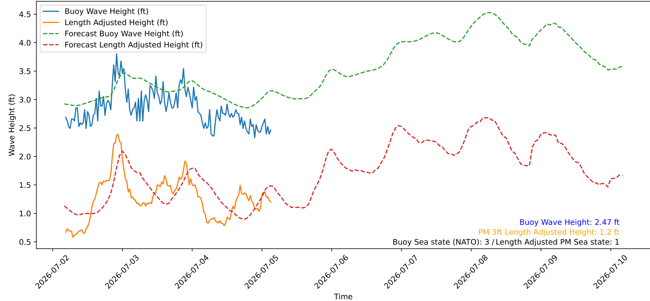
Wave Heights over Time for Red Beach at 2026-07-05 04:00:46
