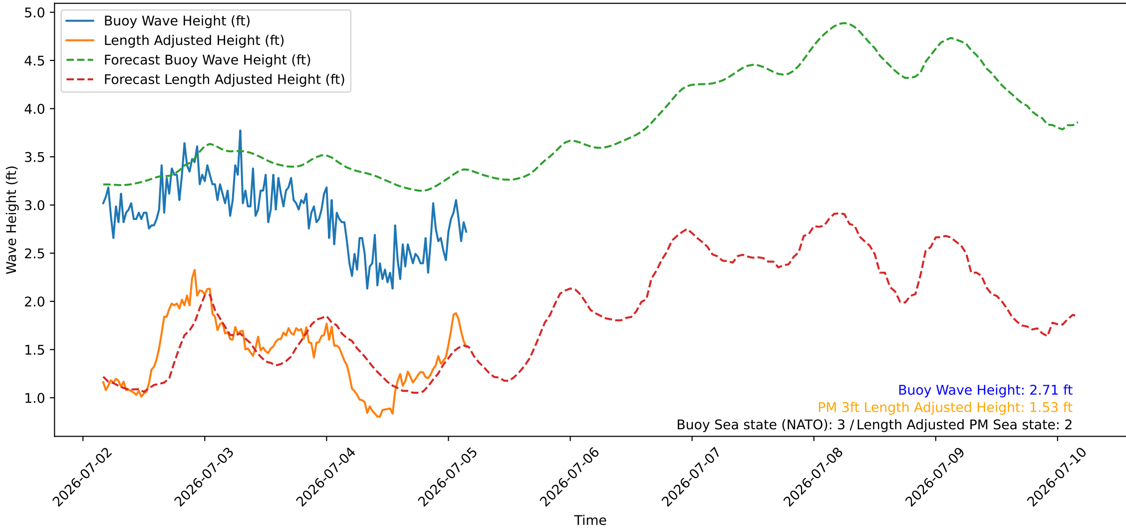
Wave Heights over Time for Oceanside Harbor at 2026-07-05 04:00:26
