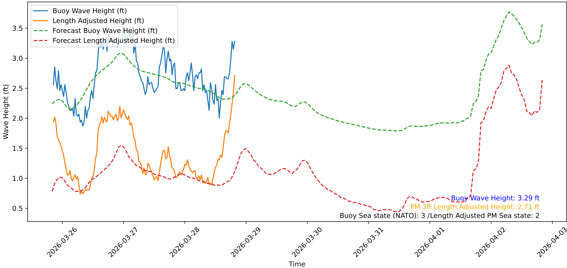
Wave Heights over Time for Green Beach at 2026-03-28 20:21:09
