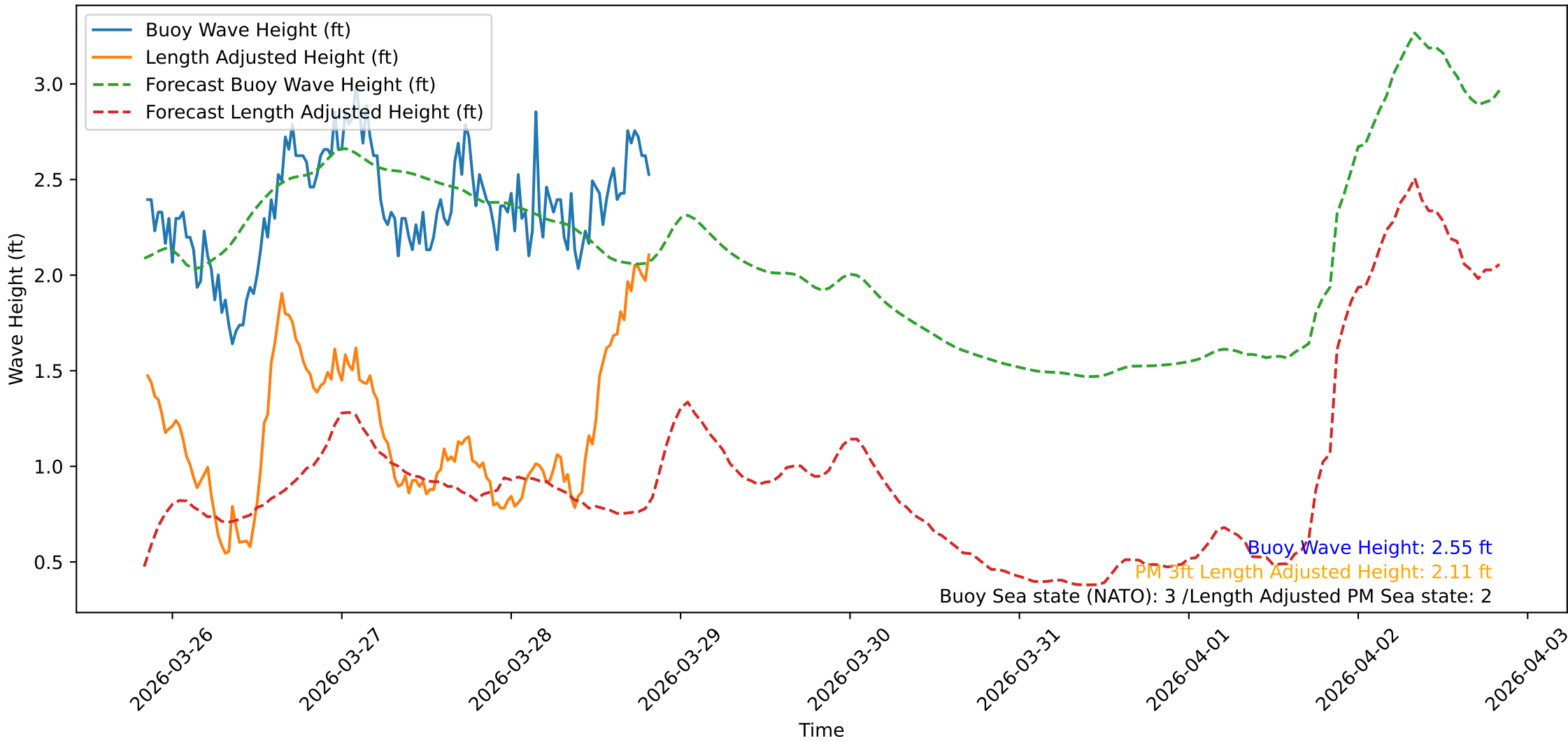
Wave Heights over Time for Red Beach at 2026-03-28 20:20:47
