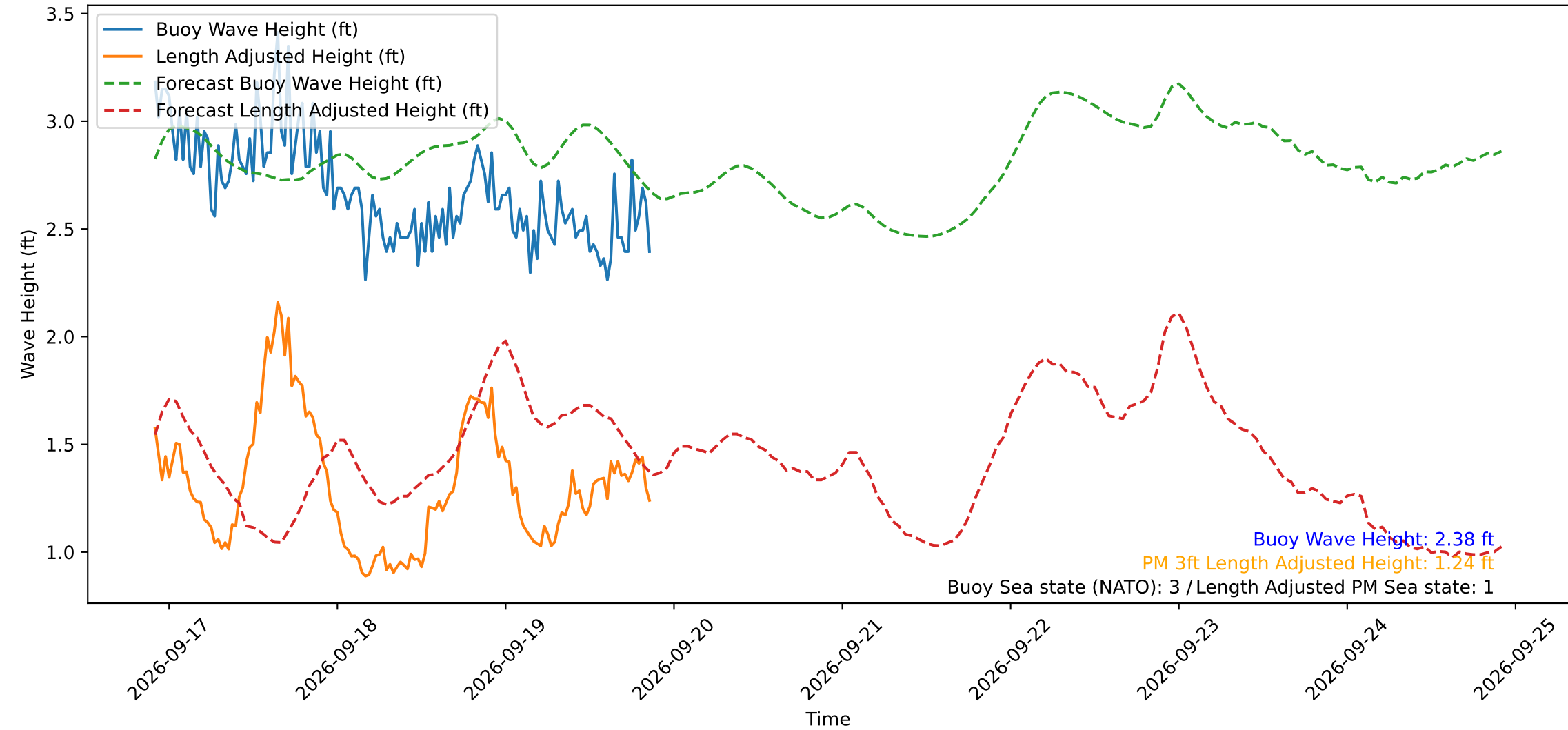
Wave Heights over Time for Red Beach at 2026-09-19 21:40:49
