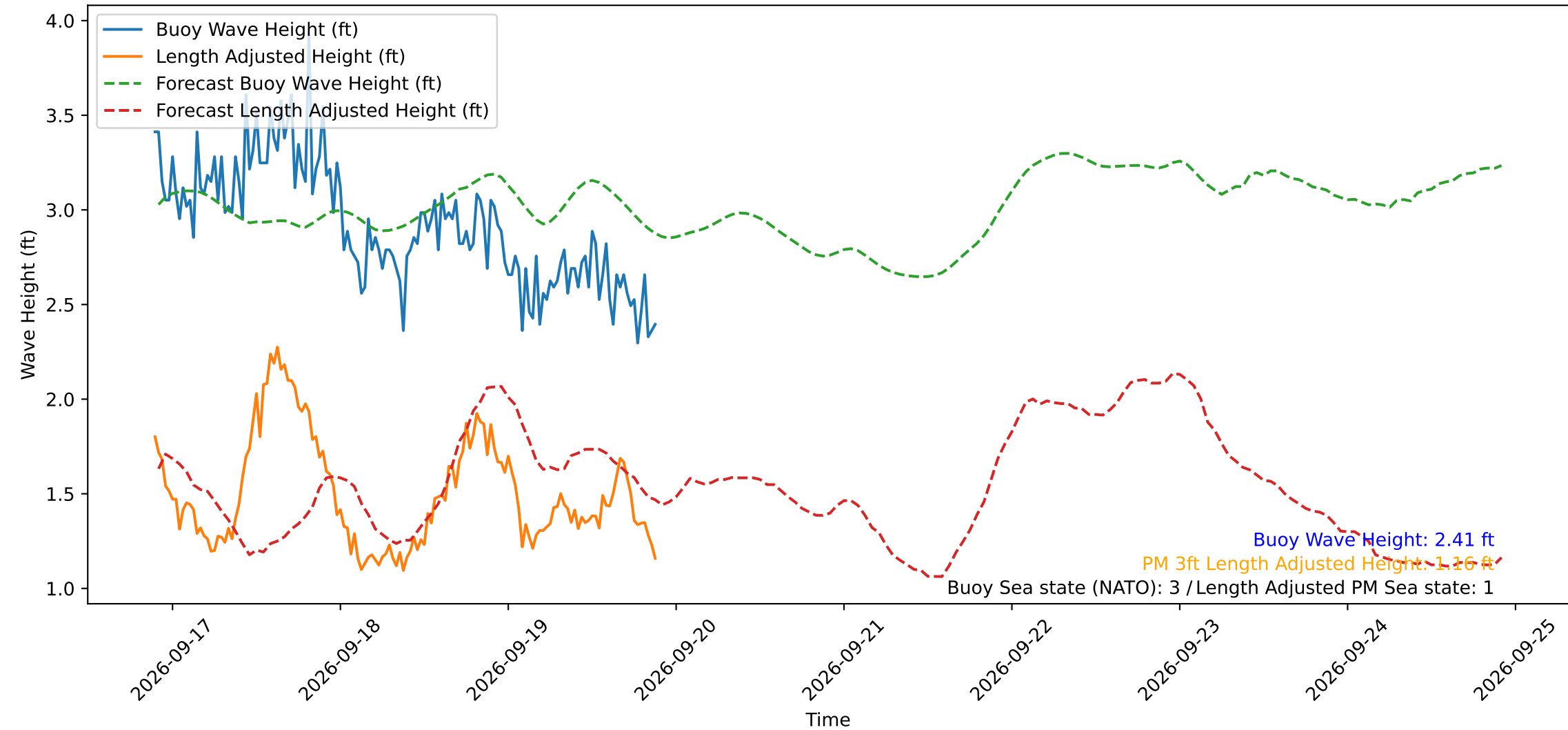
Wave Heights over Time for Oceanside Harbor at 2026-09-19 21:40:29
