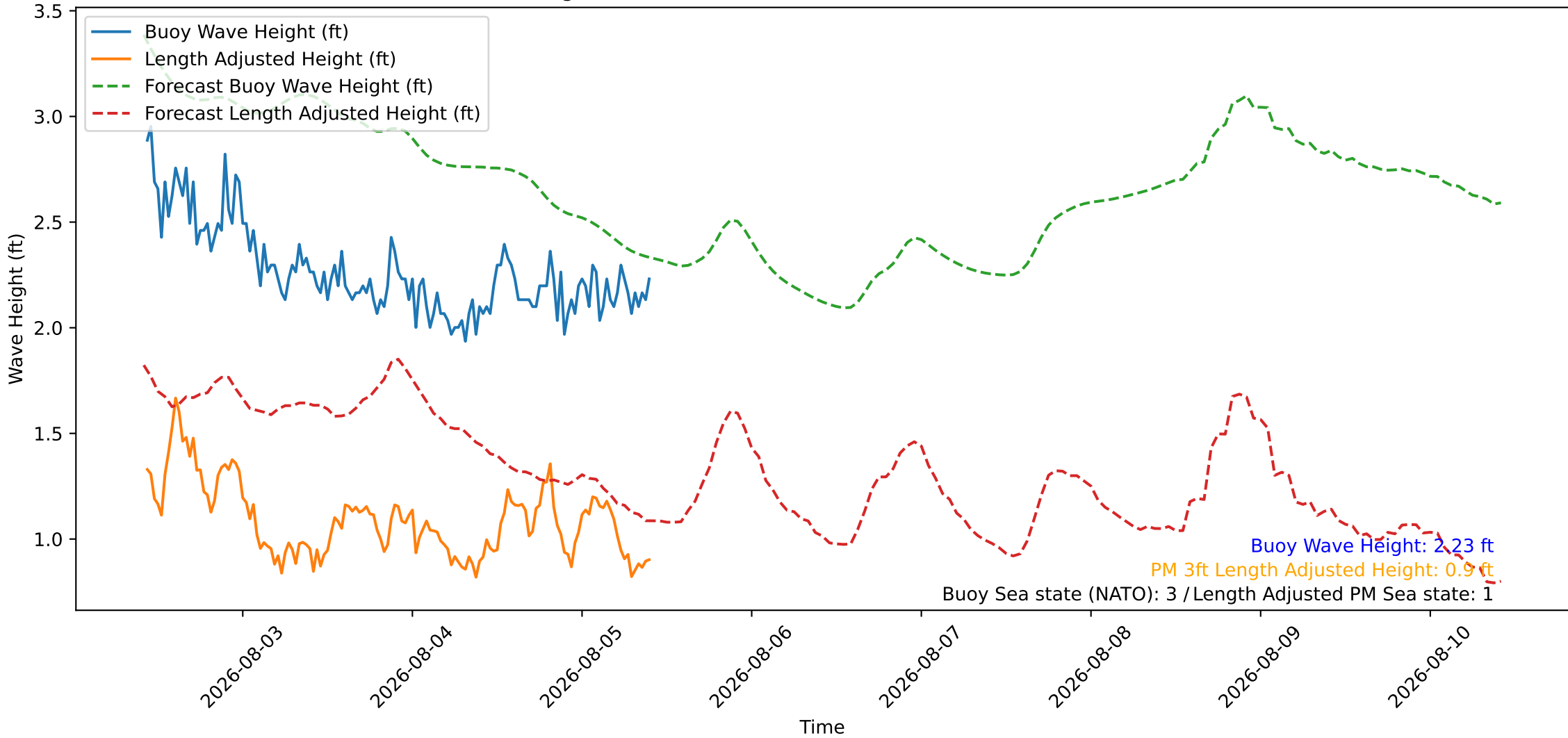
Wave Heights over Time for Green Beach at 2026-08-05 10:21:09
