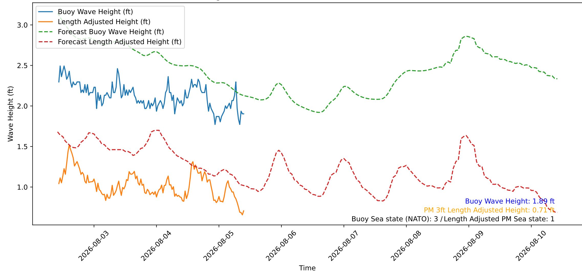
Wave Heights over Time for Red Beach at 2026-08-05 10:20:47
