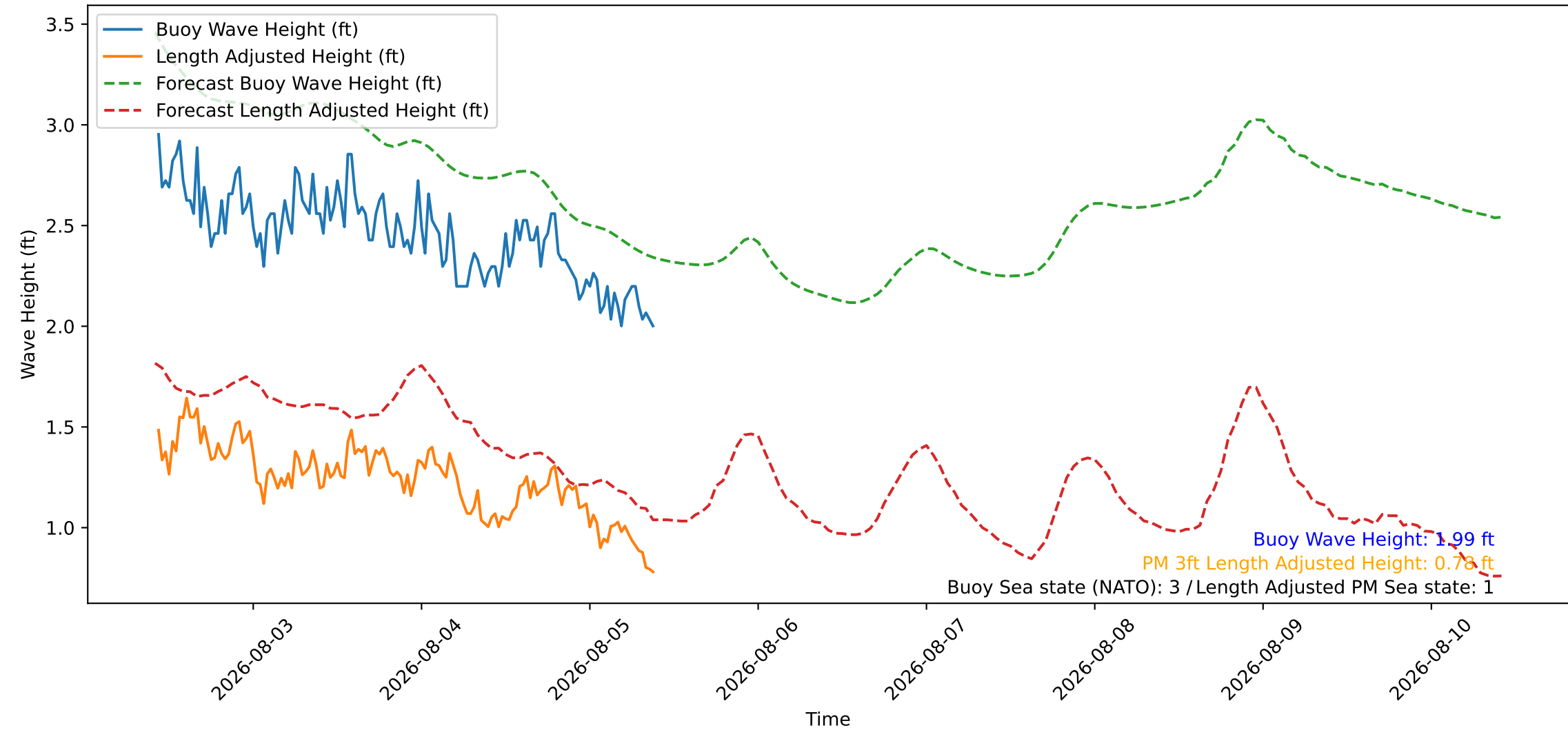
Wave Heights over Time for Oceanside Harbor at 2026-08-05 10:20:26
