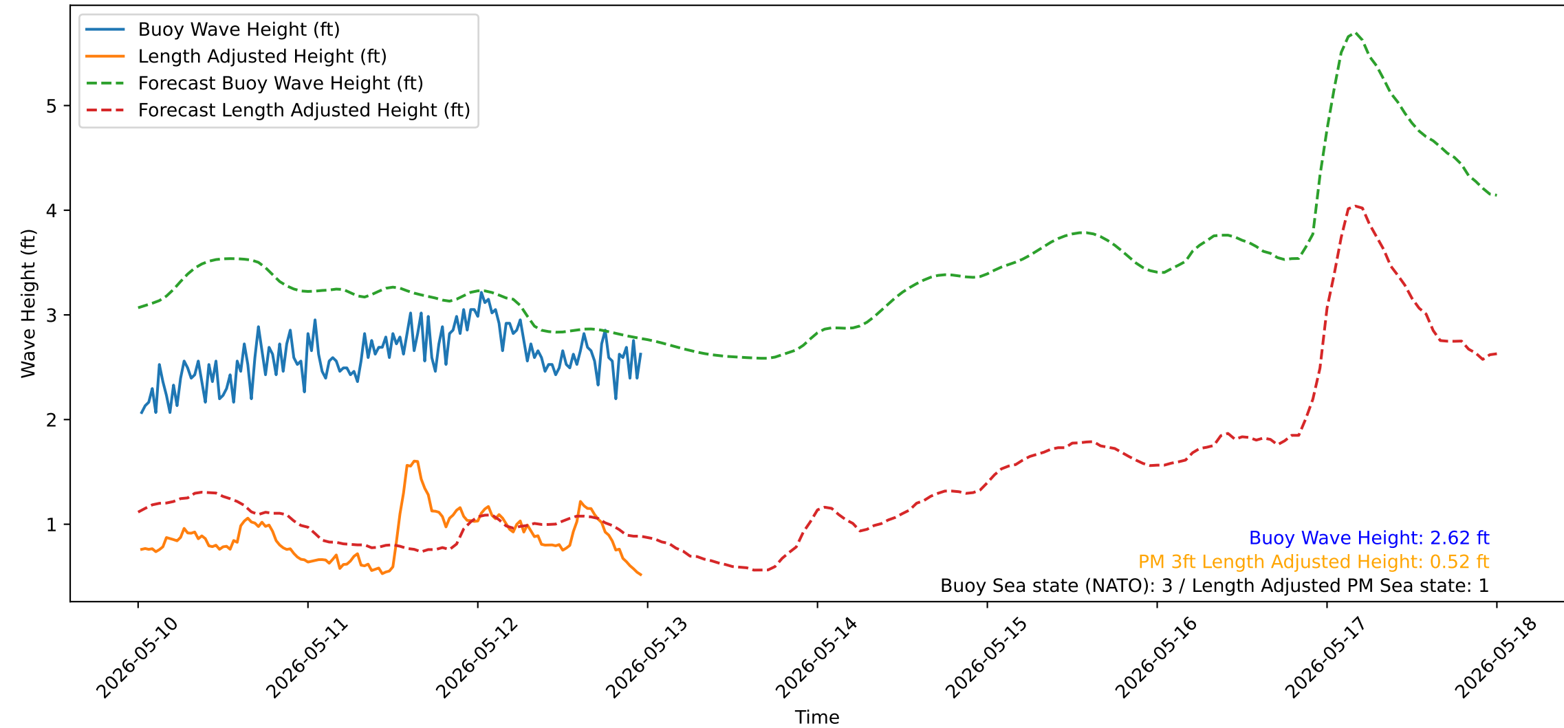
Wave Heights over Time for Red Beach at 2026-05-13 00:00:50
