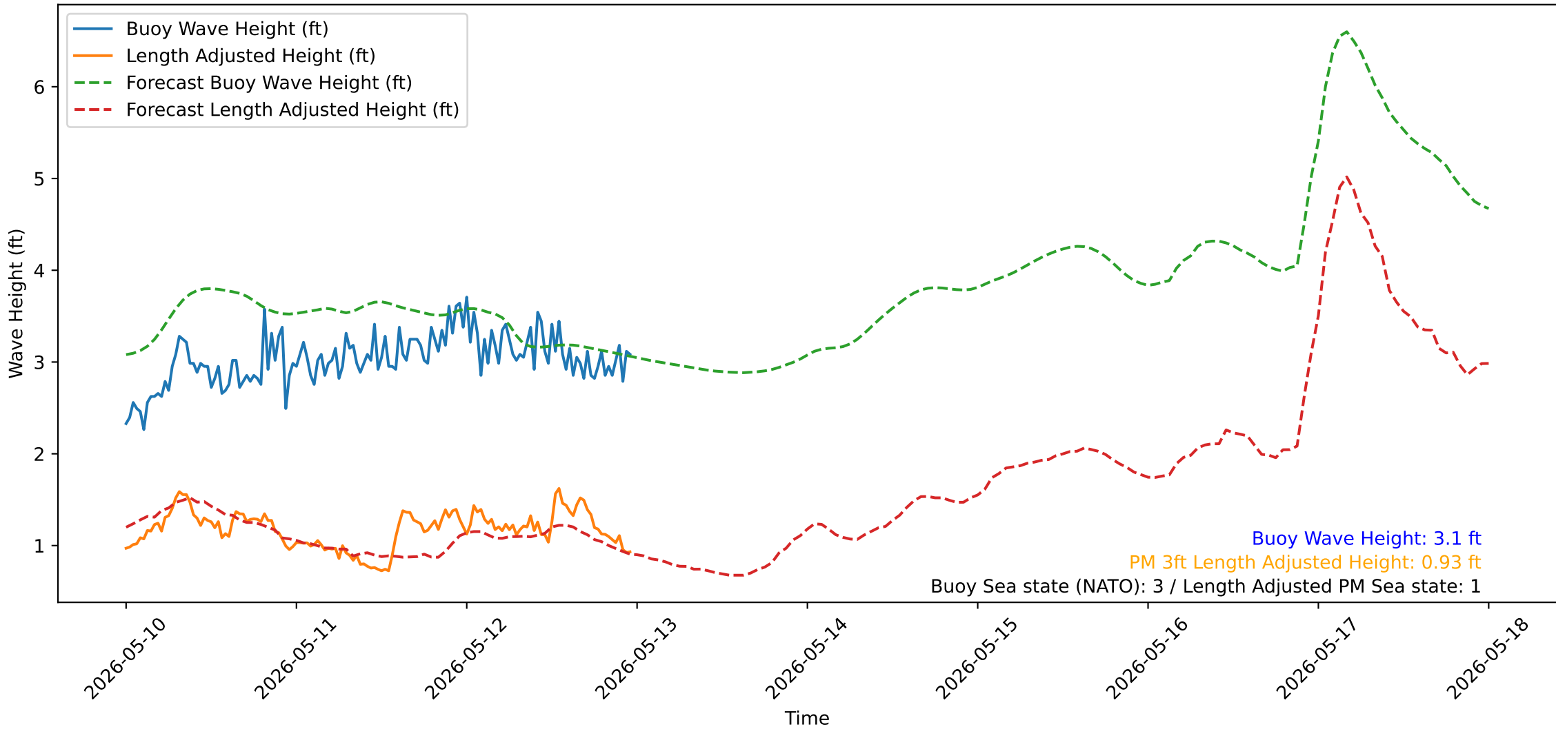
Wave Heights over Time for Oceanside Harbor at 2026-05-13 00:00:31
