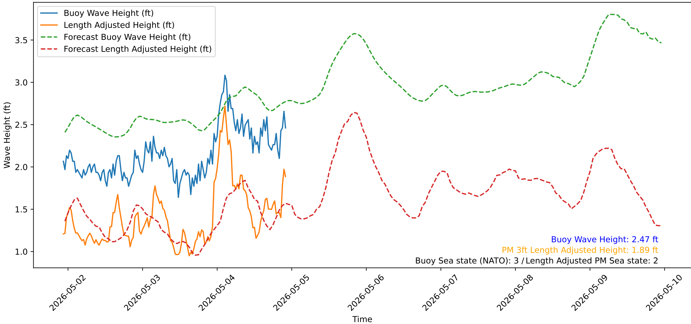
Wave Heights over Time for Oceanside Harbor at 2026-05-04 22:40:32
