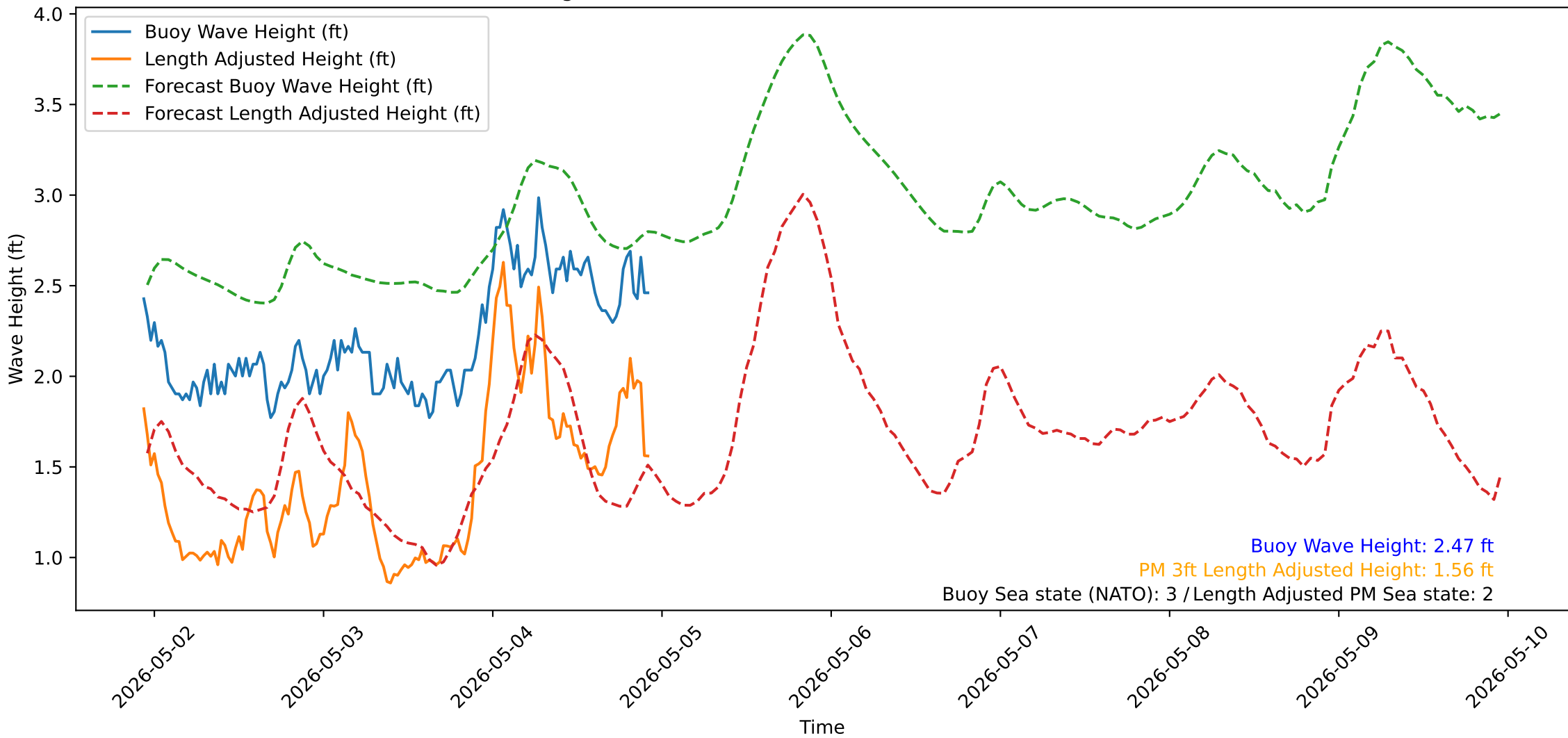
Wave Heights over Time for Green Beach at 2026-05-04 22:41:14
