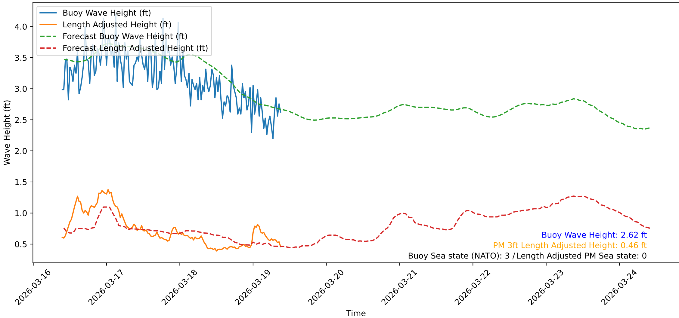
Wave Heights over Time for Green Beach at 2026-03-19 09:41:09
