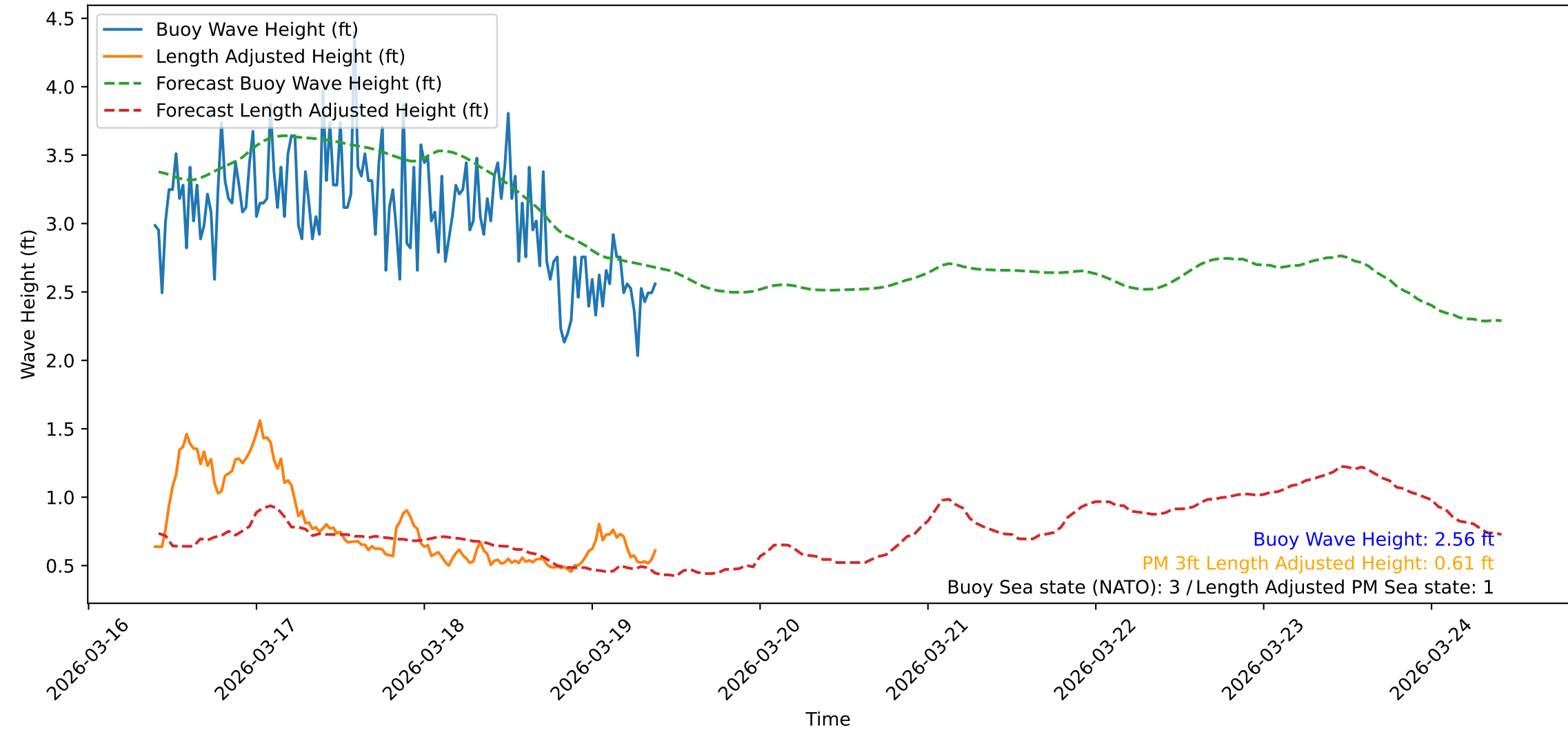
Wave Heights over Time for Oceanside Harbor at 2026-03-19 09:40:31
