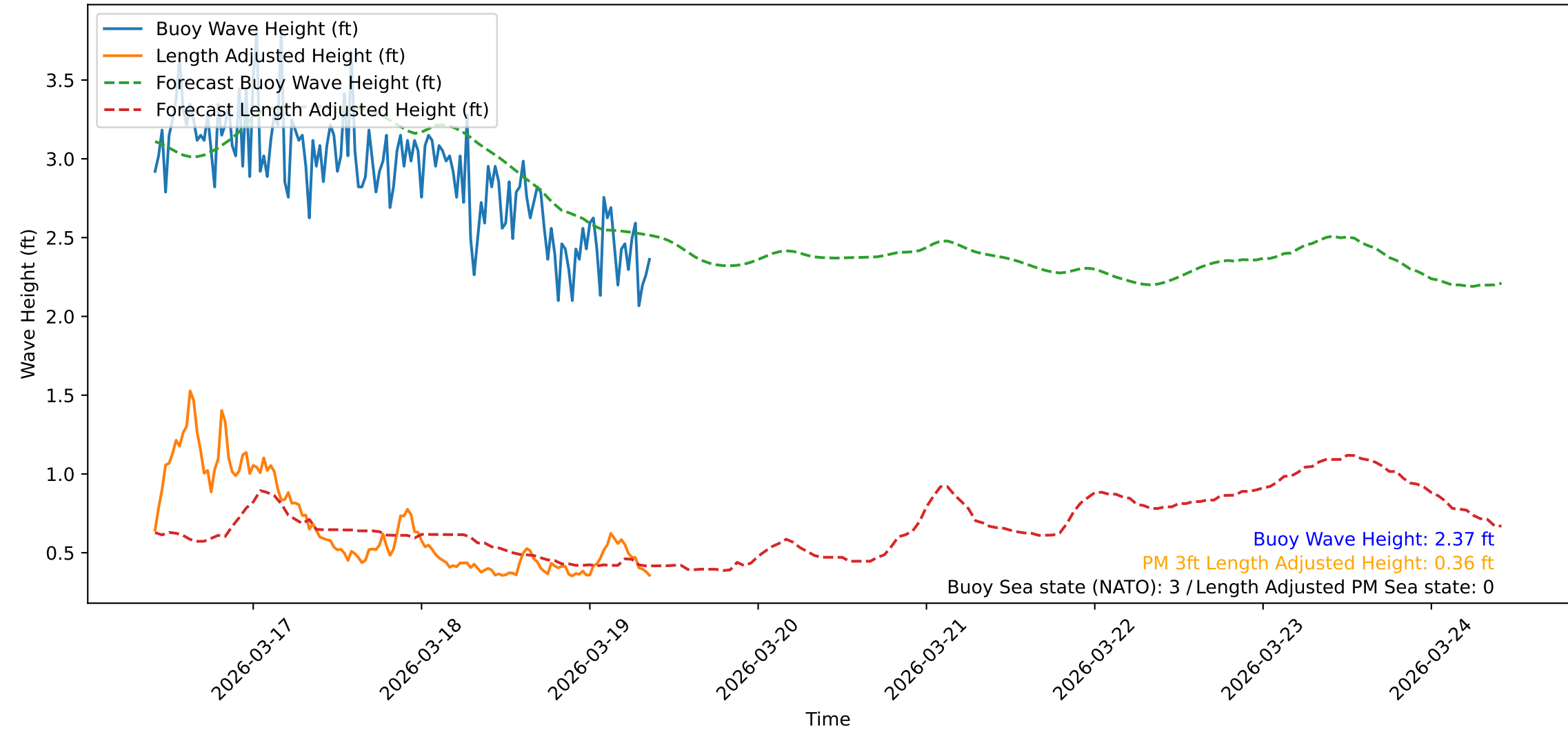
Wave Heights over Time for Red Beach at 2026-03-19 09:40:47
